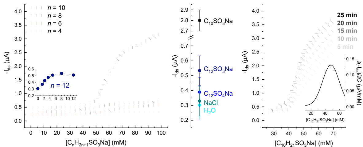
Figure 3 – Output data collected at fixed V_{ds} = -0.8 V and V_g = -1.0 V for P3HT-based OEET working with C_nH_{2n+1}SO_3Na with n = 4, 6, 8, 10 and 12 at different electrolyte concentrations ranging between 1 – 100 mM at 25 °C (left panel), working with C_{12}H_{25}SO_3Na and C_{12}H_{25}SO_4Na just above their c.m.c. ( i.e. \sim 8 - 10 mM), NaCl at 10 mM and distilled water at 25 °C (middle panel) and working with n = 10 at different stabilization times and the corresponding first derivative for stabilized data at 25 °C (right panel).
