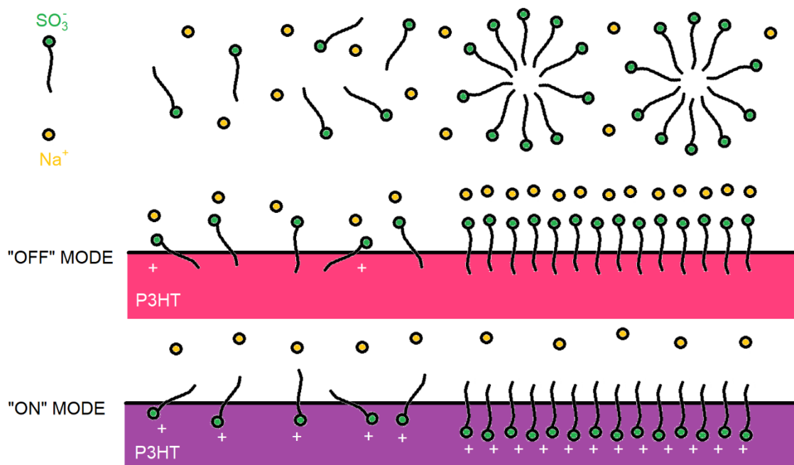
Figure 7 – Schematization of the formation of a monolayer in the electrolyte/P3HT interface above the critical micelle concentration and its effect on the “OFF” and “ON” states for P3HT-based OECT.
