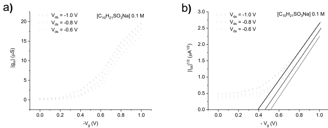
Figure 5 – a) Transconductance ( g_m vs V_g at selected V_{ds} values) and b) threshold voltage ( |I_{ds}|^{1/2} vs V_g at selected V_{ds} values) plots for P3HT-based OECT working with [C_{10}H_{21}SO_3Na] 0.1 M electrolyte at 25 °C.
