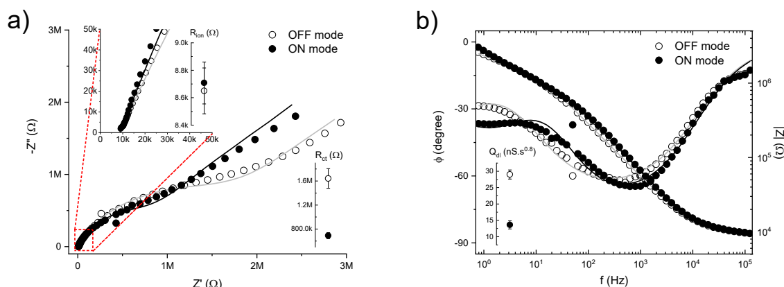
Figure 6 – a) Nyquist and b) Bode plots for P3HT-based OECT working with [C_{10}H_{21}SO_3Na] 0.1 M electrolyte at 25 °C for different operation modes; i.e. OFF ( V_{g,dc} = 0.0 V) and ON ( V_{g,dc} = -1.0 V).
