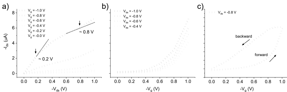
Figure 4 – a) Output ( -I_{ds} vs -V_{ds} at selected V_g values), b) transfer ( -I_{ds} vs -V_g at selected V_{ds} values) and c) hysteresis transfer ( -I_{ds} vs -V_g at selected V_{ds} value in forward and backward directions) characteristics for P3HT-based OECT working with [C_{10}H_{21}SO_3Na] 0.1 M electrolyte at 25 °C. The voltages at which the transistor output characteristic switches from linear to quasi-saturation regime are marked with arrows.
