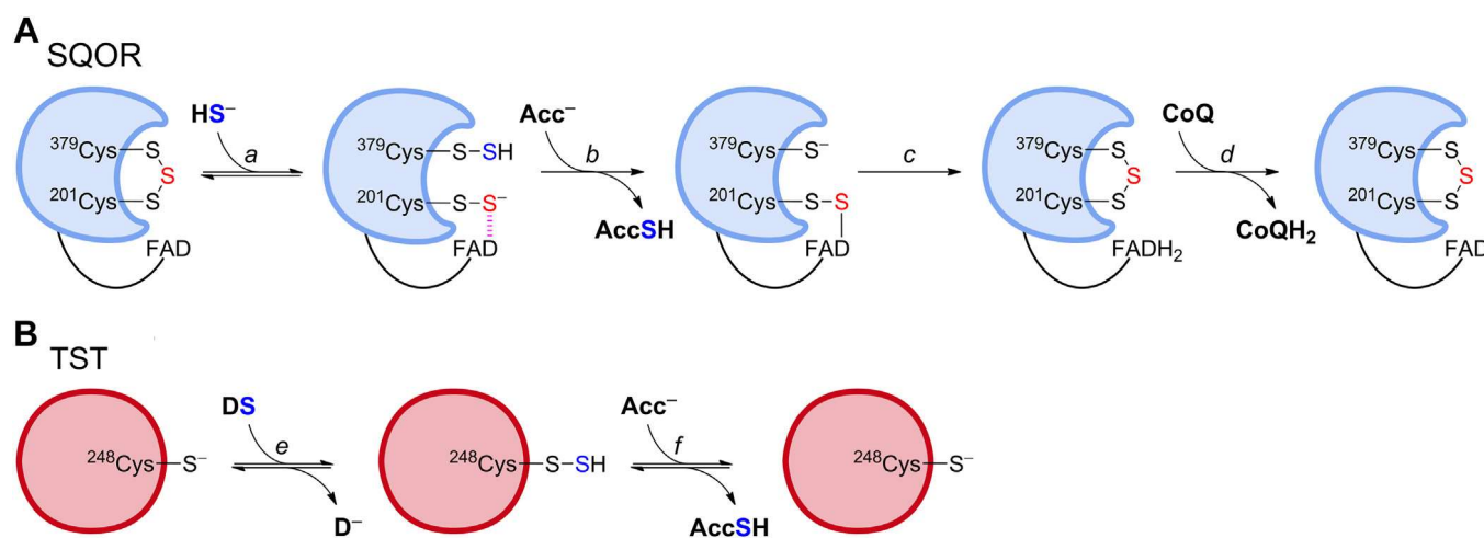
Figure 1. Proposed catalytic mechanisms for human SQOR and TST. A, the active site cysteine trisulfide in SQOR is attacked by \text{H}_2\text{S} to form two persulfides, at \text{Cys}_{379} and at \text{Cys}_{201} ; the latter engages in a transient charge transfer (CT) complex with the FAD cofactor (reaction a). Then, a thiophilic acceptor ( \text{Acc}^- ) attacks \text{Cys}_{379}\text{SSH} and the sulfane sulfur is transferred, generating \text{AccSH} and \text{Cys}_{379}\text{SH} while the CT complex is proposed to evolve to a transient C4a adduct (reaction b). Then, \text{Cys}_{379}\text{SH} attacks the adduct, regenerating the trisulfide and producing \text{FADH}_2 (reaction c). Finally, \text{FADH}_2 reduces \text{CoQ} to \text{CoQH}_2 , restoring SQOR to its resting state (reaction d) (21). B, the active site \text{Cys}_{248}\text{SH} in TST attacks a sulfane sulfur donor (DS), resulting in the formation of \text{Cys}_{248}\text{SSH} and release of the first product ( \text{D}^- ) (reaction e). Next, a thiophilic acceptor ( \text{Acc}^- ) attacks \text{Cys}_{248}\text{SSH} , producing \text{AccSH} and restoring the resting enzyme (reaction f). SQOR, sulfide quinone oxidoreductase; TST, thiosulfate sulfurtransferase.
