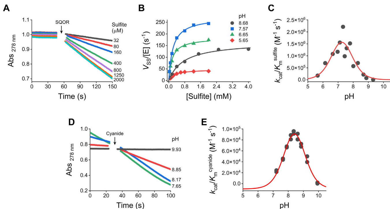
Figure 3. pH-dependence of SQOR activity. The steady-state rate of reduction of \text{CoQ}_1 was followed by the decrease in absorbance at 278 nm. The assays included 69 \mu\text{M} \text{CoQ}_1 , 0.03% DHPC, 0.06 mg/ml BSA, 150 \mu\text{M} \text{H}_2\text{S} , and variable concentrations of sulfite or cyanide in MES/Tris/ethanolamine buffer (pH 5.65–9.93, 25 °C). A, the reactions with sulfite (0.01–8 mM) were started by the addition of 1 nM SQOR. Representative absorbance kinetic traces of \text{CoQ}_1 reduction at pH 7.57. The steady-state rates were calculated from the linear fits to the data obtained 15 to 30 s after SQOR was added (subtracting the slopes before addition of SQOR). B, SQOR activity versus sulfite concentration at different pH values. Representative experiments at pH 8.68 (black circles), 7.57 (blue squares), 6.65 (green triangles), and 5.65 (red diamonds). Michaelis-Menten hyperbolas were fitted and yielded the kinetic parameters K_m^{\text{sulfite}} (Fig. S1A), k_{\text{cat}}^{\text{sulfite}} (Fig. S1B), and k_{\text{cat}}/K_m^{\text{sulfite}} for each pH. C, pH-dependence of k_{\text{cat}}/K_m^{\text{sulfite}} . Equation 3 was fitted to the data obtaining two \text{pK}_a s, 6.8 \pm 0.5 for the deprotonated species and 7.7 \pm 0.4 for the protonated one. A pH-independent k_{\text{cat}}/K_m^{\text{sulfite}} of 2.9 \pm 0.2 \times 10^6 \text{ M}^{-1} \text{ s}^{-1} was obtained for the reaction of sulfite with the persulfidated SQOR. D, the reactions with cyanide (90 \mu\text{M} ) contained 50 nM SQOR and were initiated by the addition of cyanide. Representative time courses at different pHs. To calculate the steady-state rates, the slopes in the absence of cyanide were subtracted from those obtained 4 to 20 s after the addition of cyanide. The k_{\text{cat}}/K_m^{\text{cyanide}} at each pH was calculated using Equation 2. E, pH-dependence of k_{\text{cat}}/K_m^{\text{cyanide}} . Equation 3 plus an offset was fitted to the data, yielding a \text{pK}_a of 8.9 \pm 0.2 for the deprotonated species, a \text{pK}_a of 7.9 \pm 0.1 for the protonated species, an offset of (-10 \pm 5) \times 10^3 \text{ M}^{-1} \text{ s}^{-1} , and a pH-independent k_{\text{cat}}/K_m^{\text{cyanide}} of 1.5 \pm 0.8 \times 10^6 \text{ M}^{-1} \text{ s}^{-1} for the reaction of cyanide with the persulfidated SQOR. Values are parameters \pm standard errors of the fits. DHPC, 1,2-diheptanoyl-sn-glycero-3-phosphocholine; SQOR, sulfide quinone oxidoreductase.
