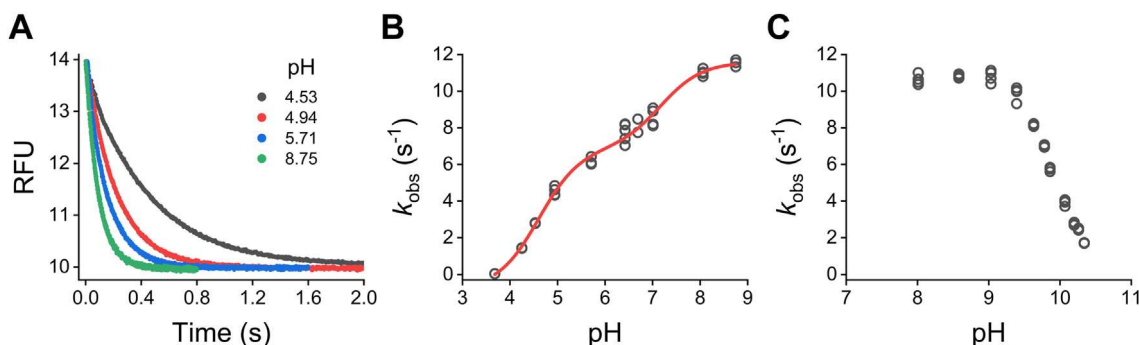
Figure 7. Stopped-flow kinetics of TST thiol with thiosulfate. A, representative fluorescence time courses ( \lambda_{ex} = 295 \text{ nm} , US 360 nm bandpass filter) of TST thiol (0.9 \mu\text{M} ) exposed to 200 \mu\text{M} thiosulfate in acetic/MES/Tris buffer (pH 3.68–8.75, 25 °C). Single or double exponential functions were fitted to the data. B, pH-dependence of k_{obs} for a representative experiment. For the double exponential fits, the smaller k_{obs} values, which corresponded to the larger amplitude, were used. Using data from three independent experiments, a two- pK_a sigmoidal function was fitted yielding pK_a values of 4.6 \pm 0.1 and 6.5 \pm 0.1 and maximal k_{obs} of 5.9 \pm 0.6 and 11.5 \pm 0.3 \text{ s}^{-1} , respectively (parameters \pm standard errors of the fit). C, pH-dependence of the k_{obs} at alkaline pH values. The reactions were performed as described but in ACES/Tris/ethanolamine buffer (pH 6.68–10.34, 25 °C), and a single exponential plus straight line function was fitted to the data to obtain the k_{obs} . Representative of two independent experiments, five replicates each. TST, thiosulfate sulfurtransferase.
