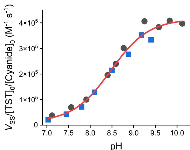
Figure 4. pH-dependence of TST activity. The steady-state activity of TST (5–100 nM) was measured by the formation of thiocyanate in the presence of thiosulfate (300 mM) and cyanide (300 \mu M, lower than K_m^{\text{cyanide}} ) in ACES/Tris/ethanolamine buffer in the pH range of 7.03 to 10.12 and 25 °C. A sigmoidal function was fitted to the data of two independent experiments (black circles and blue squares) and yielded an apparent pK_a of 8.47 \pm 0.06 and a maximum apparent rate constant of (4.0 \pm 0.1) \times 10^5 \text{ M}^{-1} \text{ s}^{-1} (parameters \pm standard errors of the fit). TST, thiosulfate sulfurtransferase.
