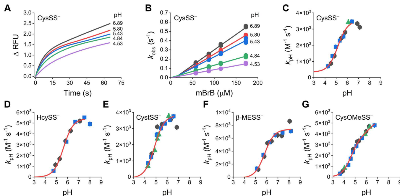
Figure 2. pK_a of LMW persulfides and their reactivity with mBrB. A, representative stopped-flow fluorescence kinetic traces ( \lambda_{ex} = 396 nm, emission cut-off 435 nm) of the reaction of CysSSH-containing mixtures (0.5–3 \mu M) with mBrB (57.5 \mu M) in acetic/MES/Tris buffer (pH 3.65–8.15, 25 °C). Exponential plus straight line functions were fitted to the time courses over 10 half-lives. In some cases, where double exponential plus straight line functions were fitted, the exponential phase with the lower observed rate constant ( k_{obs} ) and larger amplitude was attributed to the reaction of the persulfide with mBrB. B, linear dependence of k_{obs} of CysSSH with mBrB concentration. Circles are quintuplates of k_{obs} obtained for every pH and mBrB concentration. The slope at each pH represents the apparent second-order rate constants, k_{pH} . At the more alkaline pH values, a small negative y-intercept was observed, as seen previously with GSSH (13). C, for CysSSH, a single- pK_a function was fitted to the plot of k_{pH} versus pH with data obtained in three independent experiments (black circles, blue squares, and green triangles). A pK_a of 5.2 \pm 0.1 and a pH-independent second-order rate constant, k_{ind} , of (3.2 \pm 0.1) \times 10^3 \text{ M}^{-1} \text{ s}^{-1} (parameters \pm standard errors of the fit) were determined. As seen previously with GSSH (13), a small decrease of unknown origin in the k_{pH} at the more alkaline pH values was observed. D–G, the pK_a and k_{ind} of the reactions with mBrB for other LMW persulfides were determined analogously. Plots of k_{pH} versus pH for HcySSH (D), CystSSH (E), \beta -MESSH (F), and CysOMeSSH (G). In the case of CysOMeSSH, a two- pK_a function was fitted resulting in two sets of pK_a and k_{ind} values. The obtained values are summarized in Table 1. CysOMeSSH, cysteine methyl ester persulfide anion; CysSSH, cysteine persulfide; CystSSH, cysteamine persulfide anion; HcySSH, homocysteine persulfide anion; LMW, low molecular weight; mBrB, monobromobimane; \beta -MESSH, \beta -mercaptoethanol persulfide anion.
