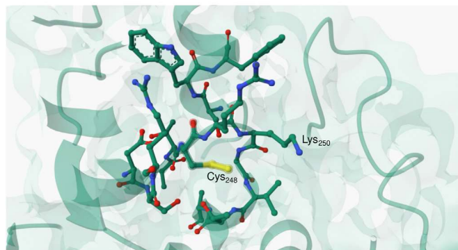
Figure 9. Persulfides in SQOR and TST. A, close-up of the bis-persulfide in the SQOR structure (PDB 6OIB). Residues within 5 Å from Cys 379 SSH, the FAD cofactor, and the CoQ substrate are depicted in sticks. B, close-up of the persulfide in the bovine TST structure (PDB 1RHD). Residues within 5 Å from Cys 248 are depicted in sticks. Figures were constructed with Mol* (65). SQOR, sulfide quinone oxidoreductase; TST, thiosulfate sulfurtransferase.
