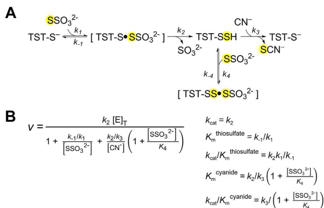
Figure 6. TST mechanism and inhibition by thiosulfate. A, TST catalytic mechanism using thiosulfate and cyanide as substrates and depicting inhibition by high concentrations of thiosulfate (30, 31). B, steady-state rate equation assuming fast equilibrium for thiosulfate binding and steady-state for the persulfidated enzyme. TST, thiosulfate sulfurtransferase.
