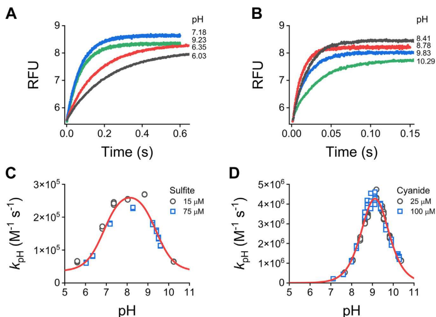
Figure 5. Stopped-flow kinetics of TST persulfide with sulfur acceptors. A and B, representative fluorescence time courses ( \lambda_{\text{ex}} = 295 \text{ nm} , US 360 nm bandpass filter) of TST persulfide (0.8–1.0 \mu M) exposed to 75 \mu M sulfite (A) or 25 \mu M cyanide (B), in ACES/Tris/ethanolamine buffer (pH 5.60–10.38, 25 °C). Single exponential functions were fitted and the k_{\text{obs}} was divided by the concentration of sulfite or cyanide to give the corresponding k_{\text{pH}} . C and D, pH-dependence of k_{\text{pH}} . Bell-shaped functions (Equation 3 or Equation 3 plus an offset) were fitted to the data, yielding pK_a values of 6.89 \pm 0.09 (deprotonated species) and 9.38 \pm 0.07 (protonated species), an offset of (3.5 \pm 0.9) \times 10^4 \text{ M}^{-1} \text{ s}^{-1} , and a k_{\text{ind}} of (2.5 \pm 0.1) \times 10^5 \text{ M}^{-1} \text{ s}^{-1} for the reaction with sulfite (C) and pK_a values of 8.87 \pm 0.06 (deprotonated species) and 9.37 \pm 0.05 (protonated species) and a k_{\text{ind}} of (1.0 \pm 0.1) \times 10^7 \text{ M}^{-1} \text{ s}^{-1} for the reaction with cyanide (parameters \pm standard errors of the fits). TST, thiosulfate sulfurtransferase.
