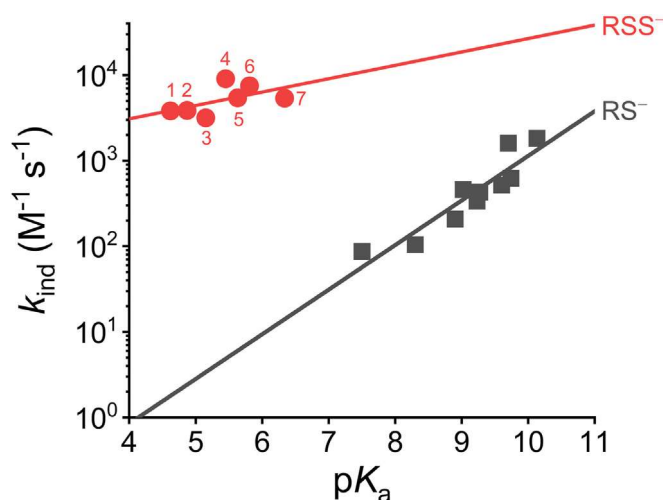
Figure 8. Comparison of the reactivity of LMW persulfide anions and thiolates with mBrB. Brønsted plot exhibiting pH-independent rate constants (in logarithmic scale) versus pK_a for the reactions of persulfide anions or thiolates with mBrB ( I = 0.15 and 25^\circ \text{C} ). Red circles: CysOMeSS ^-(\text{NH}_3^+) (1), CystSS ^- (2), CysSS ^- (3), GSS ^- (4), HcySS ^- (5), \beta -MESS ^- (6), and CysOMeSS ^-(\text{NH}_2) (7); \beta_{\text{nuc}} = 0.2 \pm 0.1 ( R^2 = 0.31 ). The values are depicted in Table 1. Black squares: reported data for LMW thiolates; \beta_{\text{nuc}} = 0.52 \pm 0.08 ( R^2 = 0.85 ) (16). LMW, low molecular weight; mBrB, monobromobimane.
