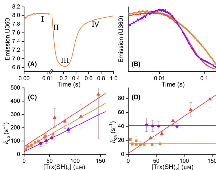
Fig. 3. Reduction of Prx1 by Trx. (A) Complete time course of the reaction of 1.25 \mu\text{M} \text{Prx1S}_2 plus 5 \mu\text{M} \text{H}_2\text{O}_2 with 68 \mu\text{M} \text{HsTrx1} consisting of: I upward exponential used to obtain k_{\text{up}} ; II downward exponential used to obtain k_{\text{dn}} ; III transient of the system cycling until the excess \text{H}_2\text{O}_2 is consumed; IV upward exponential with a k_{\text{obs}} = 12.7 \text{ s}^{-1} , consistent with the resolution (Reaction 2 in Fig. 1) the line is the average of 15 runs. (B) Time courses of reduction of 1.25 \mu\text{M} \text{Prx1S}_2 plus 5 \mu\text{M} \text{H}_2\text{O}_2 with 45.6 \mu\text{M} \text{HsTrx1} (orange, average of 15 runs), 3.75 \mu\text{M} \text{Prx1S}_2 plus 7.5 \mu\text{M} \text{H}_2\text{O}_2 with 54 \mu\text{M} \text{HsTrx2} (magenta, average of 9 runs), or 5 \mu\text{M} \text{Prx1S}_2 plus 10 \mu\text{M} \text{H}_2\text{O}_2 with 40 \mu\text{M} \text{EcTrx} (red, average of 13 runs), respectively. (C) Second-order plot of the ascending exponential rate constant ( k_{\text{up}} ) vs [\text{HsTrx1}] (orange \blacksquare ), [\text{HsTrx2}] (magenta \bullet ) or [\text{EcTrx}] (red \blacktriangle ), slopes of the linear regressions, 2.2 \pm 0.5 \times 10^6 , 1.9 \pm 0.02 \times 10^6 , 2.8 \pm 0.7 \times 10^6 \text{ M}^{-1} \text{ s}^{-1} , respectively. (D) Second-order plot of the descending exponential rate constant ( k_{\text{dn}} ) vs [\text{HsTrx1}] (orange \blacksquare ), [\text{HsTrx2}] (magenta \bullet ) or [\text{EcTrx}] (red \blacktriangle ), slopes of the linear regressions, 0, 0 and 5.3 \pm 0.6 \times 10^5 \text{ M}^{-1} \text{ s}^{-1} , respectively, the points are mean \pm SD of 15, 9, and 13 repetitions, respectively. The two horizontal lines were forced in the regression, see “Reaction order and interpretation of kinetic data” in the Results and Discussion section.
