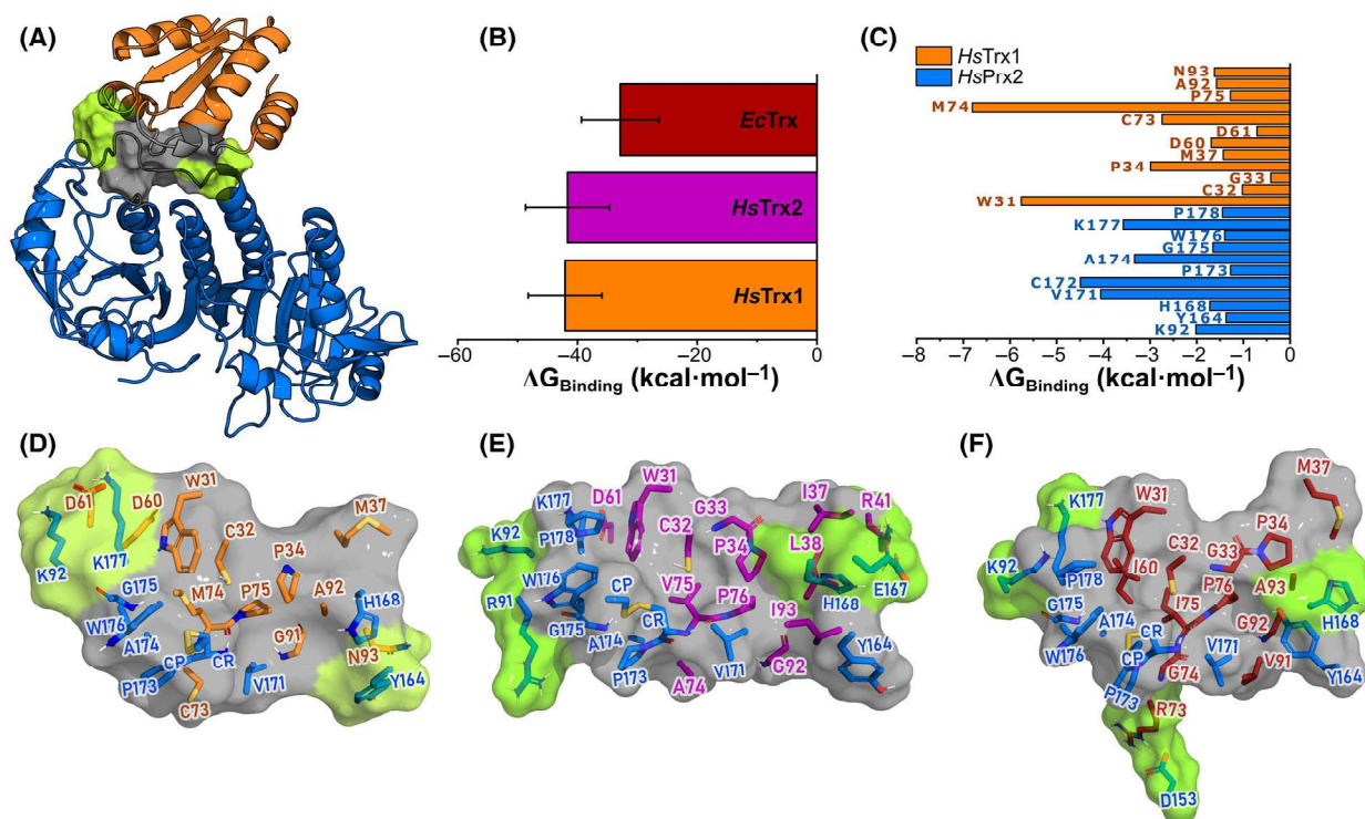
Fig. 5. Features of Prx2-Trx interaction. (A) Cartoon representation of the predicted complex between Prx2S 2 (blue) and HsTrx1 (orange). The interaction area is shown as a surface, where regions 1 (gray) and 2 (green) are depicted. Structures generated with PyMOL Molecular Graphics System, Version 2.5.5 Schrödinger, LLC. (B) MM-GBSA \Delta G_{\text{Binding}} estimation (kcal·mol -1 ) for each complex. (C) Decomposition of the \Delta G_{\text{Binding}} in a per residue basis for HsTrx1, bars represent the average \Delta G_{\text{Binding}} (B) and per residue decomposed \Delta G_{\text{Binding}} (C) calculated for 1000 frames ( n = 1000 ) of 500 ns MD simulations (one per complex). In B the error bars represent the SD of the normal distribution of the data. Most relevant residues at the interaction surface are shown for HsTrx1 (orange) (D), HsTrx2 (magenta) (E) and EcTrx (red) (F). Regions 1 and 2 are represented as surfaces and the residues are depicted as blue (Prx2(S) 2 ), orange (HsTrx1), magenta (HsTrx2) and red (EcTrx) sticks, structures generated with PyMOL Molecular Graphics System, Version 2.5.5 Schrödinger, LLC.
