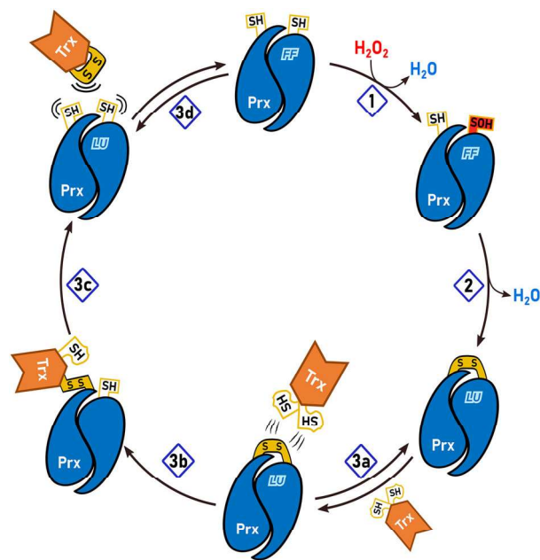
Fig. 1. Extended canonic catalytic cycle of a 2-Cys Prx. The numbers indicate the sequence of reactions: 1 Oxidation by \text{H}_2\text{O}_2 , 2 Resolution, and 3 Reduction by Trx. The Reduction step is subdivided in 3a Prx-Trx non covalent association, 3b first thiol-disulfide exchange, 3c second thiol-disulfide exchange, and 3d dissociation of the Prx-Trx non covalent complex. The “fully folded” (FF) and “locally unfolded” (LU) states are indicated. Although there are two active sites per dimer, for simplicity only one is depicted.
