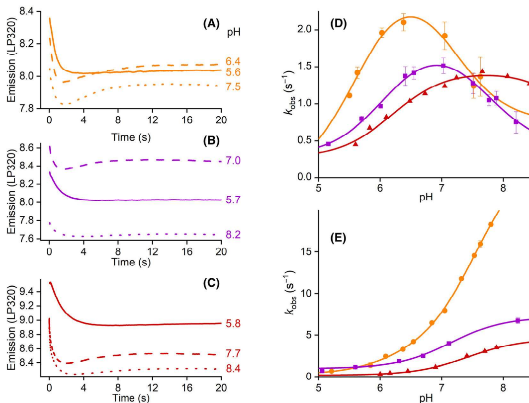
Fig. 4. Reduction of Prx2 by Trx as a function of pH and comparison with DTDPy. Panels A, B and C show reaction time courses at selected pH values for HsTrx1 (orange), HsTrx2 (magenta), and EcTrx (red), lines are averages of 12 runs. (D) The rate constant of the descent in fluorescent emission plotted vs pH has a bell-shaped profile that can be described by a two pK_a function (Eqn 6), points are average \pm SD of 12 repetitions. Best fit values of pK_a are: 5.6 and 7.2 for HsTrx1 , 6.1 and 7.7 for HsTrx2 , and 6.4 and > 8.5 for EcTrx . (E) Oxidation of each Trx by DTDPy in excess, as a function of pH, has inflection points consistent with the C_N of the free protein having pK_a = 6.1 and 7.6 ( HsTrx1 , orange), 7.1 ( HsTrx2 , magenta), and 7.4 ( EcTrx , red), points are average \pm SD of 15 repetitions.
