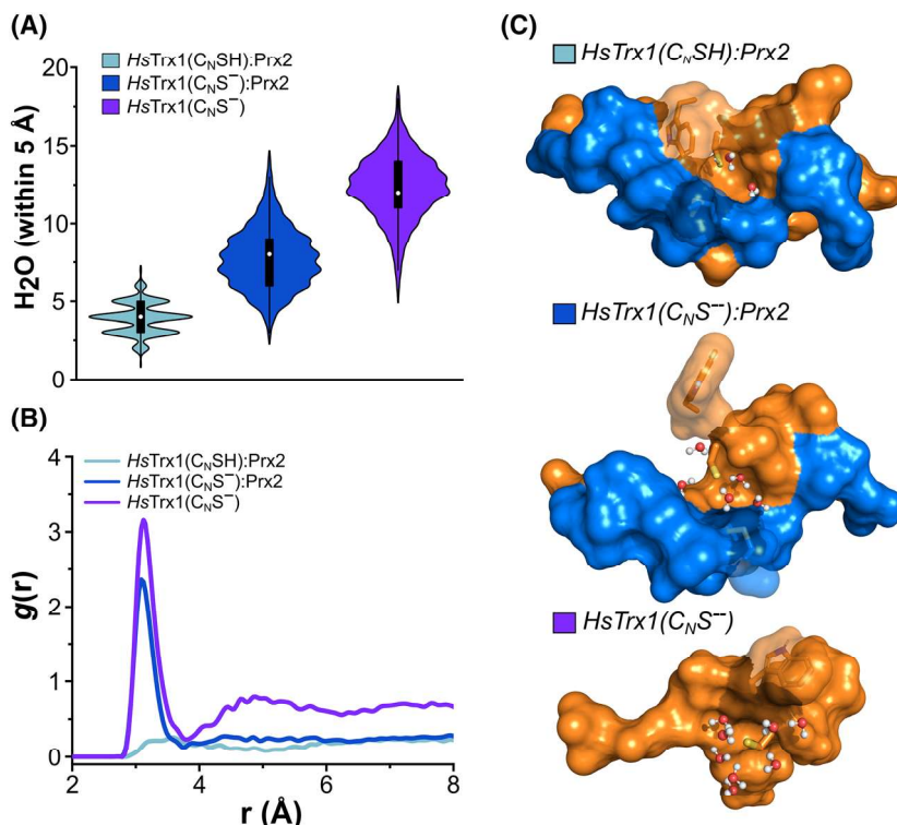
Fig. 7. The Prx2-Trx complex shields C N S - from the solvent. (A) Violin plot of the distribution of water molecules within 5 Å of C N sulfur atom during the simulated time. C N SH, C N S - and C N S - without Prx2 are compared. (B) Radial pair distribution function ( g ( r )) of water around C N sulfur for the three situations. Data in A and B represents the distribution of values for 1000 frames ( n = 1000) of each 500 ns simulation (one per condition). (C) Structural representation of the water molecules surrounding C N sulfur. W31, C N and the Prx2 disulfide are represented as sticks (behind the transparent surface), while water molecules are depicted as ball and stick. Surface colors orange and blue represent HsTrx1 and Prx2, respectively, structures generated with PyMOL Molecular Graphics System, Version 2.5.5 Schrödinger, LLC.
