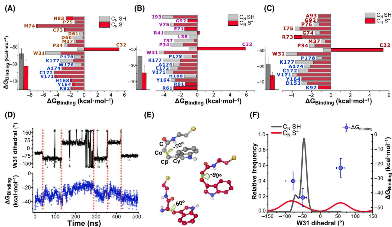
Fig. 6. Effect of C N protonation on Prx2-Trx interaction. Per residue decomposition of the \Delta G_{\text{Binding}} of the Prx2-Trx complex, for A HsTrx1 , B HsTrx2 , and C EcTrx , in all cases C N SH (gray) and C N S - (red) are compared. The insets represent the overall \Delta G_{\text{Binding}} . Residue names colored according to each Trx and blue those of Prx2. In A–C, bars represent the average of the per residue decomposed \Delta G_{\text{Binding}} calculated for 1000 frames ( n = 1000 ) of 500 ns MD simulations (one per complex and condition). The error bars in the insets represent the SD of the normal distribution of the data. (D) Time courses of W31 dihedral (black) and \Delta G_{\text{Binding}} (blue) values against the simulated time. The red-dashed lines indicate the time correspondence of the “jumps” in the properties. Data in D is the result of one simulation. (E) Ball and stick representation of W31 and C32 at the indicated W31 dihedral values, structures generated with PyMOL Molecular Graphics System, Version 2.5.5 Schrödinger, LLC. (F) Normalized relative frequency of HsTrx1 W31 C-α-Cβ-Cγ dihedral throughout the simulation for C N SH and C N S - . The \Delta G_{\text{Binding}} of the complex at values -80°, -50° and 60° is represented as blue circles. Blue points represent the average \Delta G_{\text{Binding}} for 3 W31 dihedral regions (-50°, -80°, 60°). Error bars represent the standard deviation of the dihedral (horizontal) and energy (vertical) values of 300 frames ( n = 300 ) in each region. The curves represent the Kernel-Smooth distribution of 1000 frames ( n = 1000 ) of 500 ns MD simulations (one per condition).
