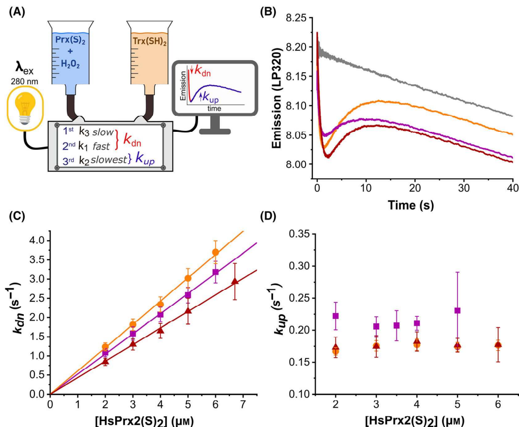
Fig. 2. Reduction of Prx2 by Trx. (A) Scheme of the rate-limiting approach. (B) Time courses of reduction of 4 \mu\text{M} Prx2S 2 by 0.2 \mu\text{M} Trx(SH) 2 in the presence of 1 \mu\text{M} H 2 O 2 . The lines are averages of 10 runs with HsTrx1 (orange), HsTrx2 (magenta), or EcTrx (red), and the gray line is a control experiment without Trx. The best fit to Eqn (4) yields two rate constants: one for the descending part of the time courses ( k_{\text{dn}} , C) and one for the ascending part ( k_{\text{up}} , D), in all cases error bars represent SD. Best fit slopes of panel C and y-intercepts of panel D are in Table 1.
