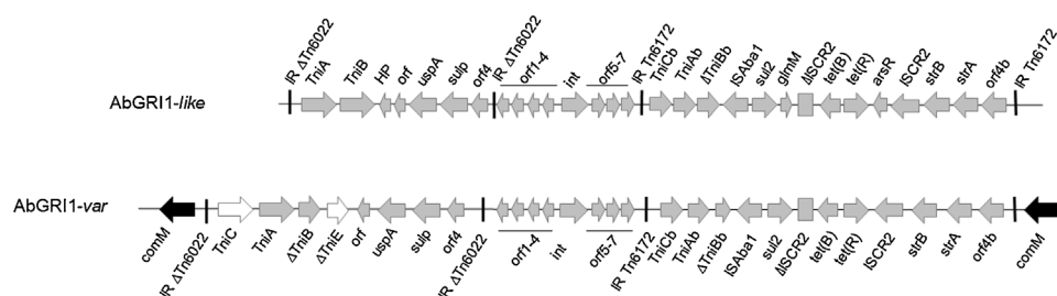
Fig. 4. Comparison of the genetic structures of the AbGRI1-like and AbGRI1-var islands in Ab376. The grey and white arrows indicate the shared and unshared genes between them.
