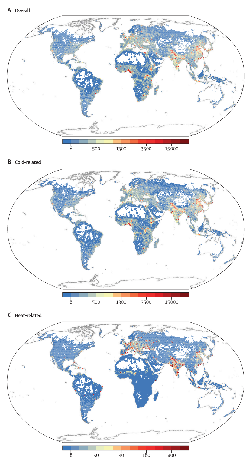
Figure 2: Average annual excess deaths due to non-optimal temperatures in 2000–19 at a spatial resolution of 0.5^\circ \times 0.5^\circ . (A) Overall annual excess deaths. (B) Cold-related annual excess deaths. (C) Heat-related annual excess deaths. Only grids with at least one annual death were included.
