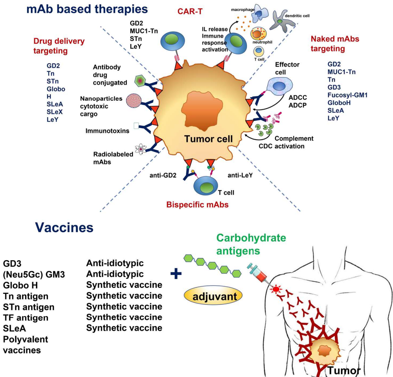
Figure 1. Schematic representation of antitumor strategies based in antibodies and vaccines targeting TACAs (Tumor Associated Carbohydrate Antigens). mAbs (monoclonal antibodies); CAR-T (Chimeric antigen receptor-T); STn (sialyl Tn); SLeA (sialyl Lewis A); SLeX (sialyl Lewis X); LeY (Lewis Y); ADCC (Antibody-Dependent Cell-mediated Cytotoxicity); ADCP (Antibody-Dependent Cellular Phagocytosis); CDC (complement-dependent cytotoxicity).
