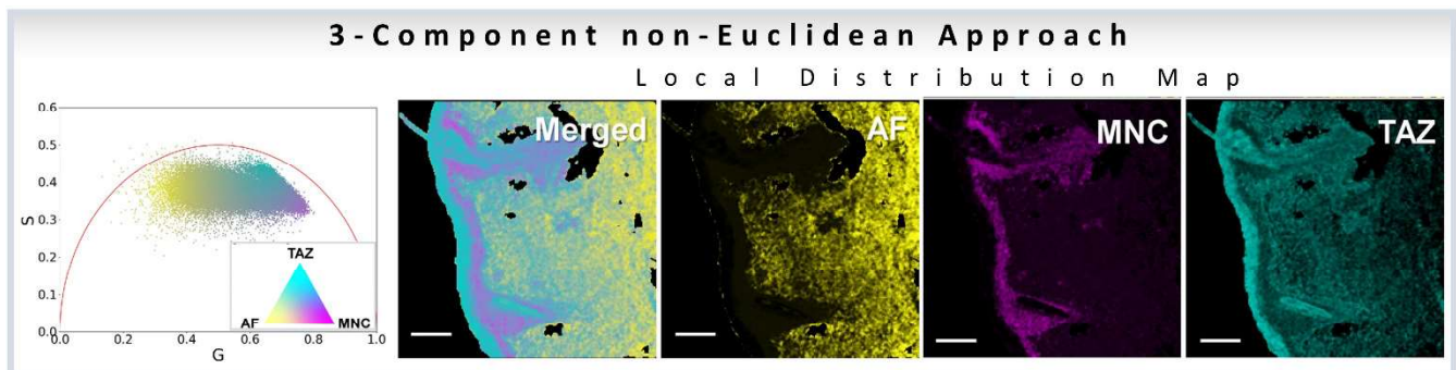
Figure 11. Quantification and visualization of minocycline (MNC), tazarotene (TAZ) in ex vivo skin samples. Quantification of the drug distribution for the three components: MNC, TAZ and autofluorescence based on the non-Euclidean geometry results in distribution patterns for the three components, as shown by yellow for AF, cyan for TAZ, and magenta for MNC, respectively. The scale bar is 100 \mu\text{m} . (Figure adapted from [36]).
