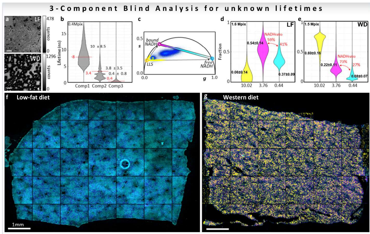
Figure 12. Biological example of three-component blind analysis (unknown lifetimes of the components) using harmonics of phasor. Study of metabolic changes in liver tissue samples using three-component blind recovery analysis. (a) Intensity images of livers of mice fed with low-fat diet (LF, top) or Western diet (WD, bottom) (b) Recovered lifetimes using three blind components are represented as gray violin plots and the median \pm SD. Expected lifetime values for individual species are shown with a horizontal red line. (c) Phasor plot for the first harmonic (second and third harmonics phasor plots are not shown). Colored circles on the universal circle indicate the recovered first harmonic phasor position of free NADH (cyan), protein-bound NADH (purple), and LLS (yellow). Fractional intensity distributions of the three components in LF (d) and WD (e) samples. Color-coded phasor-FLIM liver images of mice fed with LF (f) or WD (g). The free-to-protein-bound ratio (not including LLS) is color-coded using a magenta to cyan colormap with a yellow overlay for LLS (with values above 75%). (Panels adapted with permission from [38]).
