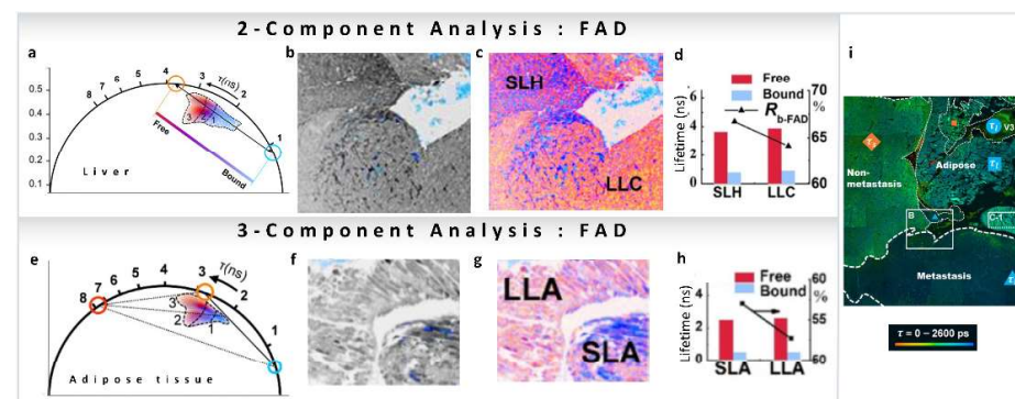
Figure 9. (a–e). Metabolic imaging of FAD using multiple components. FAD FLIM data of hepatocytes and cancer cells of metastatic pancreatic cancer (panels adapted with permission from [48]). (a) Phasor plot showing linear combination of two components, short lifetime (protein-bound FAD, blue cursor) and long-lifetime (free FAD, orange cursor). (b) Grayscale (accumulated photon counts) of hepatic cells. (c) Pseudo-color image showing different lifetime species in the short-lifetime hepatocytes (SLH) and long-lifetime cancer cells (LLC). (d) Lifetimes and ratios ( R_{b-FAD} ) of the components. (e,f) FAD FLIM data of adipocytes of metastatic pancreatic cancer. (e) Phasor plot showing three-component analysis, short lifetime (protein-bound FAD, blue cursor), long-lifetime (free FAD, orange cursor) and another much longer lifetime component (red cursor). (f) Grayscale (accumulated photon counts) of adipose cells. (g) Pseudo-color image showing different lifetime species in the short-lifetime adipose (SLA) and long-lifetime adipose cells (LLA). (h) Lifetimes and ratios ( R_{b-FAD} ) of the components. (i) Metabolic features of liver section (large-field image) of metastatic colonization revealed using FLIM. (Panels adapted with permission from [48]).
