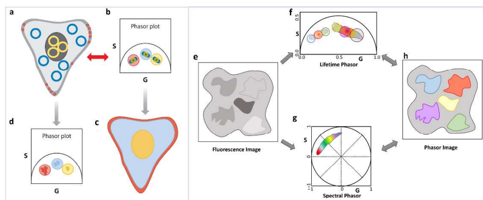
Figure 6. Reciprocity principle and multidimensional phasor approach. (a–d) Reciprocity principle. Phasor signatures from different parts of the image (a) can be segregated (b). Selection of these different phasor clouds (red, blue and yellow circle, (b) allow the image points they originated from to be selected and the image to be colored accordingly (c). Similarly, parts of the image can be selected (blue, yellow and red cursors, (a) and the corresponding phasor points can be highlighted (d). (e–h) Multidimensional phasor approach. When the exact same area of a sample is imaged (e) in different moieties using phasor approach, phasor FLIM (f) and spectral phasor (g), then the phasor image (h) can be color-coded according to one selection, in this case, lifetime phasor (f). Using the reciprocity principle, the spectral signatures of those lifetime phasor selections can be identified (g).
