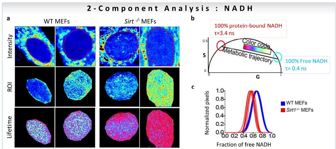
Figure 7. Biological examples of fractional intensity contributions of two species based on linear combination of phasor-FLIM. Two-component analysis (known lifetimes of the components) using a graphical approach for metabolic imaging using free to bound NADH. (a–c) Nuclear NADH metabolism is dependent on the activity of Sirt1. (a) Intensity and lifetime (FLIM) images for WT and Sirt1 -/- MEFs. Two representative images per condition are shown. (b) Phasor plot shows the color scale used to visualize the fraction of free/bound NADH along the metabolic trajectory in FLIM images. (c) Histograms show comparative analyses by overlapping the fractional free NADH distributions from WT (cyan) and Sirt1 -/- (red) MEFs. Free NADH fraction is represented in the x axis, where 1 = 100% free NADH. (Panels adapted with permission from [17]).
