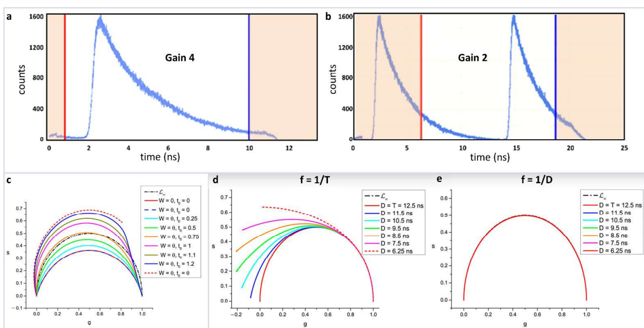
Figure 5. Improper transformation of fluorescence lifetime decays to phasor plots and their effects.
