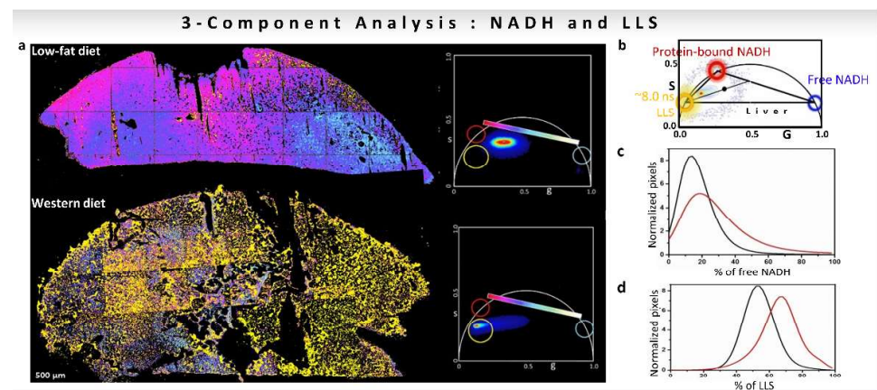
Figure 8. Three-component analysis (known lifetimes of the components) using a graphical approach for understanding of effect of diet on mice liver. (a–d) Quantification of the presence of oxidized lipids in mice fed with Western diet vs. low-fat diet using three-component analysis. (a) Color-coded phasor-FLIM liver images of mice fed with low-fat diet (LF) or Western diet (WD). The free-to-protein-bound ratio (not including LLS) is color-coded using a magenta to cyan colormap with a yellow overlay for LLS. The corresponding phasor plots are shown for each condition. (b) Blue, red and yellow circles on the phasor plot represent the phasor positions of free and protein-bound NADH, and long lifetime species (LLS), respectively. Histograms showing the percentage of free NADH (c) or LLS species (d) for the LF (black) and WD (red) diet, respectively. (Panels adapted with permission from [32]).
