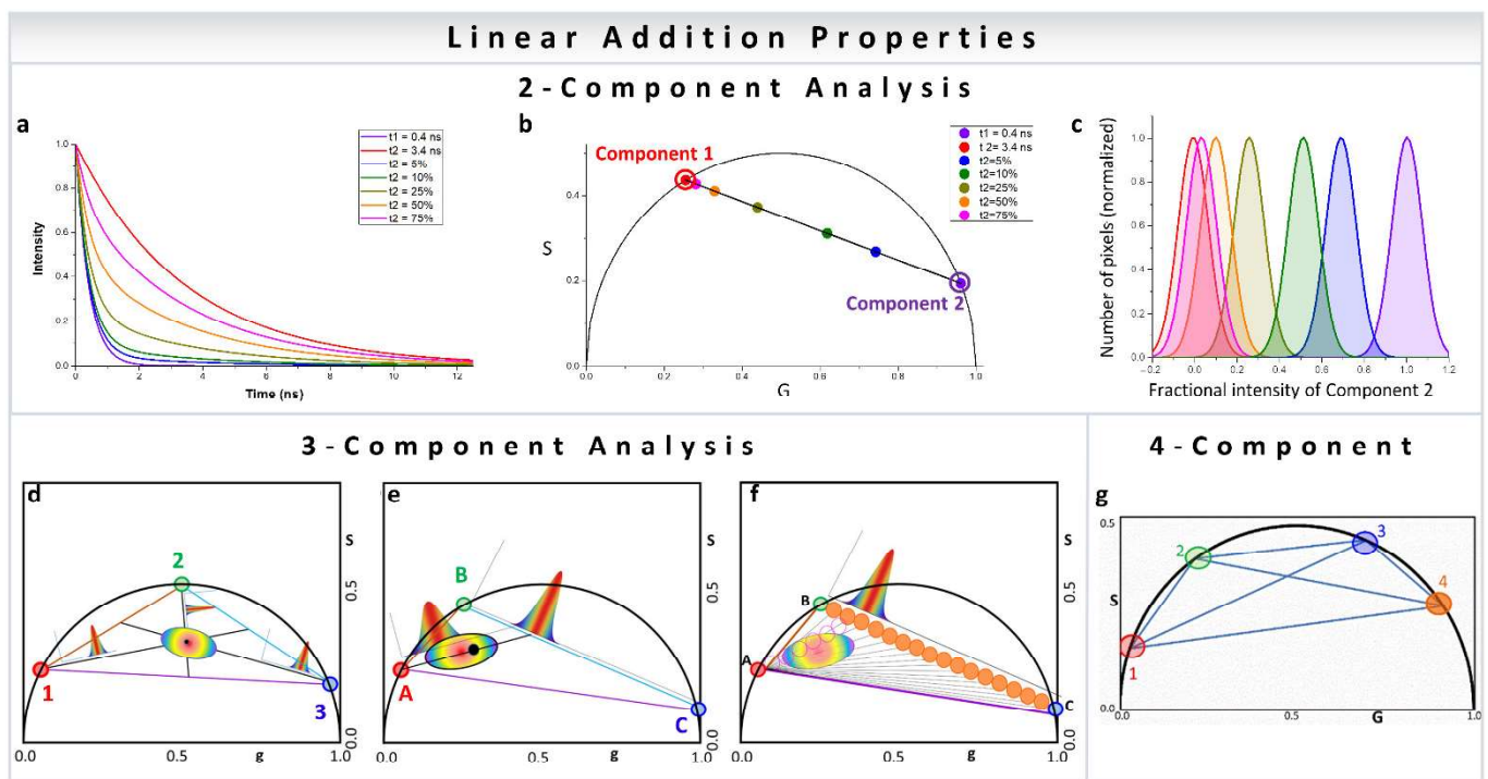
Figure 2. Multicomponent analysis in phasor plot. (a–c) Two-component analysis using phasor approach. (a) The intensity decays were calculated using the lifetime of free NADH (0.4 ns, violet) and protein-bound NADH (3.4 ns, red). Different fractions of free to bound NADH were used for calculating the decays in the middle. In increasing percentage of bound NADH—5% (blue), 10% (green), 25% (yellow-green), and 50% (orange). (b) The corresponding phasor positions were calculated, and they appear along the metabolic trajectory [18], connecting the positions of free (violet) and bound (red) NADH. Two-component analysis allows the distribution along the line joining the phasor positions of the individual components to be calculated, as exemplified by free and protein-bound NADH here. However, this is valid for any two original phasor components. (d–f) Three-component analysis using phasor approach. (d) The lines joining the individual cursor positions (red, blue and green), forming the vertices of the triangle and the phasor point whose fractional intensity contributions are being calculated (black), are extended to the opposite side of the triangle. The distances of the vertices from the black point are used for the calculation of fractional intensity contribution (the graphs). (e) Calculation of three components where two components are related, e.g., free and protein-bound NADH. In this case, the presence of the third component shifts the distribution towards that third component and away from metabolic trajectory. This distance can be converted to the fractional intensity of free NADH and plotted (the graph between green and blue points) or fractional intensity of third species (the graph along the line joining the red vertex and the opposite line). (f) Graphical analysis of three components. A cursor of a given size is scanned along point A and another point in line BC to calculate the fraction of the third component along the axis and then this process is combined for different points on BC to create the fraction of the third component. The number of points along each of these black lines are counted by scanning (orange cursors) and plotted along the coordinates of BC to calculate the fraction of free NADH. (Panels d–f adapted with permission from [32]). (g) Four-component analysis using phasor approach. Representation of four species with different phasors indicated by the number 1 to 4 (1, red; 2, green; 3, blue; 4, orange). In this case, the individual species are single exponentials since they are on the universal semicircle. The position of a phasor point in a single harmonic inside this quadrangle can be defined by multiple triangles. Multiple harmonics are needed to obtain unique solution for the contribution of the four components. (Panel g adapted with permission from [35]).
