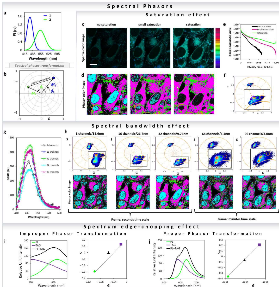
Figure 13. Spectral phasor transformation properties and important considerations. (a,b) Simulation of two gaussian curves with different centers of mass and FWHM (a), and the transformation into the spectral phasor plot (b). Note that while the blue curve has a longer M and short \Phi (meaning bluer and narrow spectra), the green curve has a shorter M and larger \Phi (meaning greener and broader spectra). The line that joins the two components represents the linear combination for all the different fractions between component 1 and 2. (c–f) Effect of the spectral saturation on the spectral phasor transformation. (c) Spectral and (d) pseudo-color images of HeLa cells stained with ACDAN ( 5 \mu M final concentration), imaged at different laser powers (with increasing saturation from left to right). Scale bar 10 \mu m . (e) The corresponding intensity histograms. (f) Based on a set of cursors in the phasor plot for the no-saturation condition, the effect of saturation and changes in the location of the phasor cloud by aberrant transformation can be seen. The phasor plot consists of the clouds from the three images (no-saturation, small-saturation, saturation). (g,h) Effect of the spectral bandwidth on the spectral phasor transformation. (g) The average spectra of the pixels from each image are shown here (8, 16, 32, 64 and 96 channels, respectively). Note that counts were kept in a similar range for comparison purposes. The data were acquired using a 32-channel spectral on the Zeiss LSM 710, therefore by default it records spectra using 32 parallel channels. Note that increasing resolution (increasing number of channels and decreasing the bandwidth per channel) of the phasor transformation results in a broader cloud (due to the poorer S/N per channel). The second noticeable
