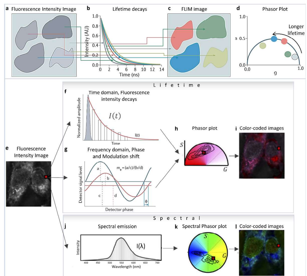
Figure 1. Phasor transformation. (a) Fluorescence lifetime imaging microscopy (FLIM) measures the fluorescence lifetime decays in different parts of the image (b), and color-codes areas (c) according to their decay times (b) or their phasor clusters (d). The resulting phasor plot (d) represents species
