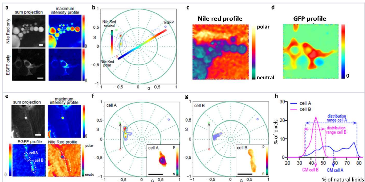
Figure 14. Analysis of the lipid metabolic profile of EGFP+ cells in the zebrafish line with the transgene fabp4 (−2.7): EGFPcaax. (a–d) Schematic representation of the three-component analysis for the Nile Red fluorescence in the presence or absence of the EGFP fluorescence. EGFP− cells let us define the neutral-polar Nile Red trajectory and EGFP+ cells without Nile Red, allowing us to identify the phasor position of the third component (GFP, identifying the specific cell-adipocyte). Notice that after three cursors were defined, a triangle has all possible linear combinations, and the third component was used to analyze the Nile Red information from the cells of interest. Two scales of colors were defined for the Nile Red profile and the EGFP profile. (e–g) Examples for the analysis of the Nile Red profile in two cells from the zebrafish larvae with the transgene fabp4 (−2.7): EGFPcaax at 8 dpf. Notice that the Nile Red spectrum characteristic in the EGFP+ cell is pulled towards the third component, which enables the identification and analysis of the Nile Red profile for these cells avoiding confusing the information coming from Nile Red in GFP− tissue. (h) “Nile Red axis” is defined as a normalized fraction of pixels along the Nile Red profile. The histogram shows the percentage of polar lipids in the region of the cell analyzed. Scale bars: A: 20 \mu m; B: 50 \mu m. (Panels adapted with permission from [56]).
