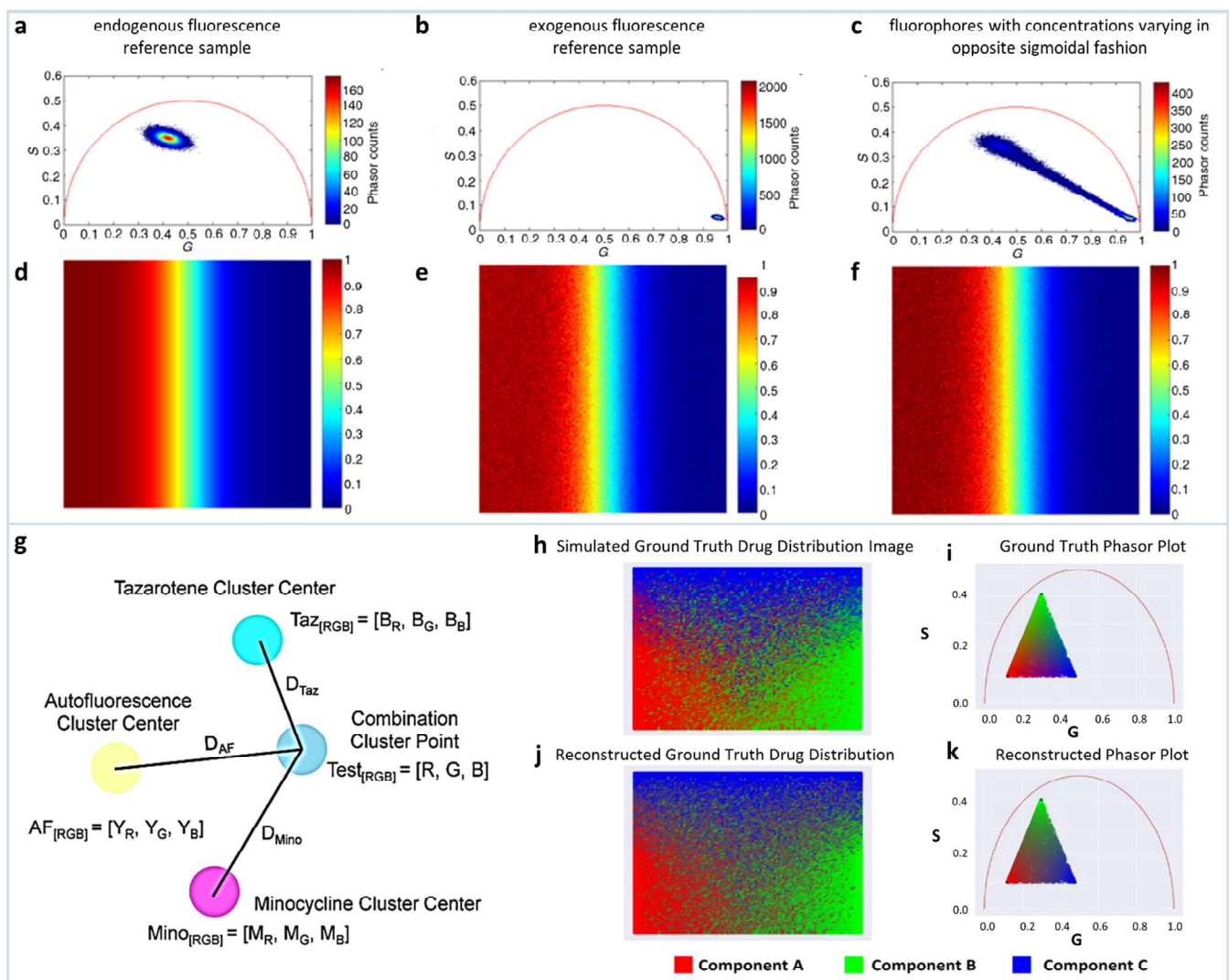
Figure 4. Multicomponent analysis based on non-Euclidean geometry. (a–c) Simulation to validate the proposed non-Euclidean separation algorithm. (a) Phasor plot of simulated endogenous fluorescence reference sample, (b) exogenous fluorescence reference sample, (c) fluorophores with concentrations varying in opposite sigmoidal fashion. (d–f) Three-component analysis of drug distribution using non-Euclidean geometry. Simulated endogenous fluorescence contribution to the test image. Estimation of endogenous fluorescence contribution computed using the traditional Euclidean method and using the proposed non-Euclidean method. (Panels a–f adapted with permission from [37]). (g–k) Distance-based method of assigning phasor plot pixel colors in a multicomponent fluorescence contribution analysis algorithm. (g) A sample setup of a distance calculation. Yellow, cyan, and magenta points → the center of exogenous (autofluorescence), and two endogenous reference clusters (TAZ and MNC), respectively, and blue point → a phasor point from the tissue sample. (h,i) Simulated ground truth tissue map of drug distribution and calculated phasor plot. (j,k) Reconstructed tissue drug distribution using the multicomponent phasor analysis algorithm and phasor plot. (Panels g–k adapted with permission from [36]).
