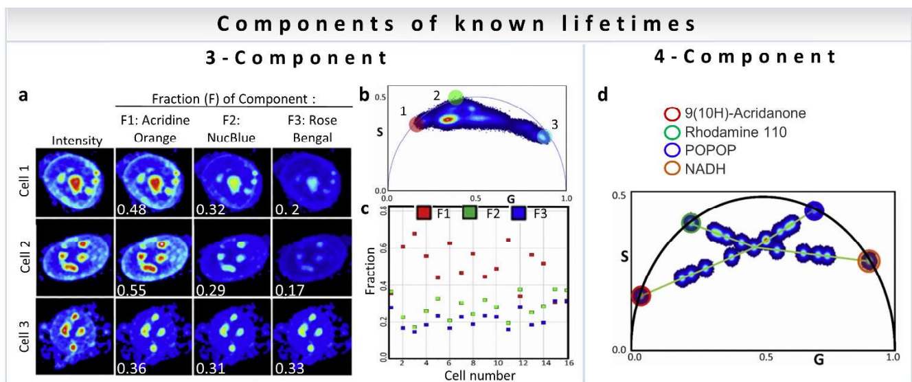
Figure 10. Multiple-component fraction analysis (known lifetimes of the components) to calculate average from an image. (a–c) Three-Component fraction analysis (known lifetimes of the components). Obtaining intensity fractions of three nuclear dyes mixed in live cells with three-component analysis. (a) Representative images of three different cells, all of them stained with the three nuclear dyes: Acridine Orange (Fraction 1, F1), NucBlue (F2) and Rose Bengal (F3). Total intensity (column 1) and normalized recovered images of the intensity fractions (average fraction written in white) of the three dyes are shown in columns 2–4. (b) Phasor plot corresponding to 47 different cells. The colored circles indicate in the phasor plot the phasor position for the first harmonic at 80MHz of Acridine Orange (red circle), NucBlue (green circle) and Rose Bengal (blue circle). (c) Fractional intensity values obtained with the three-component analysis of 16 cells. (d) Four-Component analysis (known lifetimes of the components) using harmonics. (Panel adapted with permission from [35]). Phasor plot corresponding to 22 different mixtures of 9(10H)-Acridanone (red circle, 12 ns), Rhodamine 110 (green circle, 3.8 ns), POPOP (blue circle, 1.4 ns), and NADH (orange circle, 0.4 ns) (phasor positions of the pure single exponential species on the universal semicircle are shown by circles). To solve the four-component system, the phasor plot was measured at 80MHz (first harmonic) and 160 MHz (second harmonic, not shown). (Panels adapted with permission from [35]).
