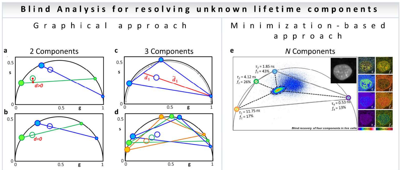
Figure 3. Blind component analysis for resolving unknown lifetimes in phasor plot—assuming the components have mono-exponential lifetimes. (a,b) Graphically finding two unknown lifetime components and their relative fractional intensities. (a) Universal circle is scanned for candidate components. For each position of the first component (small blue dot), a line is drawn through the data point (blue empty circle) and the second point is found where the blue line meets the universal circle (large blue filled circle). The second harmonic ( h_2 ) for the candidate components are obtained mathematically: small green dot and the large green filled circle. A line is drawn through them (green line). (b) Solution is the only lifetime pair that has the lines (blue and green) going through the data points for the two harmonics, that is, when the distance from the green line to the green empty circle is zero. The relative fractions are obtained by the ratios between the distances from the filled dots to the empty circles on both sides of the line. (c,d) Finding the three lifetime components in the universal circle. (c) Schematic configuration of three components generating a data point (ring in the middle). As an example, the ratio between the two distances is related to the intensity fraction ( f ) of the component located in the short lifetime region; f_1 = d_1 / (d_1 + \tilde{d}_1) . In the same manner, the other two fractions can be obtained for the other two components. (d) Solution to the three-component problem is the only combination of components such that the three fractions are the same in each of the triangles composed of the three harmonics (blue–green–orange). The short, medium, and long lifetime components in each harmonic are depicted by increasingly larger filled circles. (e) Minimization-based approach. This general algorithm can technically be solved the problem to N number of components depending on noise propagation in the multiple harmonics. (Panels a–e adapted with permission from [38]).
