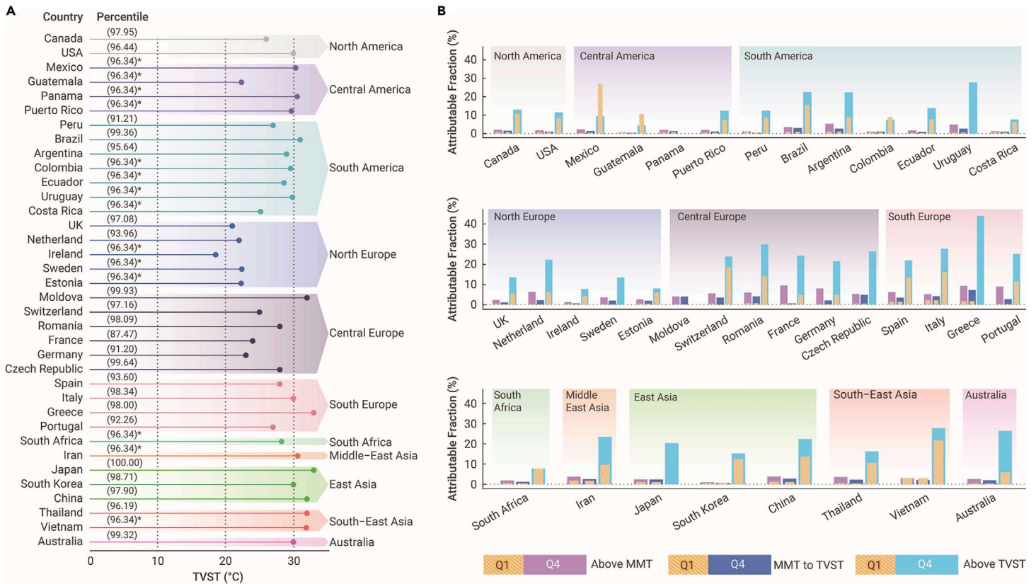
Figure 2. Figure 2 Fractions of all-cause mortality attributable to heat exposure by temperature variability (A) TVST identified for each country for TV. *For countries without identifiable TVST, the quantile threshold of the 96.34th percentile (the average of all identifiable country-specific TVSTs) in the temperature distribution for each country was used. (B) Comparison of AFs of mortality due to heat exposure for Q1 and Q4 of TV in each country, stratified by TVST. Yellow bars: the AFs for the Q1 of TV; purple bars: the AFs of mortality due to heat exposure above MMT for the Q4 of TV; dark blue bars: the AFs of mortality due to heat exposure from MMT to TVST for the Q4 of TV; light blue bars: the AFs of mortality due to heat exposure above TVST for the Q4 of TV. AF = attributable fraction; MMT = minimum mortality temperature; Q1 = the 1st quartile; Q4 = the 4th quartile; TV = temperature variability; TVST = temperature variability sensitive heat threshold.
