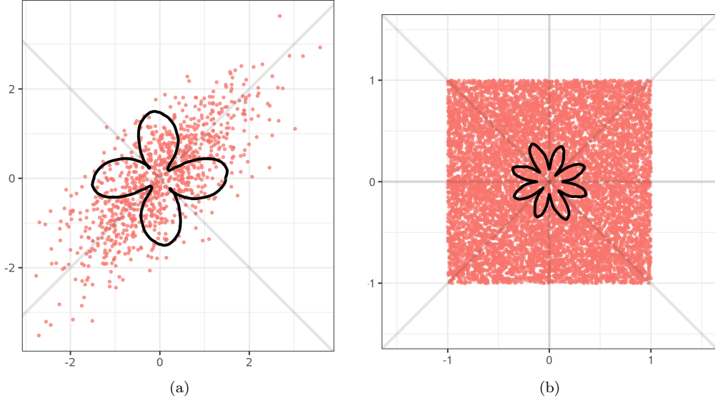
Figure 2: In each subfigure, simulated data are depicted as red points; the black line illustrates the estimate of the function g in a polar plot format, and the gray lines indicate the true axes of symmetry. Subfigure (a) represents a bivariate normal distribution ( Scenario 1 ), while subfigure (b) represents a uniform distribution within a square ( Scenario 2 ).
