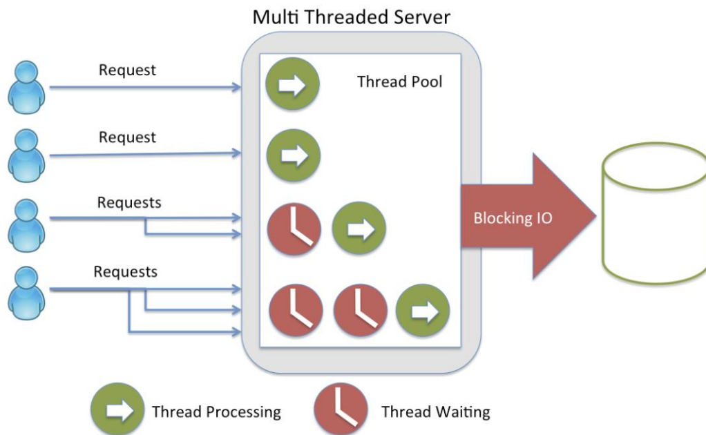
Figura I2 – Multi Threaded Server
