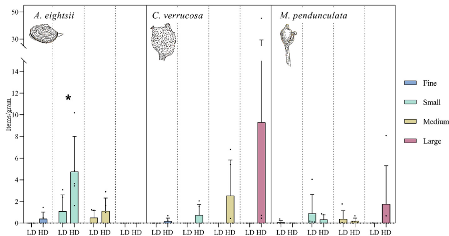
Fig. 3. Barplot indicating the items per gram for the different particle size fractions (fine: 10–20 \mu\text{m} , small: 45–53 \mu\text{m} , medium: 106–125 \mu\text{m} , and large: 850–1000 \mu\text{m} ) in the two treatments (LD: low dose, HD: high dose) and the three species: Aequioldia eightsii , Cnemidocarpa verrucosa , and Molgula pedunculata . (Bars represent the mean, whiskers the standard deviation, dots represent the value for each replicate, and the asterisk represents statistical differences between treatments in a size fraction).
