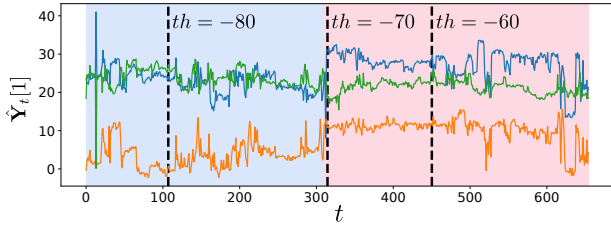
Fig. 3. The evolution of \hat{\mathbf{Y}}_t[1] for entries (i, j) \in \mathcal{O} in the RSSI graph. The background color indicates the change-point estimated through our embedding and the vertical lines by applying different thresholds th to the graph.
