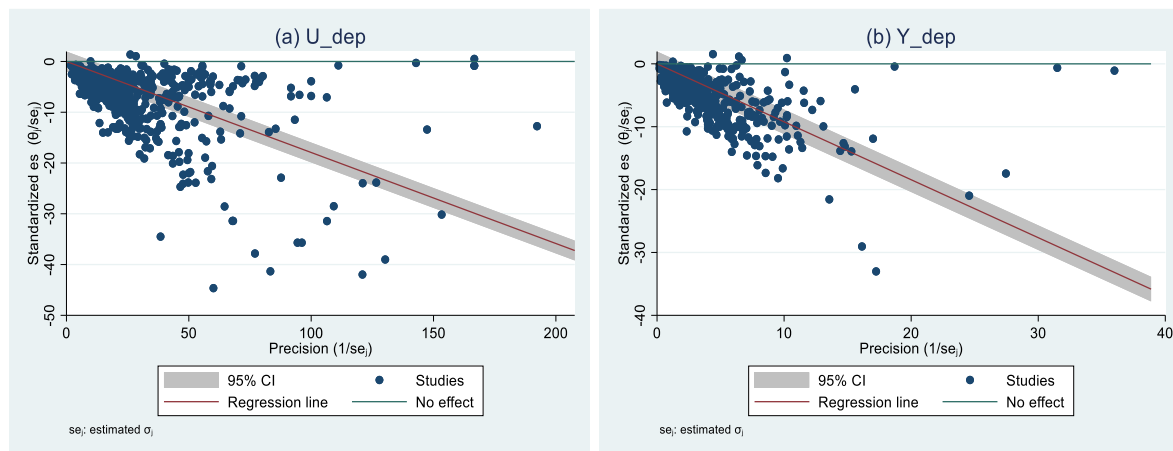
Fig. 4. Galbraith plots.
