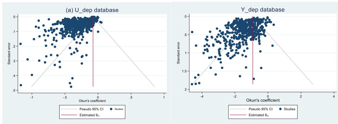
Fig. 2. Funnel plot.
