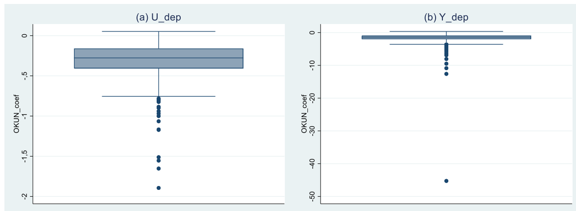
Fig. 5. Box plots.
