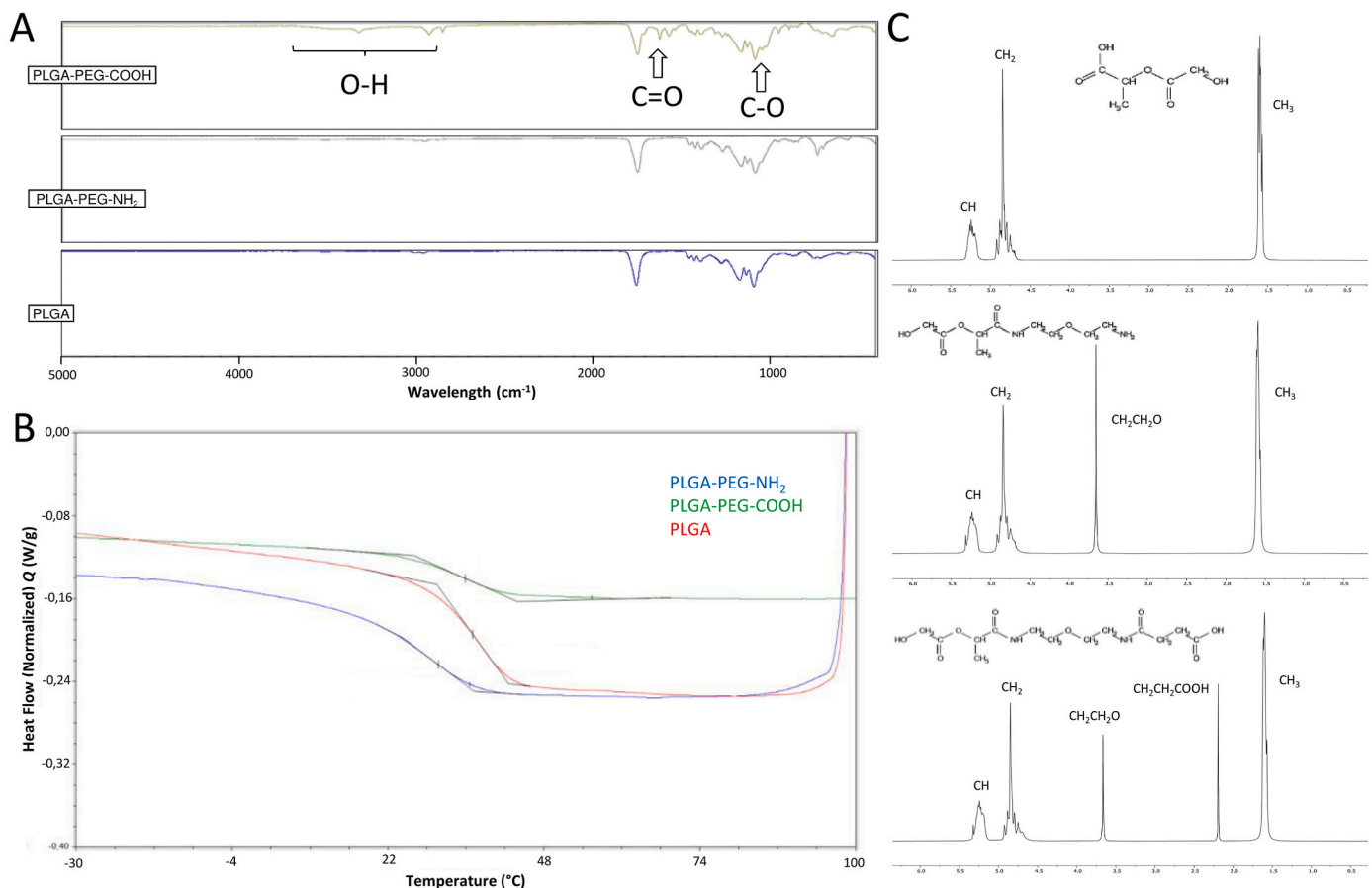
Fig. 1. Chemical validation of PLGA-PEG-COOH polymer. (A) Fourier Transform-Infrared spectra of PLGA-PEG-COOH, PLGA-PEG-NH 2 and PLGA. The typical stretchings for O-H, C=O and C-O bounds were annotated. (B) Differential scanning calorimetry thermograms of PLGA polymers. (C) 1 H NMR spectra of PLGA (top), PLGA-PEG-NH 2 (middle) and PLGA-PEG-COOH (low) copolymer in CDCl 3 . Each peak is annotated with the corresponding group.
