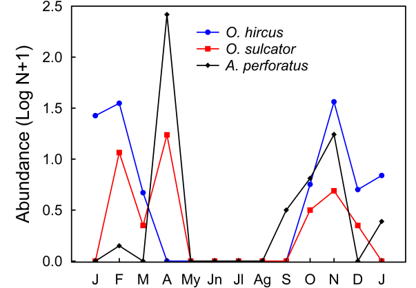
Fig. 7. Monthly flight activity of dung beetle species sampled during 2010 in Eucalyptus plantation in Puntas de Sauce Maciel (Florida, Uruguay).
