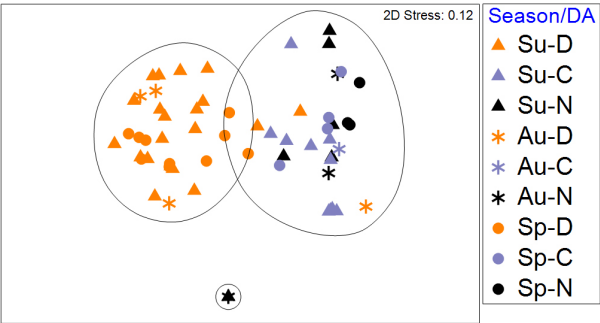
Fig. 4. Non-metric multidimensional scaling of diurnal (D), crepuscular (C) and nocturnal samples (N) of dung beetles in autumn (Au), spring (Sp) and summer (Su) in the open pasture in Puntas de Sauce Maciel (Florida, Uruguay).
