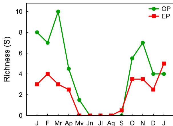
Fig. 3. Monthly variations (mean/trap) in species richness of Scarabaeidae in pitfall traps located in open pasture (OP) and Eucalyptus plantation (EP) in Puntas de Sauce Maciel (Florida, Uruguay).
