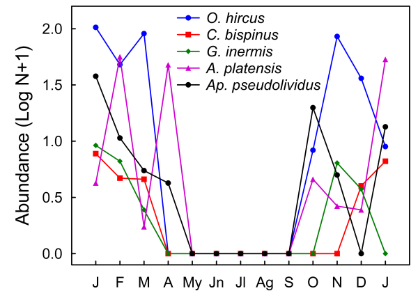
Fig. 6. Monthly flight activity of dung beetle species sampled during 2010 in open pasture in Puntas de Sauce Maciel (Florida, Uruguay).
