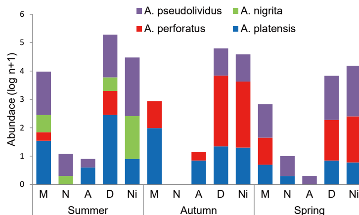
Fig. 9. Seasonal variation of daily flight activity of Aphodiinae species in a livestock ranch at Puntas de Sauce Maciel, Florida (Uruguay). (M: morning; N: noon; A: afternoon; D: dusk; Ni: night).
