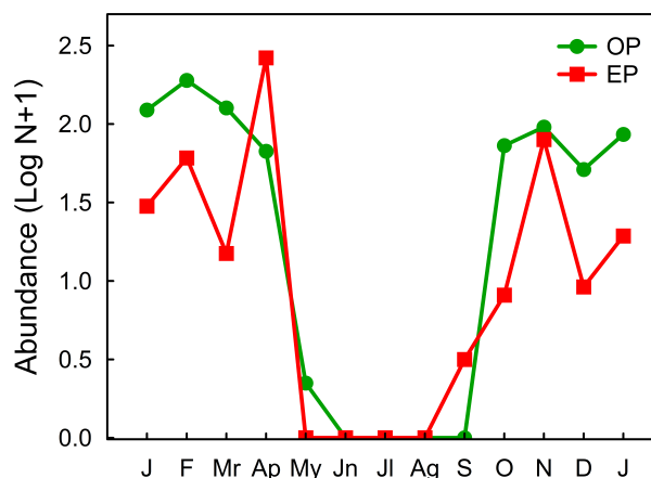
Fig. 2. Monthly variations (mean/trap) in abundance of Scarabaeidae in pitfall traps located in open pasture (OP) and Eucalyptus plantation (EP) in Puntas de Sauce Maciel (Florida, Uruguay).
