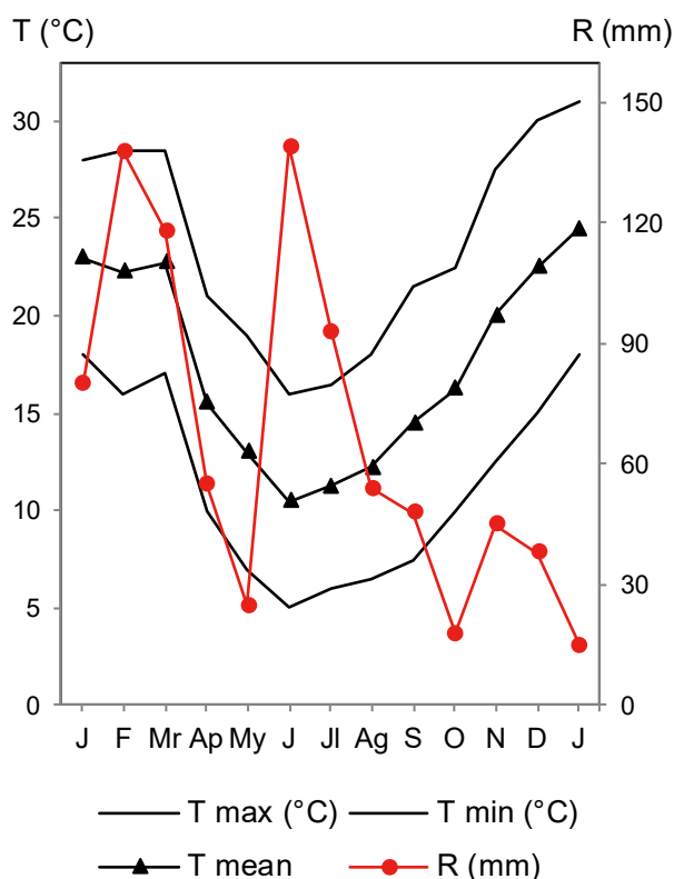
Fig. 1. Climatological recordings at Puntas de Sauce Maciel, Florida (Uruguay), from January 2010–January 2011.
