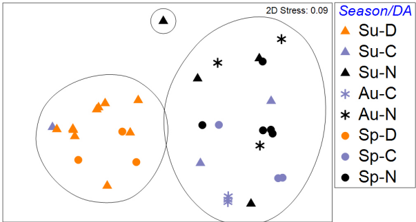
Fig. 5. Non-metric multidimensional scaling of diurnal (D), crepuscular (C) and nocturnal samples (N) of dung beetles in autumn (Au), spring (Sp) and summer (Su) in the Eucalyptus plantation in Puntas de Sauce Maciel (Florida, Uruguay).
