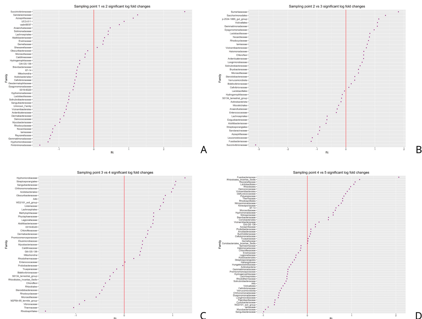
Fig. 5. ANCOM-BC significant results. Significant differences in relative abundance (q value > 0.05) at family level are shown. A. Sampling point 1 to 2. B. Sampling point 2 to 3. C. Sampling point 3 to 4. D. Sampling point 4 to 5. lfc: log fold change. lfc negative values indicate the relative abundance decreases from one sampling point to the next, positive values indicate an increase.
