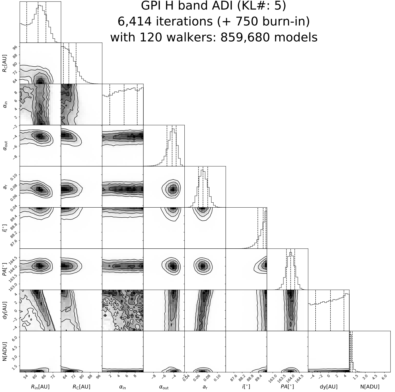
Figure A12. Posterior distribution for HD 111520 SE H -band models.
