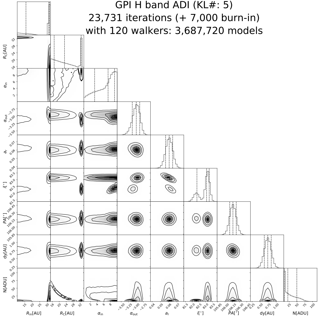
Figure A13. Posterior distribution for HD 114082 H -band models.
