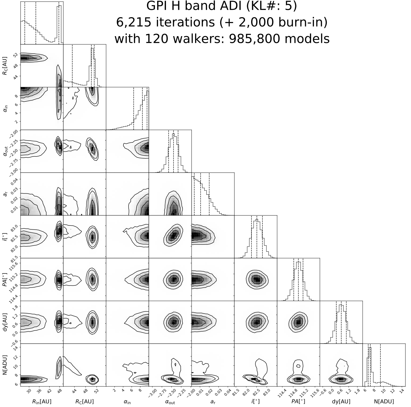
Figure A14. Posterior distribution for HD 146897 H -band models.
