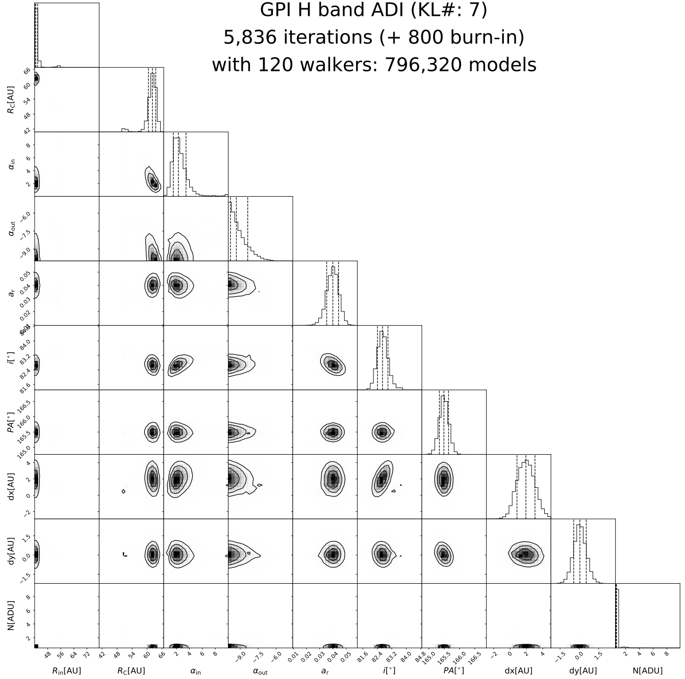
Figure A3. Posterior distribution for HD 35841 H -band models.
