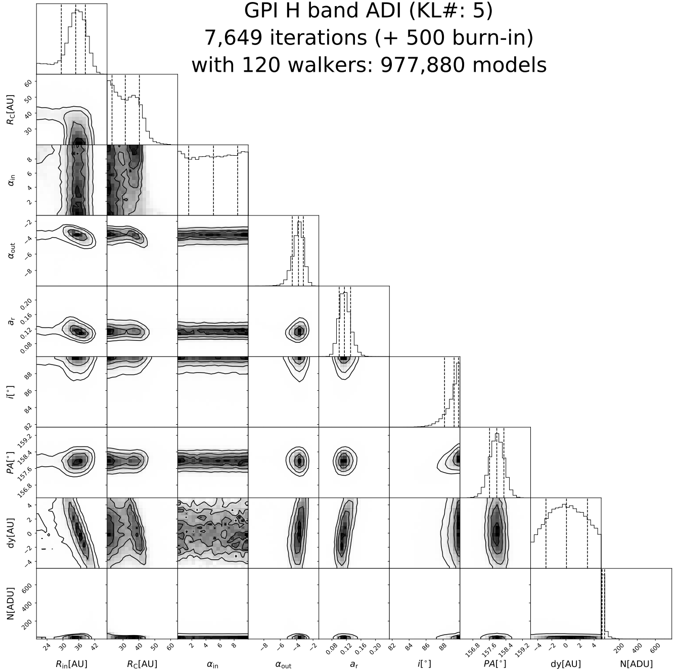
Figure A9. Posterior distribution for HD 110058 SE H -band models.
