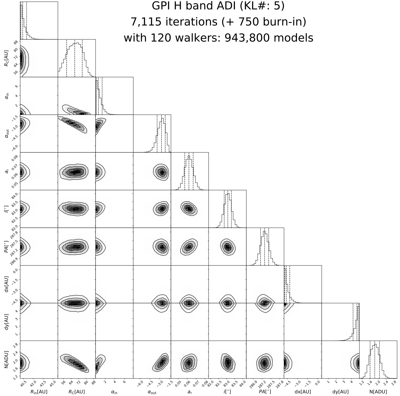
Figure A5. Posterior distribution for HD 106906 NW H -band models.
