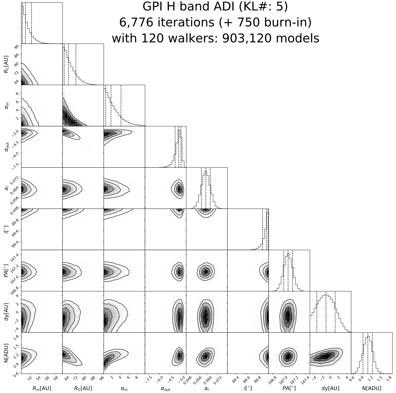
Figure A11. Posterior distribution for HD 111520 NW H -band models.
