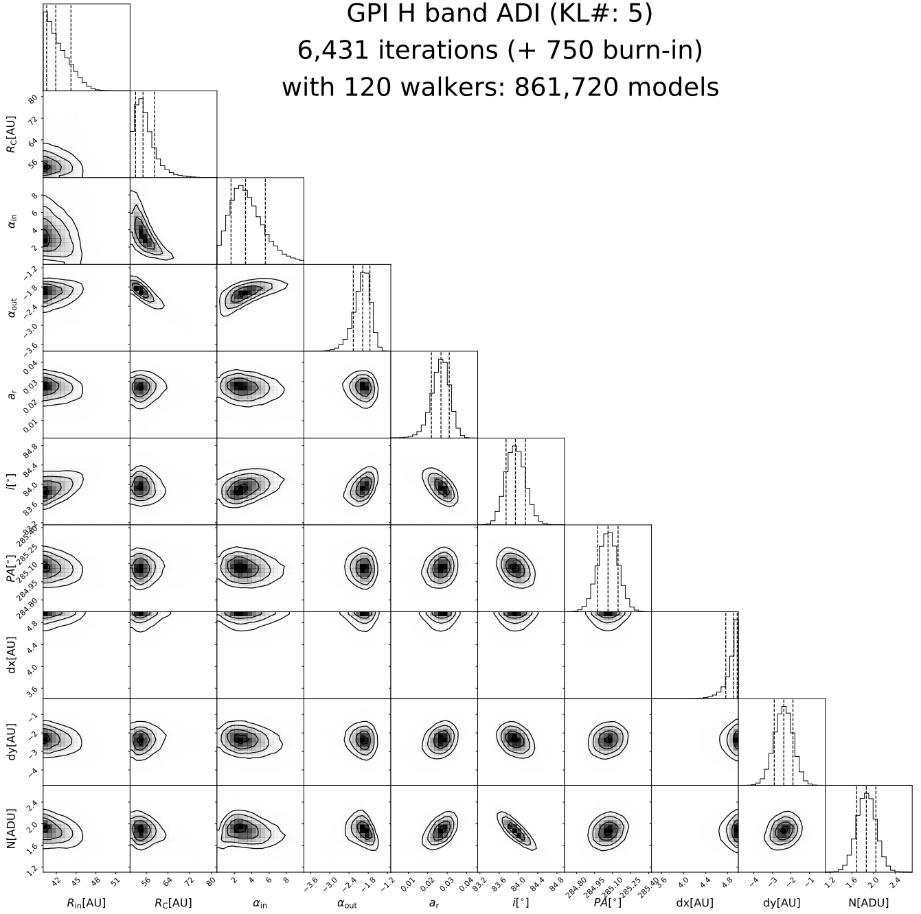
Figure A4. Posterior distribution for HD 106906 whole disk H -band models.
