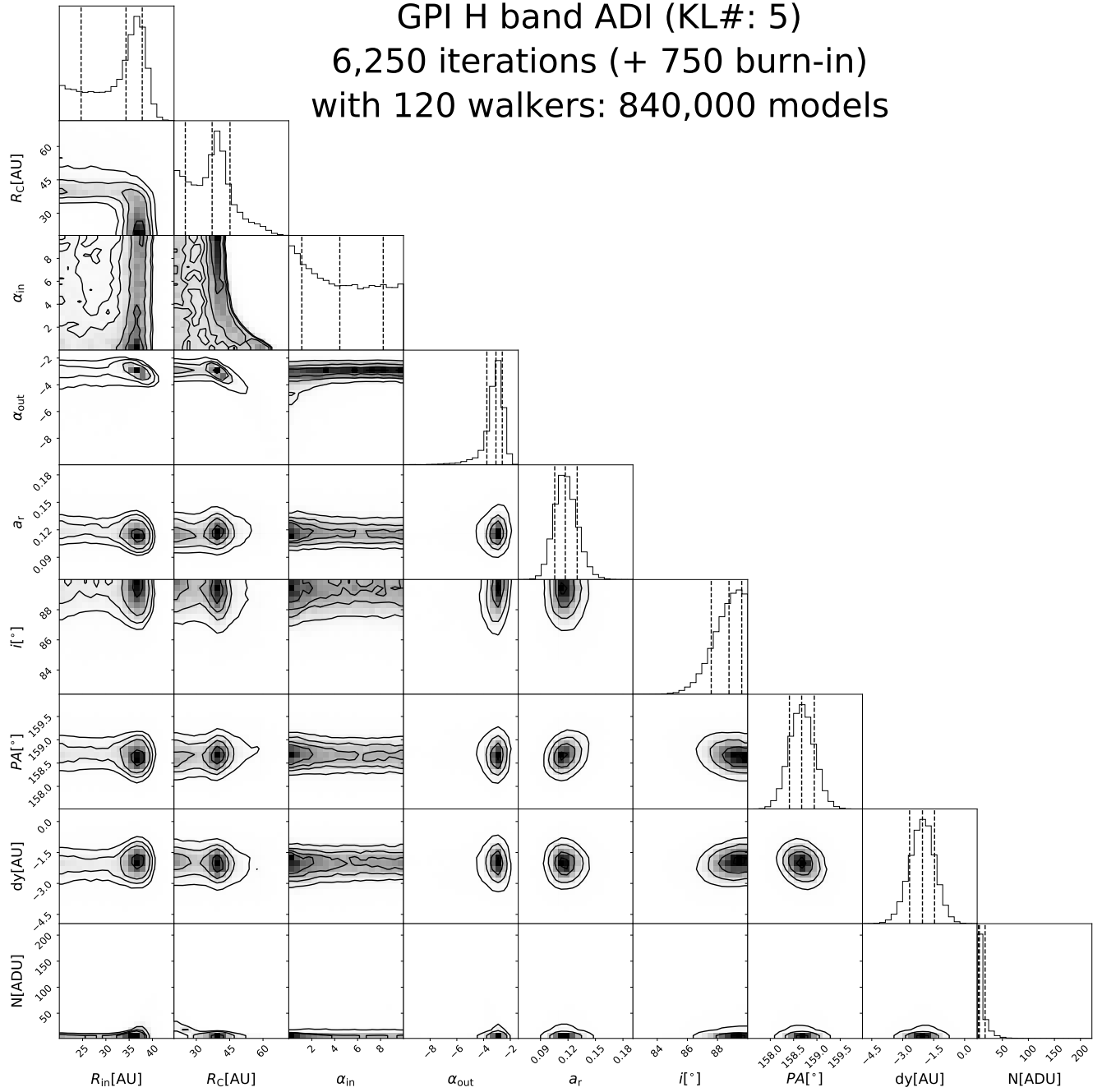
Figure A7. Posterior distribution for HD 110058 whole disk H -band models.
