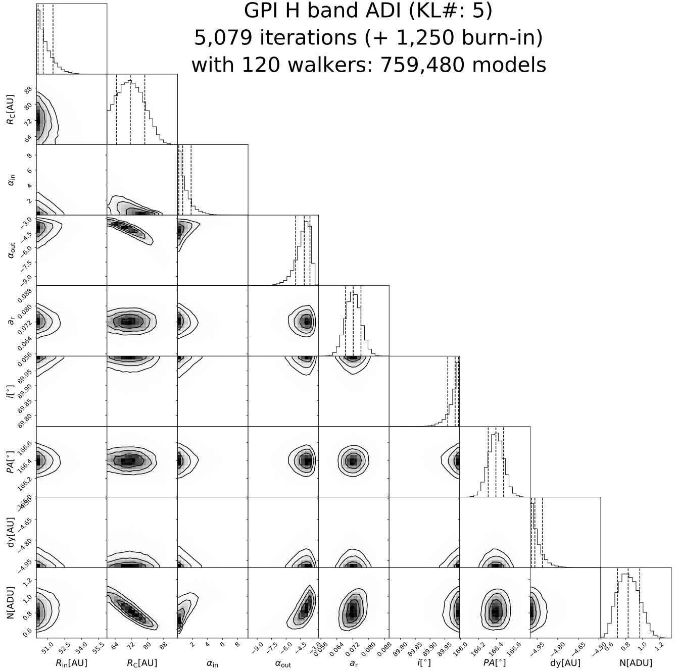
Figure A10. Posterior distribution for HD 111520 whole disk H -band models.
