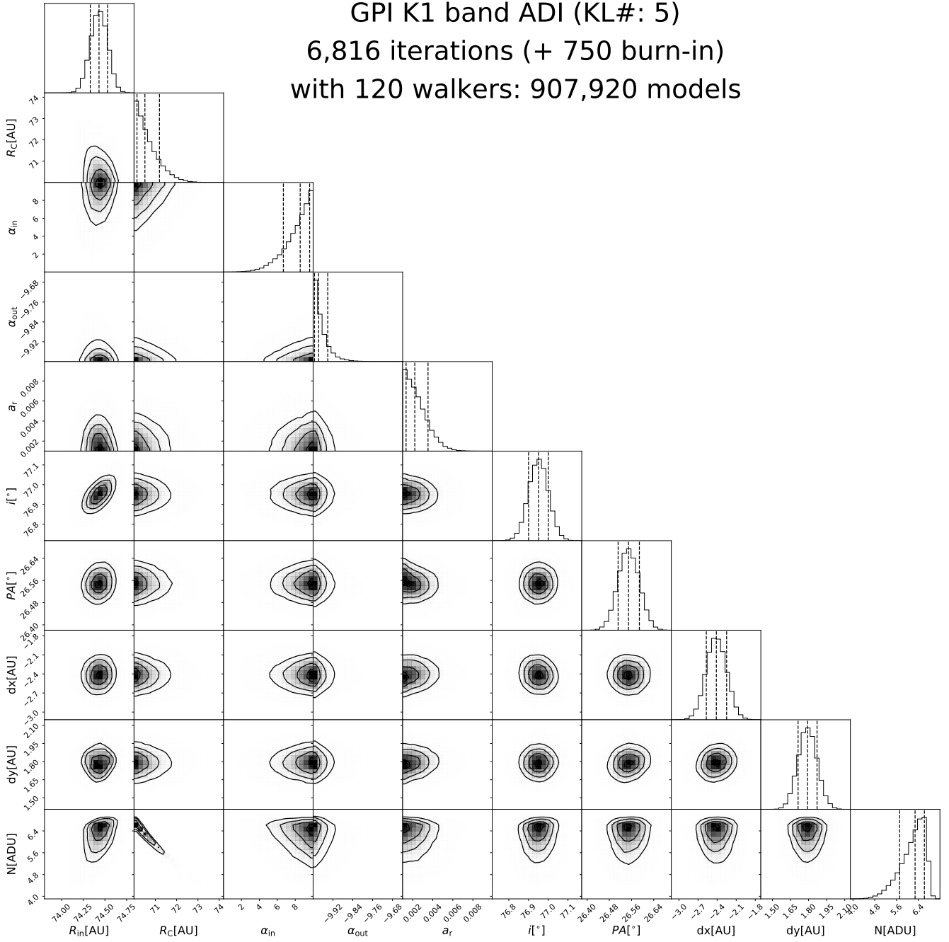
Figure A16. Posterior distribution for the Milli et al. (2017) SPF HR 4796A K1 -band models.
