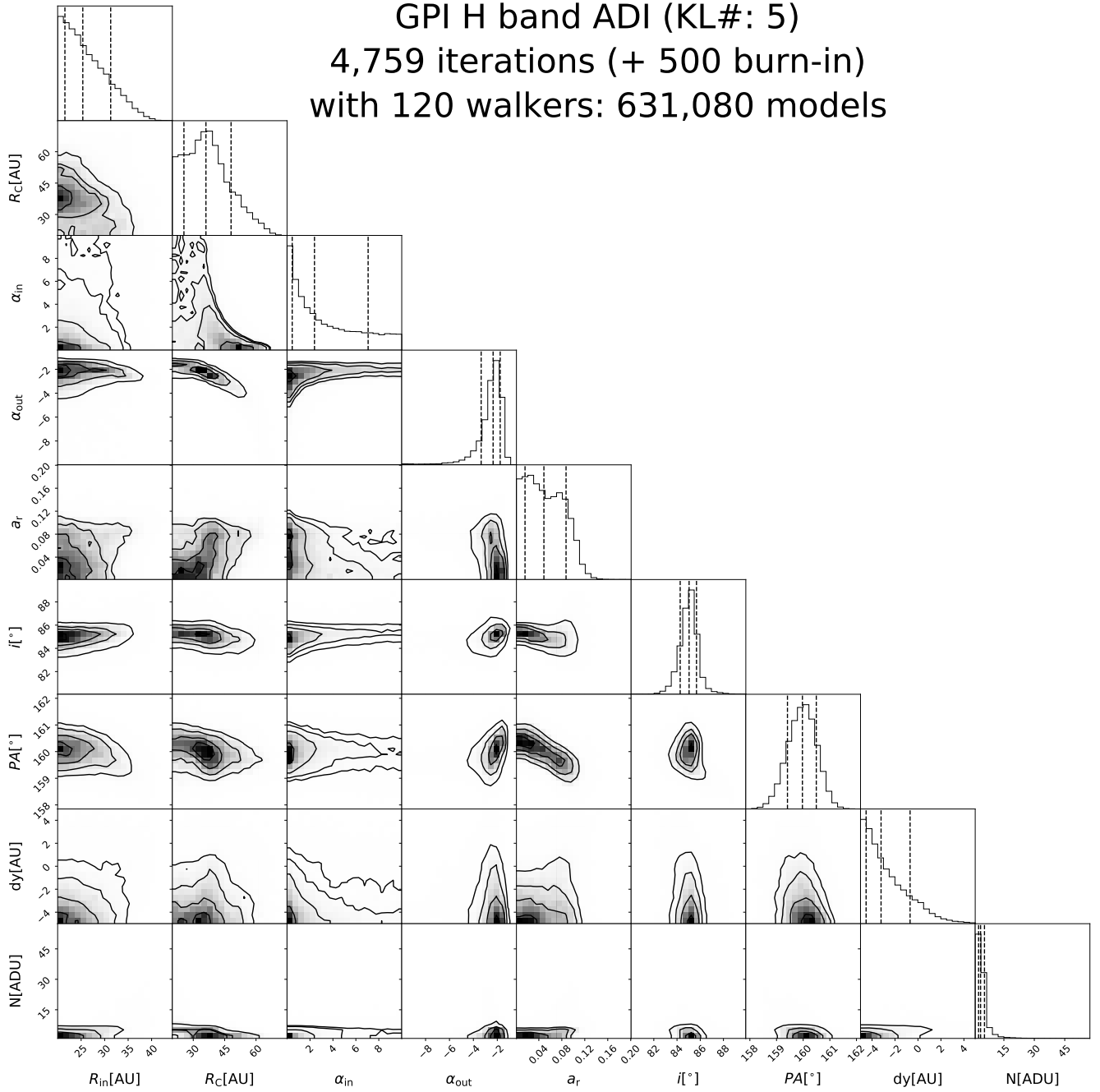
Figure A8. Posterior distribution for HD 110058 NW H -band models.
