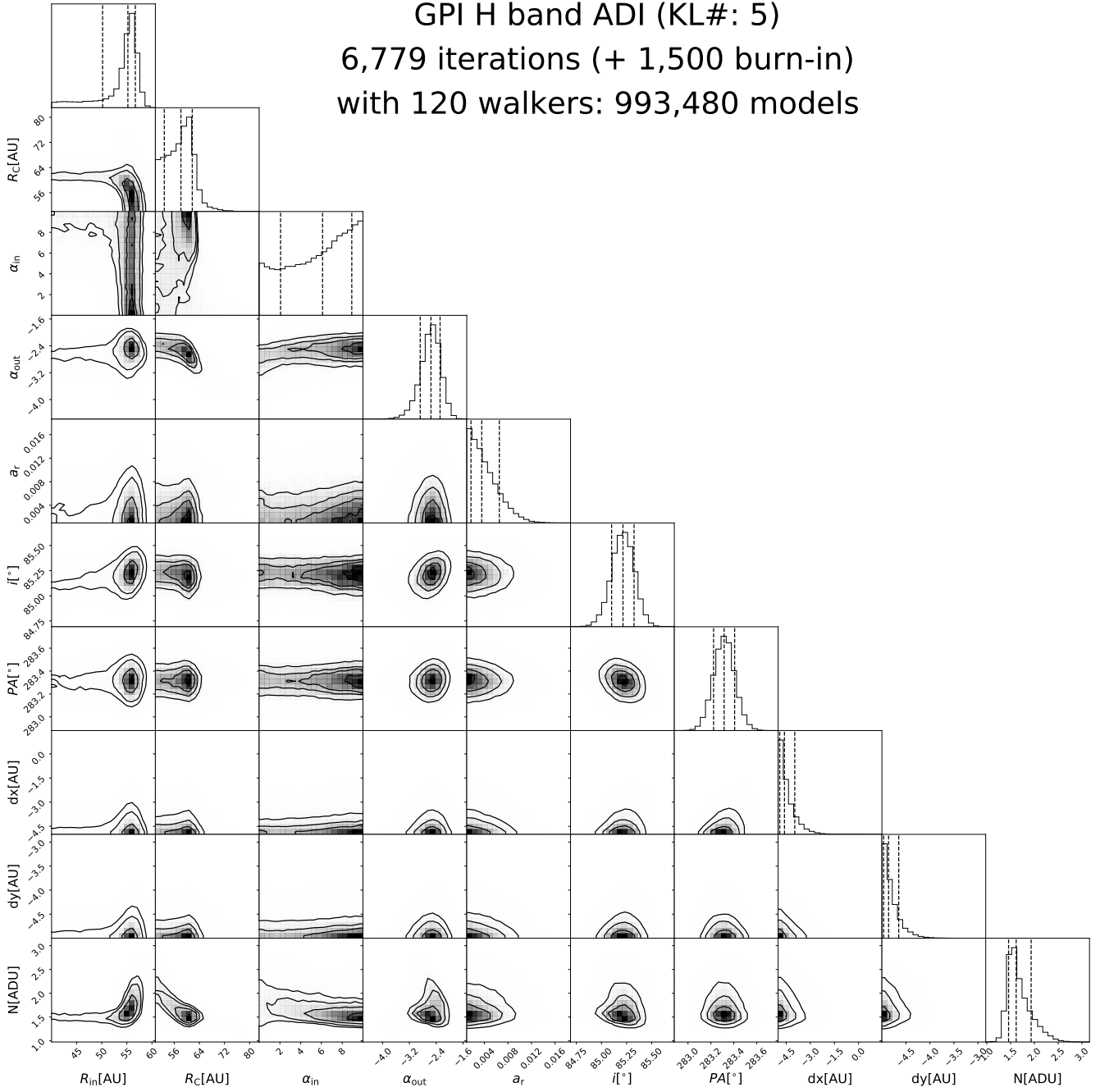
Figure A6. Posterior distribution for HD 106906 SE H -band models.
