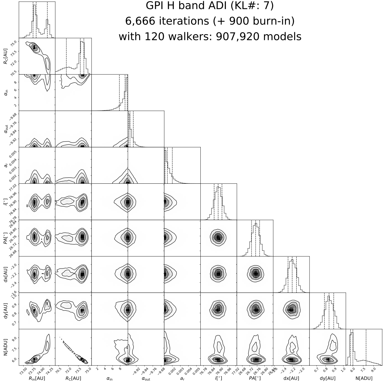
Figure A15. Posterior distribution for the Milli et al. (2017) SPF HR 4796A H -band models.
