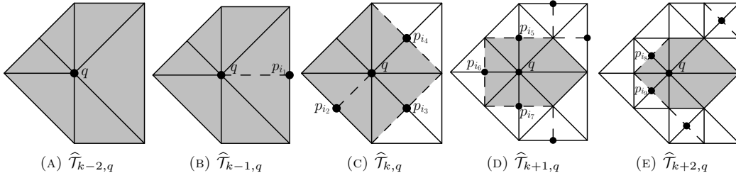
FIGURE 7.1. Local auxiliary meshes \hat{\mathcal{T}}_{j,q} with |j - k| \leq k_* = 2 . Index sets \mathcal{S}_{k-1,q} = \{i_1\} , \mathcal{S}_{k,q} = \{i_2, i_3, i_4\} , \mathcal{S}_{k+1,q} = \{i_5, i_6, i_7\} , \mathcal{S}_{k+2,q} = \{i_8, i_9\} of compatible bisections to transition from \hat{\phi}_{j-1,q} to \hat{\phi}_{j,q} . The support of \hat{\phi}_{j,q} is monotone decreasing as j increases and is plotted in grey.
