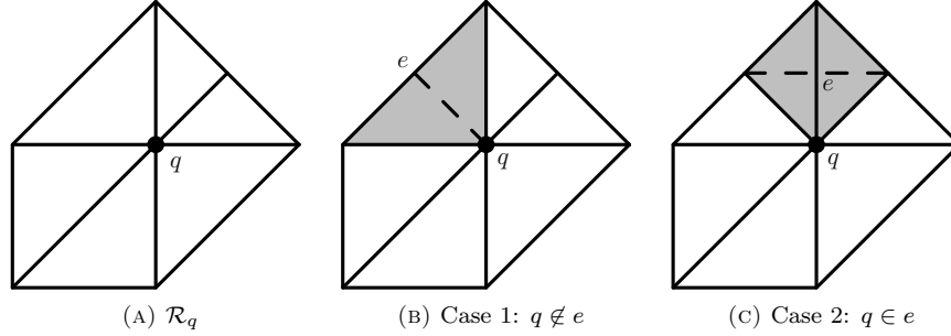
FIGURE 5.3. Two cases of bisection in \mathcal{R}_q : the bisection edge e is on the boundary of the patch and q does not belong to the bisection triplet (middle); the node q is an endpoint of e and belongs to the bisection triplet (right). The former can happen a fixed number k_* of times before the second takes place, where k_* depends on the shape regularity of \mathbb{T}(\mathcal{T}_0) .
