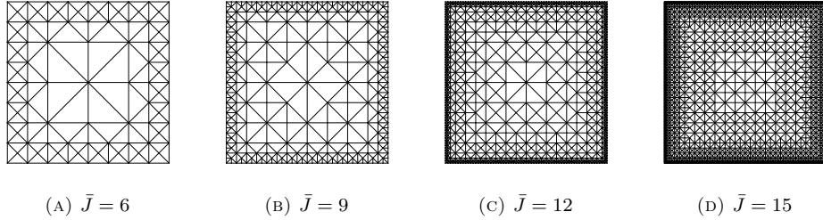
FIGURE 8.2. Graded bisection grids on (-1, 1)^2 , using strategy (8.1) with \theta = 4 and \mu = 2 .
