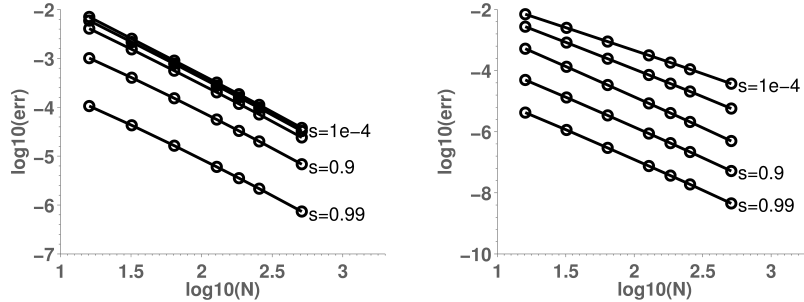
Left: errors in H_s^{2s}(-1, 1) norm of order 1.5. Right: errors in L_s^2(-1, 1) norm, orders range from 1.5 to 2.
