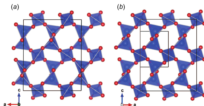
Figure 10 A comparison between two silica polymorphs, (a) moganite ( I2/a , No. 15) and (b) right-handed \alpha -quartz ( P3 2 21 , No. 154) with its unit cell converted to a monoclinic C2 (No. 5) space group. The black solid lines show unit cells, and the small rectangle in panel (b) shows the original unit cell of \alpha -quartz.
