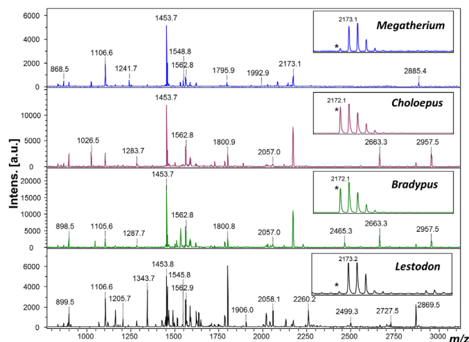
Fig 1. MALDI-ToF mass spectra of collagen extracted from Lestodon and Megatherium digested with trypsin. * Note the clearly observable difference in deamidation as a marker for protein ageing due to the presence of a glutamine residue in this peptide.
