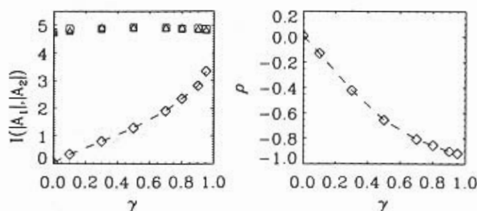
Figure 5.3: Left: Entropy of |A_1| ( \square ) and |A_2| ( \triangle ) and their mutual information I ( \diamond ) as a function of \gamma . Right: Correlation coefficient \rho of |A_1| vs |A_2| as a function of \gamma .
