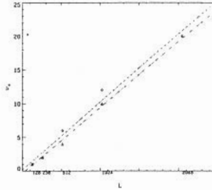
Figure 3.7: The critical winding number ( \nu_c ) as a function of the length L of the system is shown. Different symbols correspond to c_1 = 2.1 and c_2 = -0.8 ( \Delta ) and c_1 = 1.96 and c_2 = -0.83 ( \Diamond ). The straight lines are linear fits to the two sets of data.
