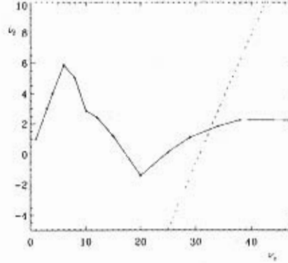
Figure 3.6: The final averaged winding number ( \bar{\nu}_f ) as a function of the initial one \nu_i . The initial condition is a TW with winding number \nu_i for c_1 = 2.1 and c_2 = -0.8 . The dashed line corresponds to the lowest of the two fastest Fourier modes of fastest growth in the linear regime as a function of \nu_i .
