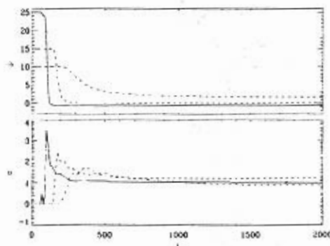
Figure 3.3: a) Temporal evolution of \bar{\nu}(t) for four different initial winding numbers \nu_i = 25 (solid), 20 (dotted), 15 (dashed) 10 (dashed-dotted). c_1 = 2.1, c_2 = -0.83 (PT regime). b) Winding number standard deviation \sigma .
