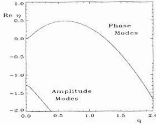
Figure 1.14: The growth rate (1.27) vs. the wave number of the modes q of the perturbation. For the set of parameter values c_1 = -0.2, c_2 = -4.0 and k = 0.6 , the "Amplitude modes" are damped, while the "Phase modes" are unstable and identify a mode of fastest growth.
