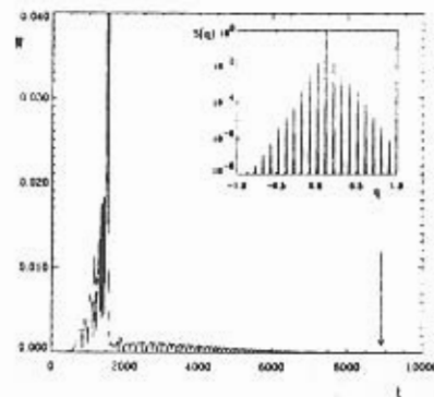
Figure 3.10: a) The time evolution of W for a quasiperiodic state. The initial condition is a TW sinusoidally perturbed for c_1 = 2.1 and c_2 = -0.6 . In the inset the spatial power spectrum S(q) as a function of wavenumber at the time t = 8900 indicated by an arrow in the main picture.
