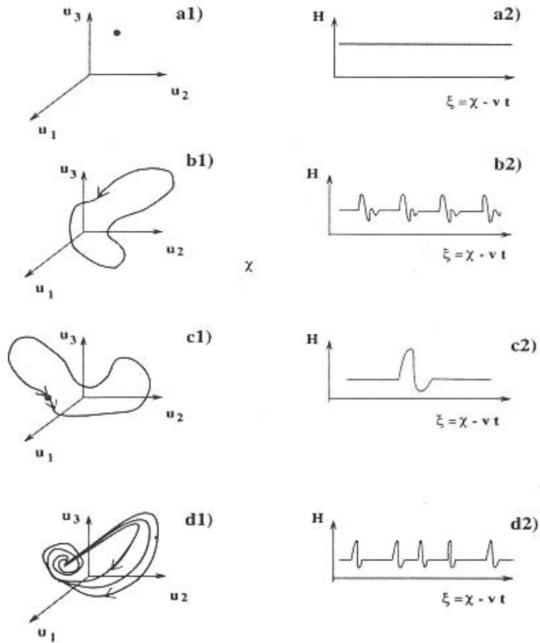
Figure 3.15: Schematic relationship between trajectories of the dynamical system (3.26) in phase space (left column) and solutions u(\chi, \tau) = H(\xi = \chi - v\tau) of equation (3.20) (right column). a1) Fixed point of (3.26), a2) uniform solution of (3.20) (traveling wave in the CGLE (3.1)). b1) Periodic solution (limit cycle) of (3.20), b2) periodic train solution of (3.20) (quasiperiodic solution of the CGLE (3.1)). c1) Homoclinic trajectory of (3.26), c2) single pulse of (3.20). d1) Chaotic trajectory of (3.26), d2) spatially irregular solution of (3.20) (frozen turbulence in the CGLE).
