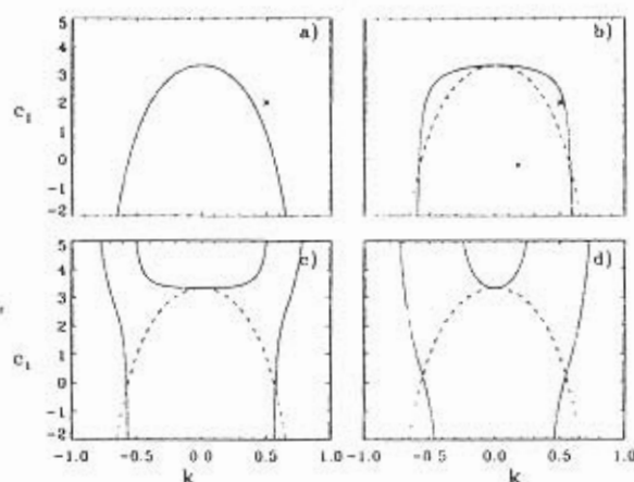
Figure 4.2: Stability region for the plane wave (4.2) for c_2 = -0.3 for a) \gamma = 0 , b) \gamma = 0.5 , c) \gamma = 0.7 , d) \gamma = 2 . For comparison, the boundary of the stability region for \gamma = 0 is shown in figs. b)-d) as a dashed line.
