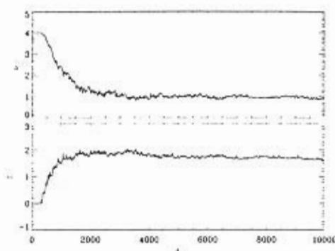
Figure 3.4: a) Temporal evolution of \bar{\nu}(t) for an initial winding numbers of \nu_i = 4 in the bichaos regime. c_1 = 1.6, c_2 = -1.0 . b) Winding number standard deviation \sigma .
