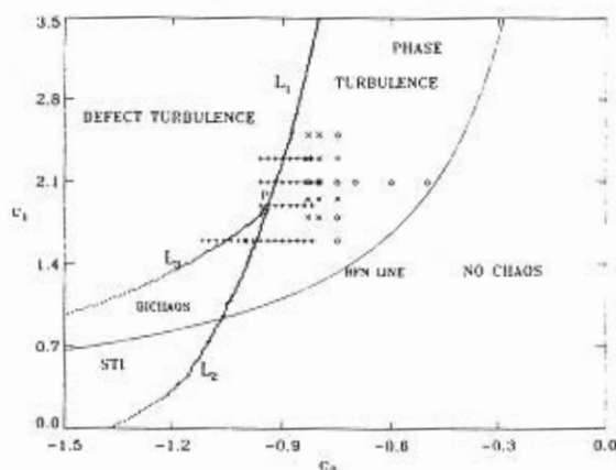
Figure 3.1: Regions of the parameter space [c_1, c_2] for the CGLE displaying different kinds of regular and chaotic behavior. Lines L_1, L_3 were determined in [165, 42, 43]. See the text for the explanation of the different points.
