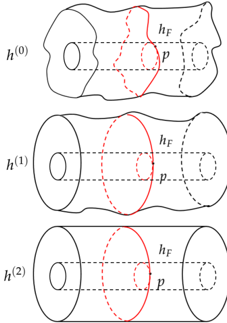
Figure 5.2: Schematic depiction of the steps involved in the proof.
