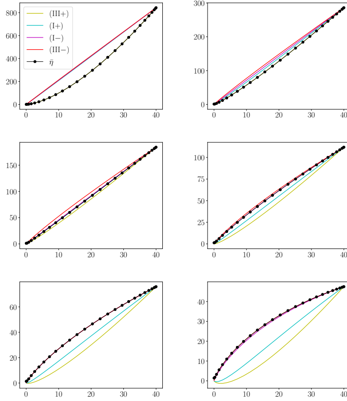
Figure 6.8: Plots of \bar{\eta} together with the fitting models (III+), (I+), (I-) and (III-) for the six solutions in Table 6.4 corresponding, from left to right, from top to bottom, to L = 8.8798, 4.8839, 4.2468, 3.7568, 3.4885, 3.2559 . The \bar{\eta} curve overlaps the best-fitting model in all cases, while some of the bad-fitting model curves overlap among themselves; that is why not all curves are visible in all plots.
