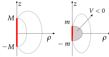
Figure 2.1: Representation of a Schwarzschild solution and a Kerr solution with the same ADM mass M , in Weyl-Papapetrou coordinates. The dashed lines represent level sets of V . Observe the reduction in the horizon coordinate length ( m < M ) and the position of the ergo-region.
