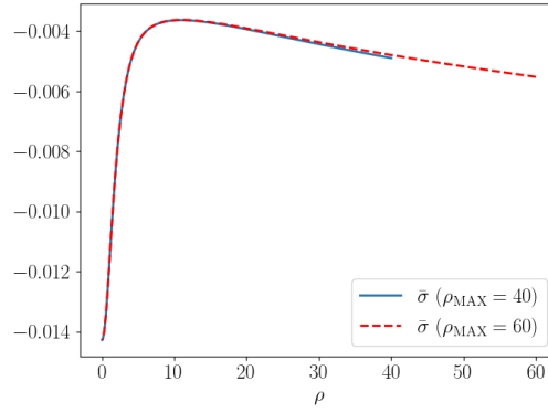
Figure 6.4: Plot of \bar{\sigma}(z = 0) when computed using two values of \rho_{\text{MAX}} for the case L = 6.9770 .
