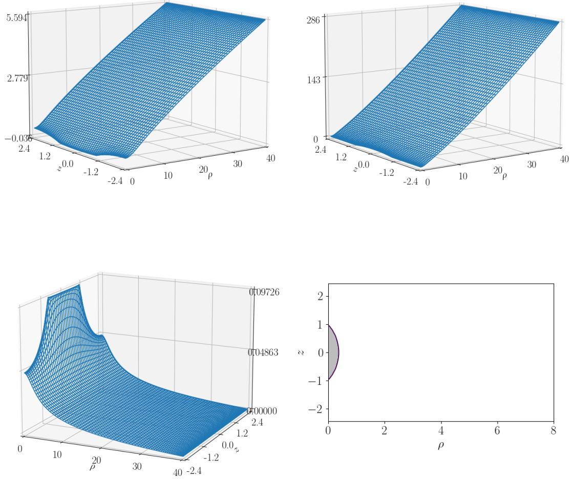
Figure 6.6: Plots of the metric functions V (top left) and \eta (top right), and plot of \Omega and the ergosphere (as a gray region) at the bottom for the solution with N_h = 40 of Table 6.1.
