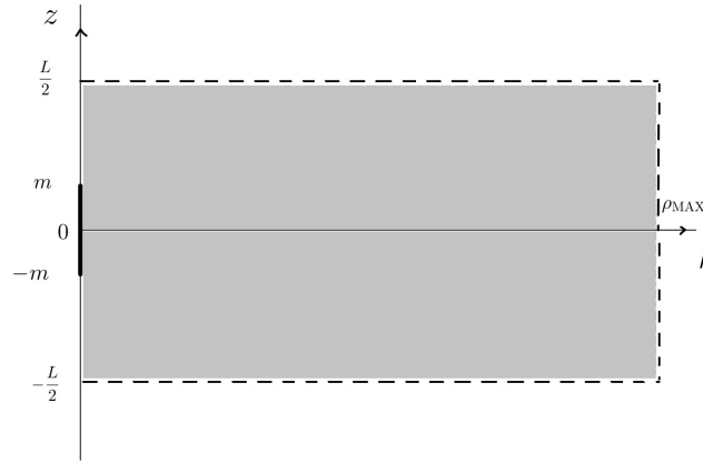
Figure 6.1: The numerical domain with the horizon indicated by the thick interval on the z -axis.
