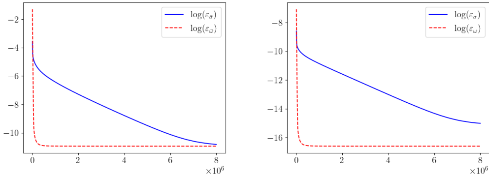
Figure 6.3: Convergence of the parabolic flow to stationary state as a function of time steps for the solution with N_h = 40 in Table 6.1.
