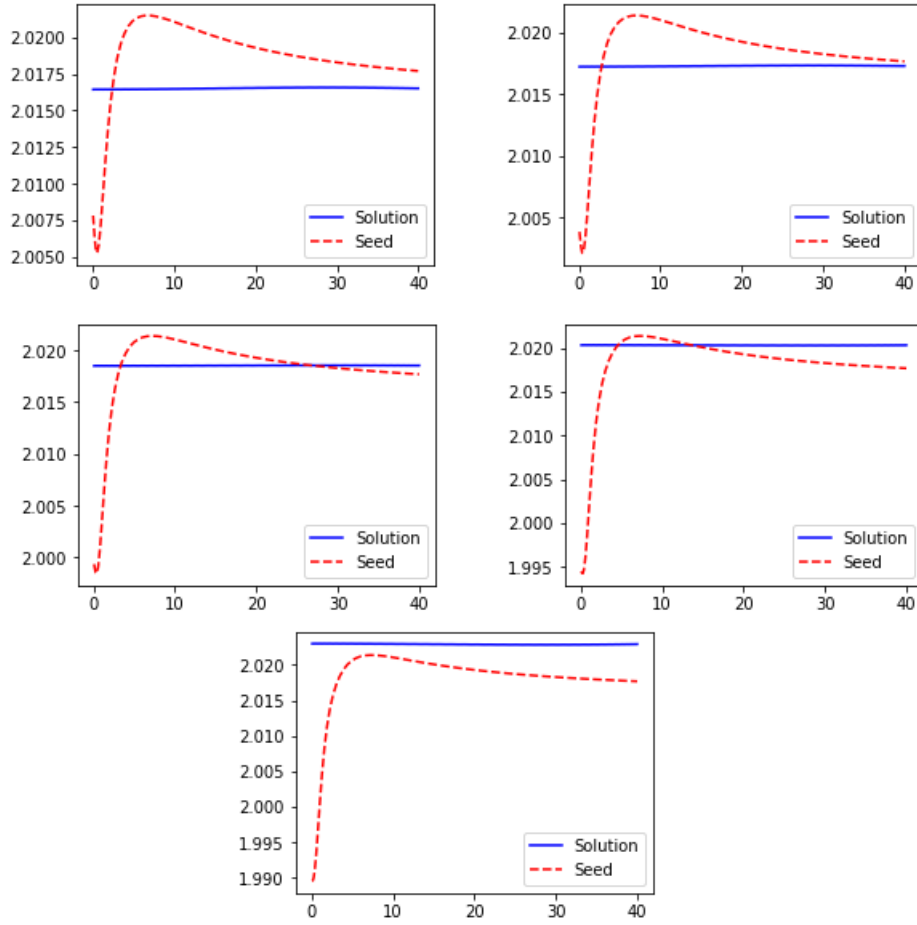
Figure 6.12: Plots of M(\rho) for the seed and for the numerically computed solution compared for five runs in the series. From left to right, from top to bottom, the plots correspond to the cases with L = 13.9539, 11.4915, 9.7677, 8.4937, 7.5136 .
