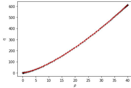
Figure 6.13: Plot of the best fitting Kasner-like asymptotic behavior for L = 13.9539 . The Kasner exponent is given in Table 6.6 .
