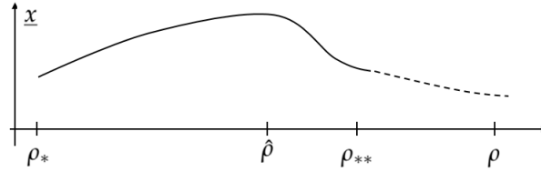
Figure 4.1: Schematic representation of \underline{x} decreasing after \hat{\rho} .
