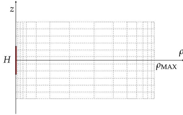
Figure 6.2: Schematic representation of the \rho - z grid defined. Observe that the poles H \cap \mathcal{A} are in the middle of two consecutive grid points.
