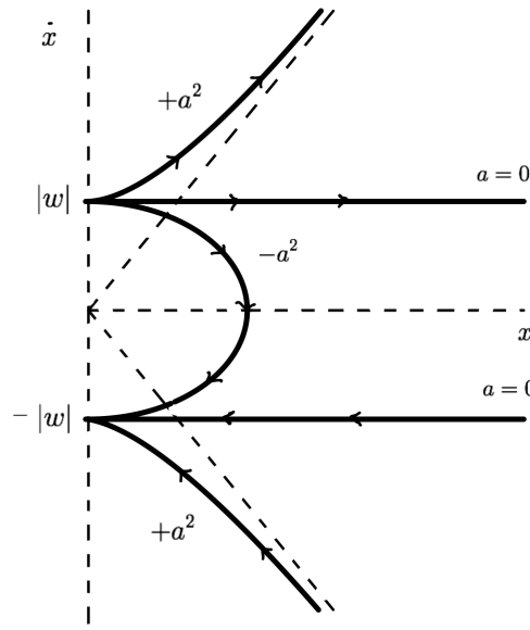
Figure 3.1: Types of U -orbits in phase space (U, \dot{U}) . Those of physical interest are the ones on top \epsilon = 1 and a = 0 .
