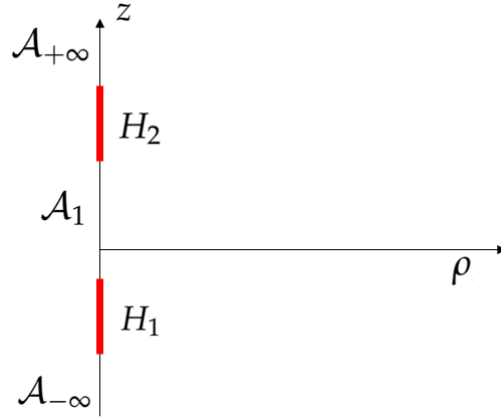
Figure 2.2: Example showing the case where H := \mathcal{H} \cap \mathcal{N} has two connected components, H_1 and H_2 , and the axis has three connected components: \mathcal{A}_{-\infty} and \mathcal{A}_{+\infty} are unbounded, while \mathcal{A}_1 is bounded.
