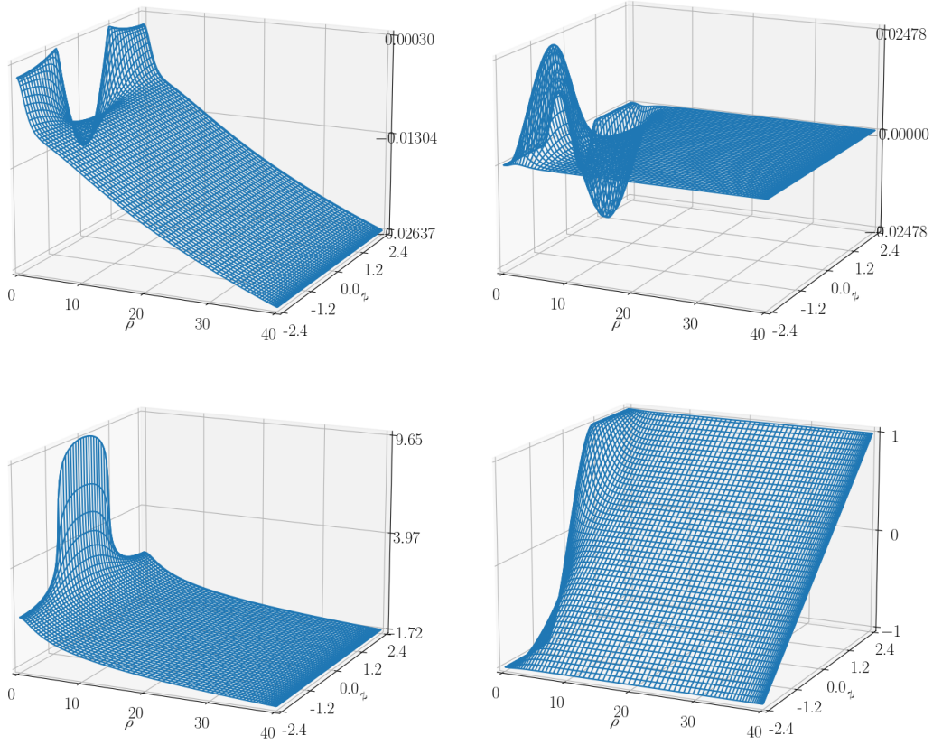
Figure 6.5: Plots of the solution corresponding to L = 4.8839 of Table 6.1. From left to right, from top to bottom: \bar{\sigma} , \bar{\omega} , \sigma , \omega .
