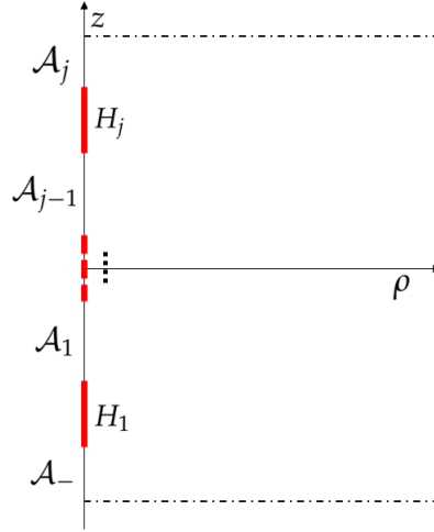
Figure 6.10: Schematic representation of a multi-horizon set-up, for j horizons. The data is either z -odd or z -even.
