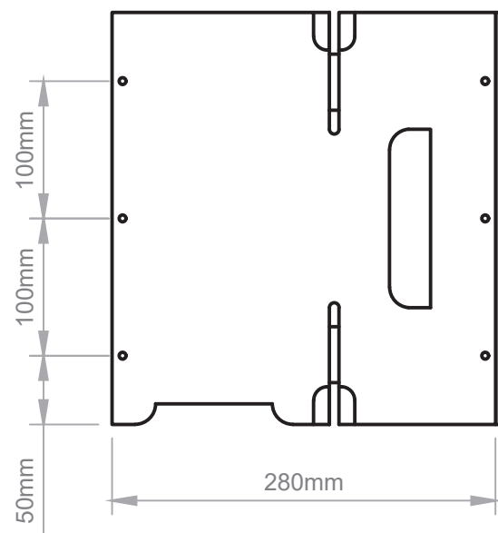
Vista Frontal
