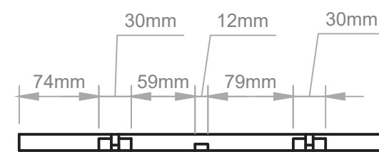
Vista Frontal
