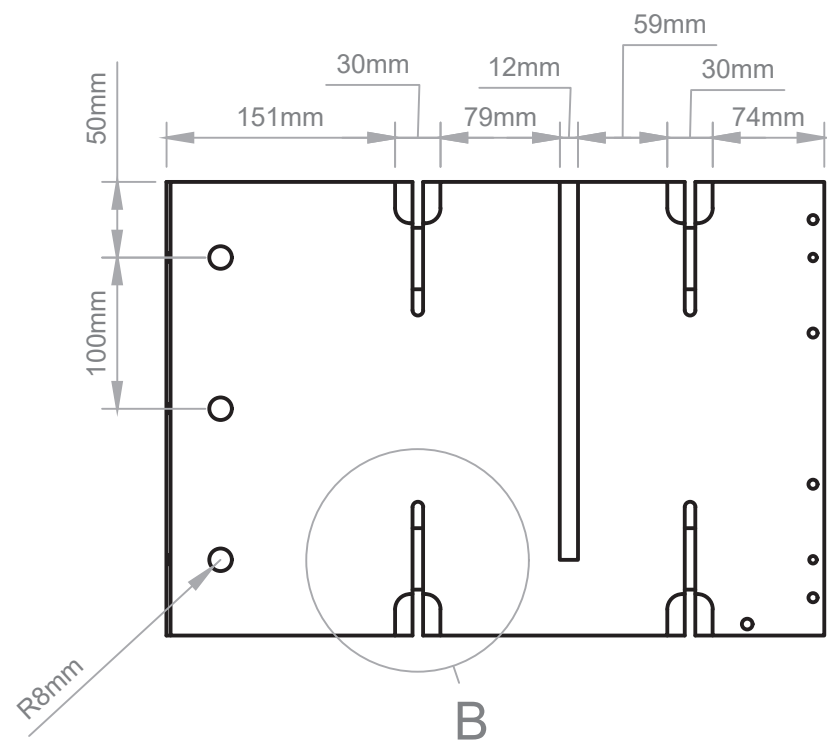
Vista Frontal
