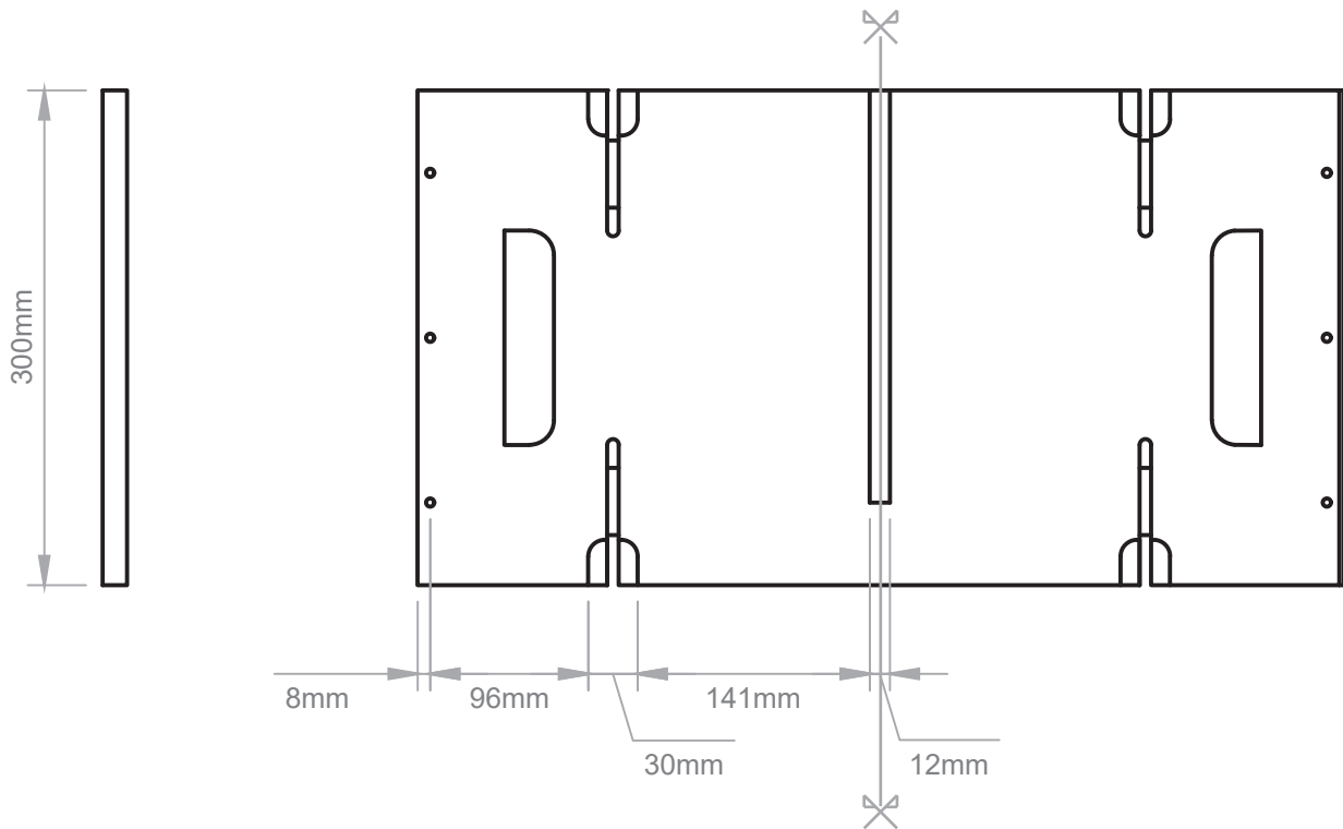
Vista Frontal
