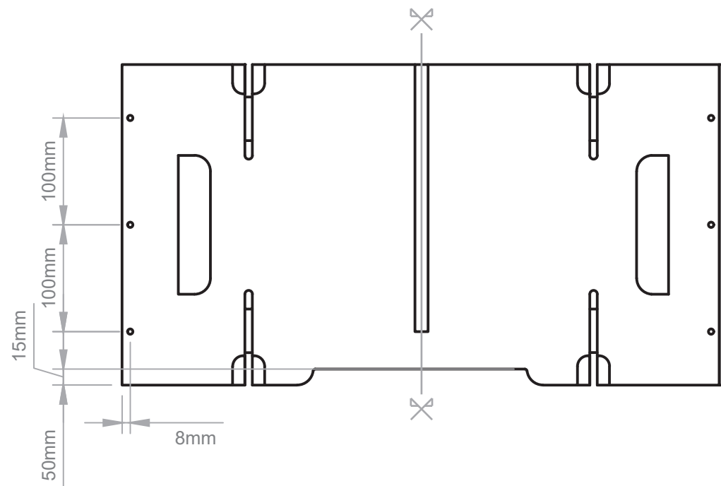
Vista Frontal
