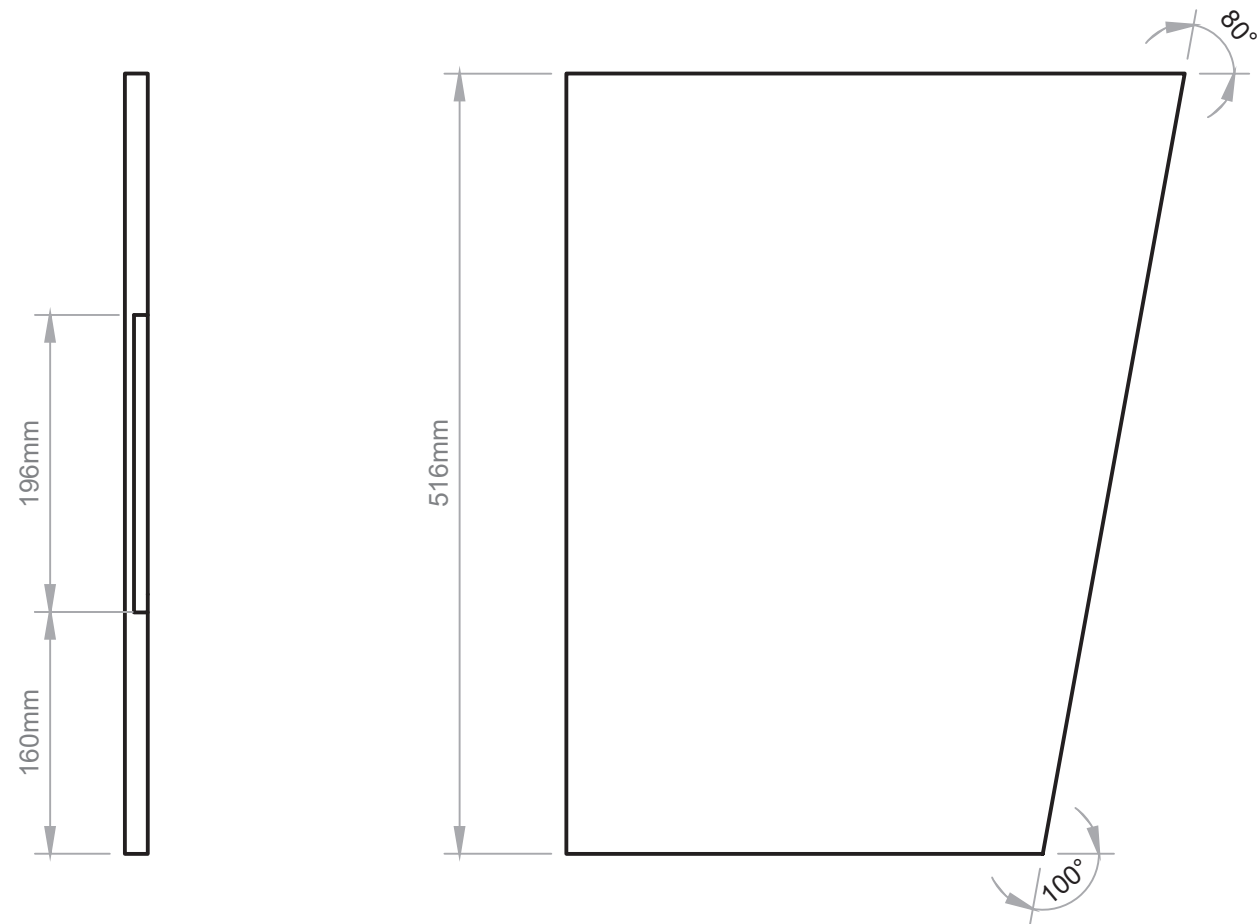
Vista Frontal
