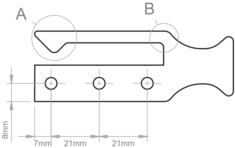
Vista Frontal
