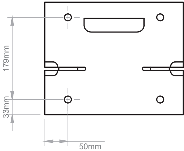
Vista Frontal
