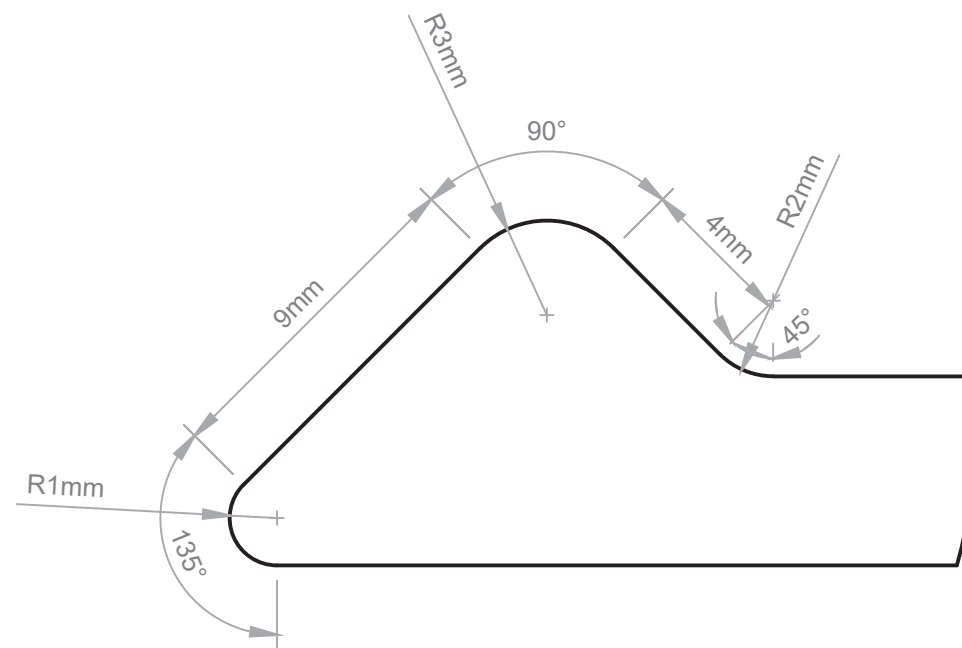
A (5:1)
