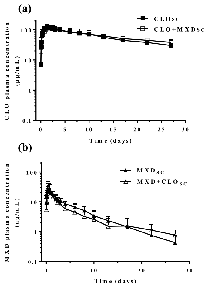
Fig. 1. Comparative mean ( \pm SD) (a) closantel (CLO, 5 mg/kg) and (b) moxidectin (MXD, 0.2 mg/kg) plasma concentration profiles obtained after its subcutaneous administration either alone or co-administered to parasitized lambs.
