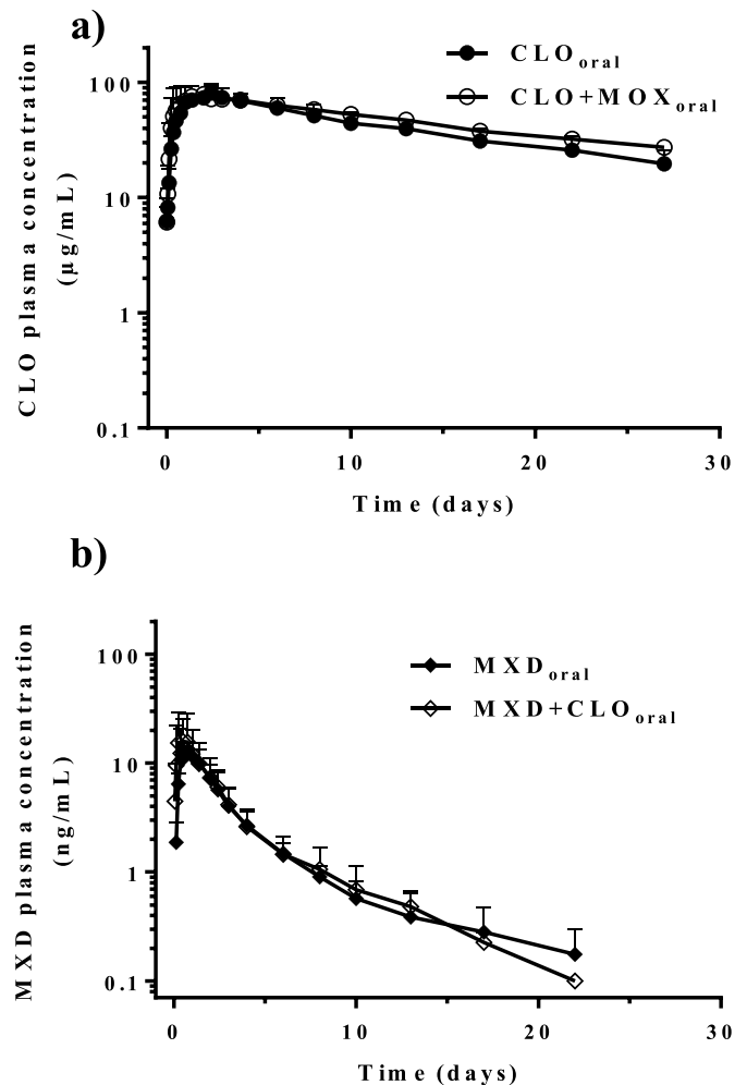
Fig. 2. Comparative mean ( \pm SD) (a) closantel (CLO, 10 mg/kg) and (b) moxidectin (MXD, 0.2 mg/kg) plasma concentration profiles obtained after its oral administration either alone or co-administered to parasitized lambs.
