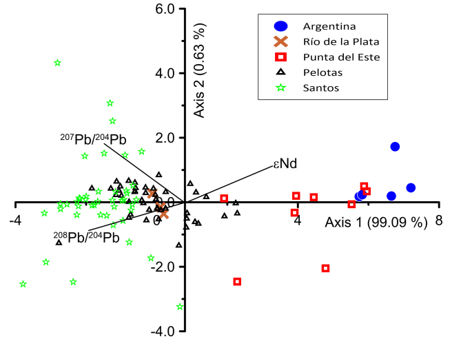
Figure 4. Scatter plot of the samples according to the first two axes generated from the discriminant analysis.
