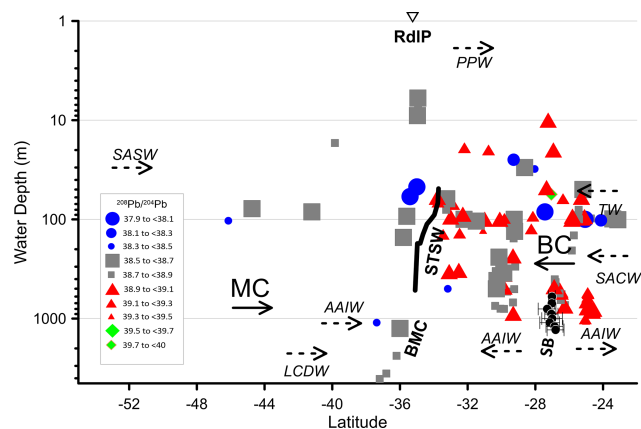
Figure 9. Latitudinal and bathymetric variability of ^{208}\text{Pb}/^{204}\text{Pb} in the sector between 23 and 55° S. Río de la Plata (RdIP). Water masses: Plata Plume Water (PPW), Subantarctic Shelf Water (SASW), Tropical Water (TW), South Atlantic Central Water (SACW), Antarctic Intermediate Water (AAIW), and Lower Circumpolar Deep Water (LCDW). Currents: Malvinas Current (MC) and Brazil Current (BC). Fronts: Subtropical Shelf Front (STSW), Brazil–Malvinas Confluence (BMC), and Santos Bifurcation (SB). Vertical axis in \log_{10} scale.
