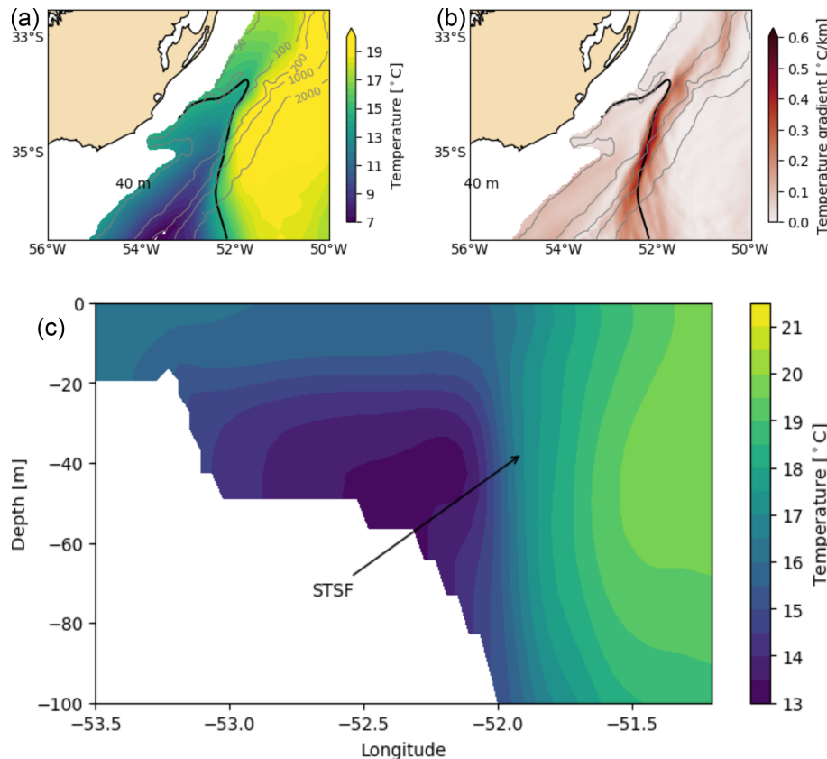
Figure 6. Graphical outputs of the LLC2160 focused on the Subtropical Shelf Front. (a) Variations of temperature in the zone of the front. (b) Temperature gradient; the front is recognized as the zone of maximum gradient (darker colors). (c) Vertical transect at 35° S showing the location of the Subtropical Shelf Front (STSF) as the gradient of the Subantarctic Shelf Water (deep blue) and the Subtropical Shelf Water (light green).
