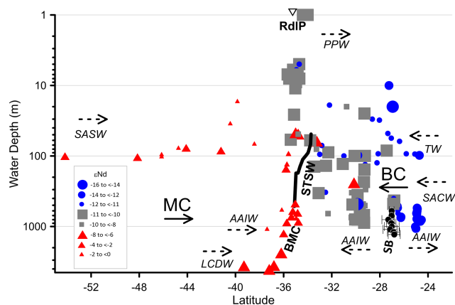
Figure 7. Latitudinal and bathymetric variability of \epsilon\text{Nd} in the sector between 23 and 55° S. Water masses: Plata Plume Water (PPW), Subantarctic Shelf Water (SASW), Tropical Water (TW), South Atlantic Central Water (SACW), Antarctic Intermediate Water (AAIW), and Lower Circumpolar Deep Water (LCDW). Currents: Malvinas Current (MC) and Brazil Current (BC). Fronts: Subtropical Shelf Front (STSW), Brazil–Malvinas Confluence (BMC), and Santos Bifurcation (SB). Vertical axis in \log_{10} scale.
