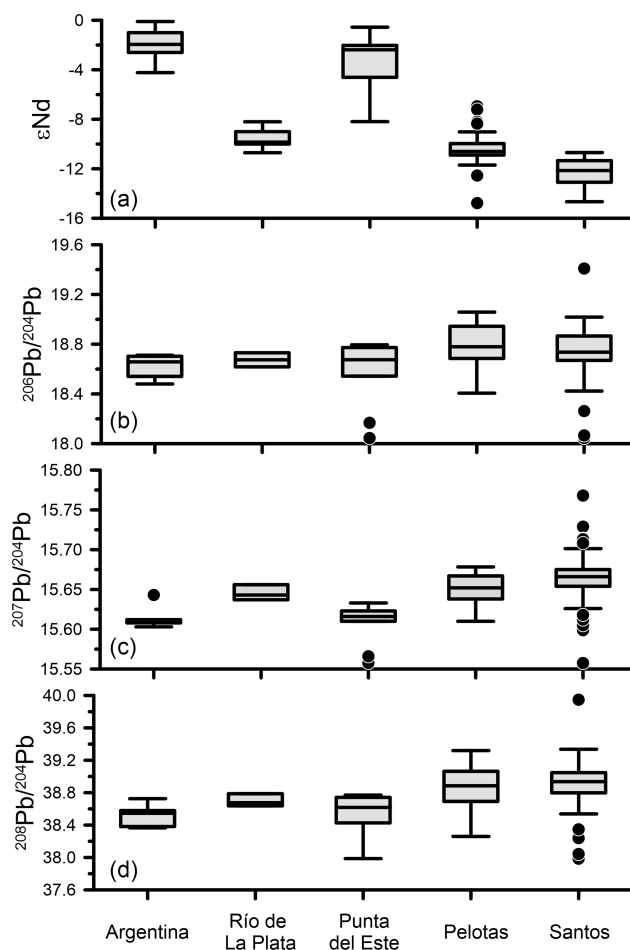
Figure 2. Box plots of the distributions of (a) \epsilon\text{Nd} , (b) ^{206}\text{Pb}/^{204}\text{Pb} , (c) ^{207}\text{Pb}/^{204}\text{Pb} , and (d) ^{208}\text{Pb}/^{204}\text{Pb} . Outliers are shown as dots.
