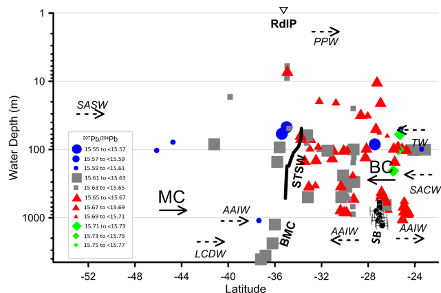
Figure 8. Latitudinal and bathymetric variability of ^{207}\text{Pb}/^{204}\text{Pb} in the sector between 23 and 55° S. Río de la Plata (RdIP). Water masses: Plata Plume Water (PPW), Subantarctic Shelf Water (SASW), Tropical Water (TW), South Atlantic Central Water (SACW), Antarctic Intermediate Water (AAIW), and Lower Circumpolar Deep Water (LCDW). Currents: Malvinas Current (MC) and Brazil Current (BC). Fronts: Subtropical Shelf Front (STSW), Brazil–Malvinas Confluence (BMC), and Santos Bifurcation (SB). Vertical axis in \log_{10} scale.
