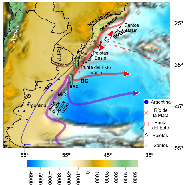
Figure 1. Location of the study area, displaying the main flows, oceanographic boundaries, and sampling stations. Thick violet line: Malvinas Current (MC); thin blue line: Subantarctic Shelf Water (SASW); thin brown line: Río de la Plata Plume (RdPP); thick red line: Brazil Current (BC); shaded rectangles: Subtropical Shelf Front (STSF) and Brazil–Malvinas Confluence (BMC); dashed red line: Santos Bifurcation (SB) and Intermediate Western Boundary Current (IWBC). Other abbreviations: Antarctic Intermediate Water (AAIW), Upper Circumpolar Deep Water (UCDW), North Atlantic Deep Water (NADW), and Lower Circumpolar Deep Water (LCDW). Bottom scale: topography in meters.
