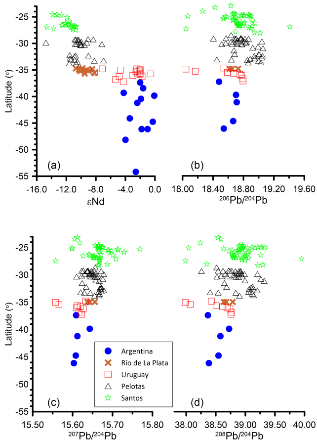
Figure 3. Latitudinal variations of (a) \epsilon\text{Nd} , (b) ^{206}\text{Pb}/^{204}\text{Pb} , (c) ^{207}\text{Pb}/^{204}\text{Pb} , and (d) ^{208}\text{Pb}/^{204}\text{Pb} .
