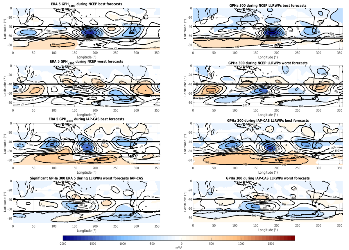
Fig 31. Anomalies of Z_{300} fields from T_d - T_{d+10} , being T_d the dates when we obtained the best/worst forecast in the NCEP and IAP-CAS models. Left (right) Figs show the anomalies of Z_{300} field obtained using the reanalysis (forecast) data. Orange (blue) areas signal positive (negative) anomalies.
