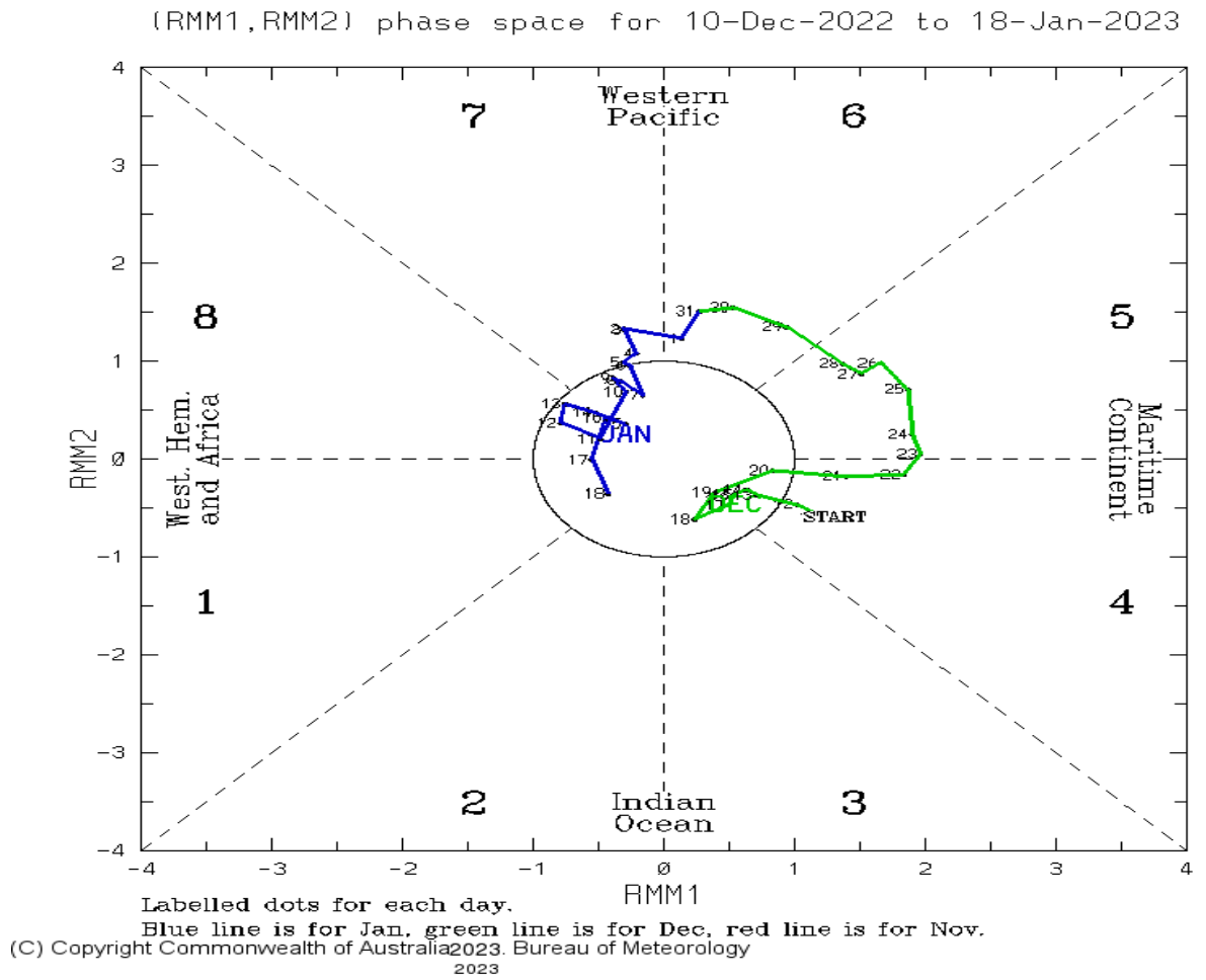
Fig 10. Propagation of the MJO between middle December 2022 to middle January 2023. Green (blue) line signals the propagation of the MJO in the month of December (January). When the MJO is within the centre circle of the Fig, the MJO is inactive or in its neutral phase (source: http://www.bom.gov.au/climate/mjo/ ).
