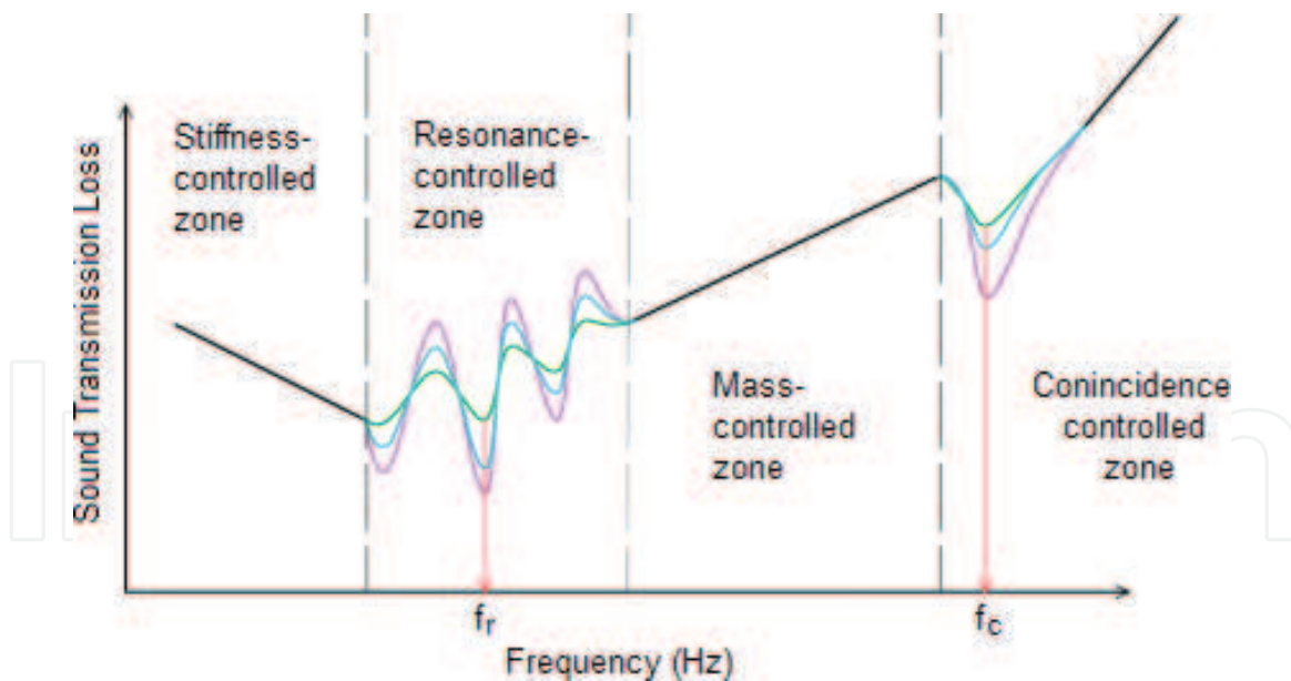
Figure 7. Acoustic performance of a simple homogeneous wall (adapted from [7]).
