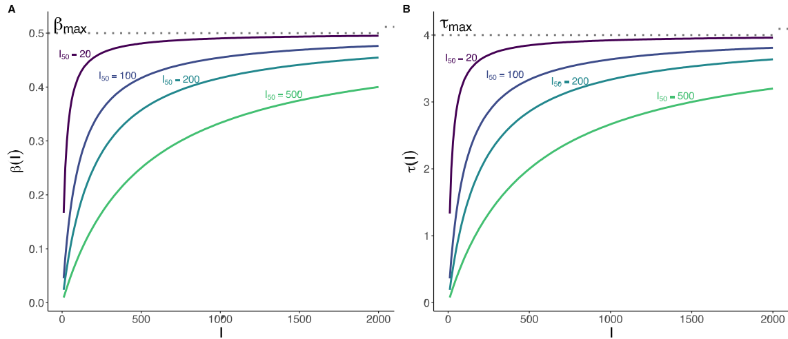
Fig. A1. Relationship between transmission rate b(I) and infection period S(I) with the number of infected individuals I , following the saturating functions b_t(I) = b_0 + (b_{\max} - b_0) \cdot I(t) / (I_{50,b} + I(t)) and S_t(I) = S_0 + (S_{\max} - S_0) \cdot I(t) / (I_{50,S} + I(t)) respectively. The parameters I_{50,b} and I_{50,S} are the number of infection numbers at which transmission rate and infection period attain half of its maximum values b_{\max} and S_{\max} . b_0 and S_0 represent the smaller transmission rate and infection period, which are attained at the lower level of infection. The saturation parameters I_{50,b} and I_{50,S} summarize the different components of the tracing strategy: the better performance of a tracing system is, the larger the I_{50,b} and I_{50,S} values will be. In this example, b_0 = S_0 = 0 , b_{\max} = 0.5 and S_{\max} = 4 .
