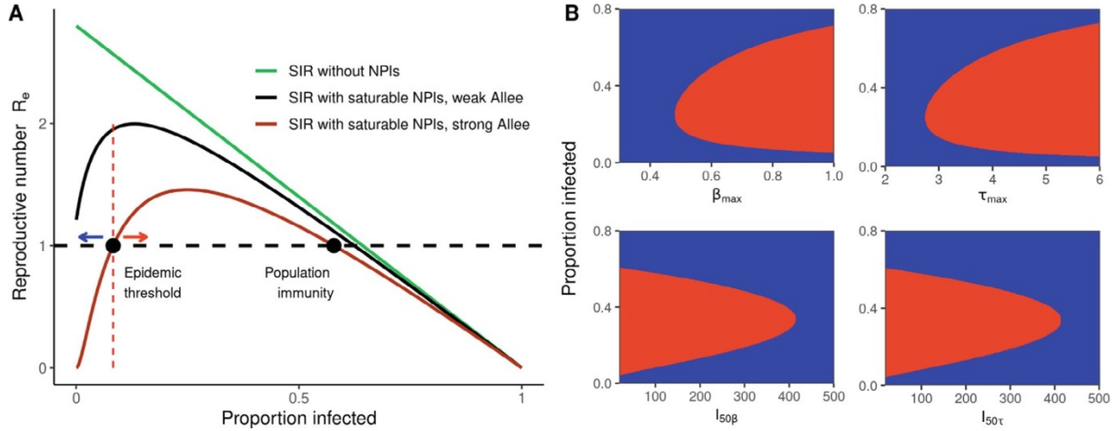
Fig. 2. Saturation processes and disease dynamics. These results are similar to those presented in Fig. 1 but obtained from a general SIR model with a rise in transmission rate (b) and infectious period (S) with I. (A) Effective reproduction number as a function of the proportion of the population infected R_e(I) . For the green line (SIR without NPIs), b was fixed to b_{\max} and S was fixed to S_{\max} . For the red line (model with saturable NPIs inducing strong Allee effect), the model parameters were: b_{\max} = 0.7 , S_{\max} = 4 , I_{50,b} = 100 , I_{50,S} = 100 , and b_0 = S_0 = 0 . For the black line (model with saturable NPIs inducing a weak Allee effect), the same parameters as for the red line were used, except for the modifications of b_0 = 0.4 and S_0 = 3 . Arrows highlight the expected trend in infection numbers around the infection threshold. (B) The alternative epidemic states of growth ( R_e(I) > 1 , red) or containment ( R_e(I) < 1 , blue) are determined by both the proportion of the infected population (vertical axis) and the transmission and infectious period parameters. These parameters capture the saturation in contact tracing with the rise in infection number ( I_{50,b} , I_{50,S} ) and the strength of other NPIs ( b_{\max} , S_{\max} ). Parameters used were the same as for the strong Allee effect in panel A, with exception of the parameter varied in the horizontal axis.
