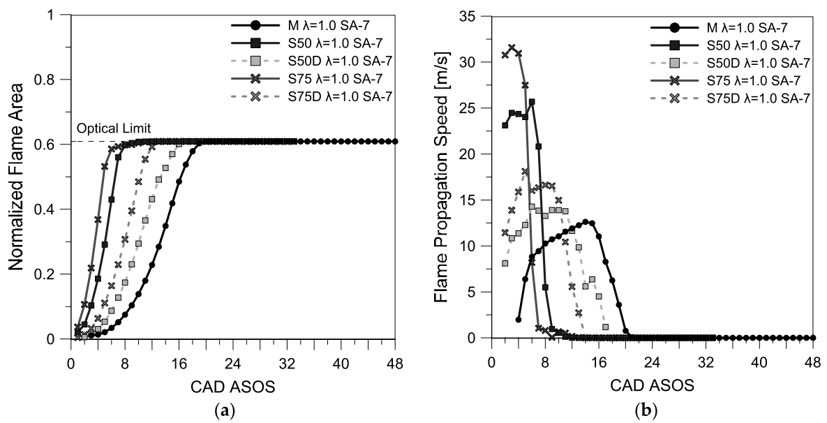
Figure 14. Average flame front evolution in terms of normalized area (cross-section piston area) and flame propagation speed for stoichiometric air-fuel ratio and five different fuels.
