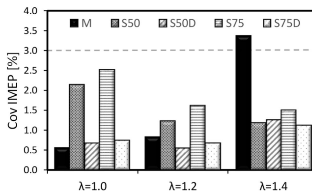
Figure 8. Coefficient of variation of indicated mean effective pressure for M, S50, S50D, and S75D at fixed SA ( -7 CAD ATDC) and air-fuel dilution from 1.0 to 1.4.
