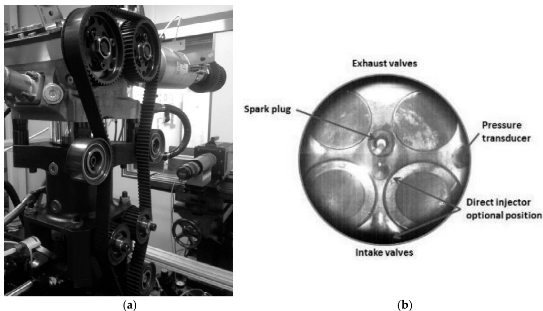
Figure 1. (a) Experimental setup of the single cylinder PFI-SI research engine with an optical arrangement (camera and intensifier), and (b) cylinder head bottom view.
