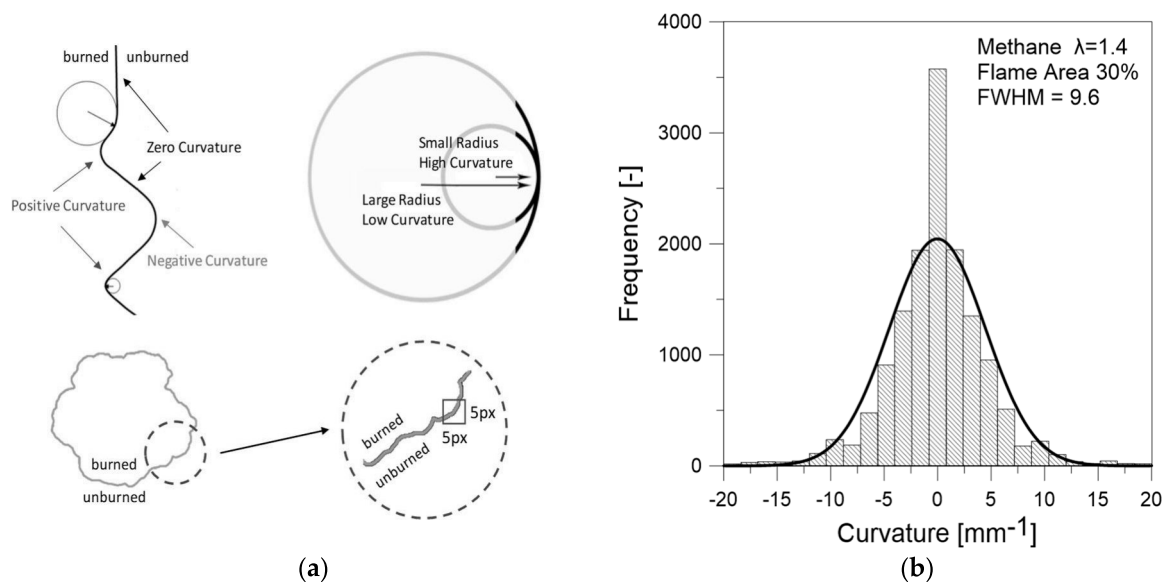
Figure 4. (a) Schematic representation of the procedure used for measuring flame curvature, and (b) histogram representative of the curvature frequency distribution and related Gaussian fitting curve evaluated for methane in baseline conditions.
