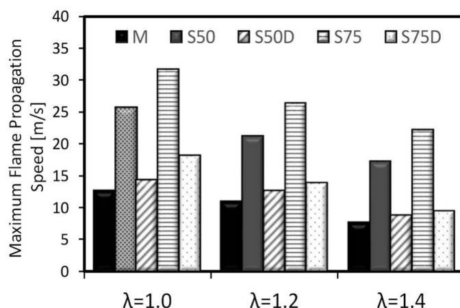
Figure 17. Maximum flame propagation speed obtained from average propagation speed data for all fuels and air-fuel ratios.
