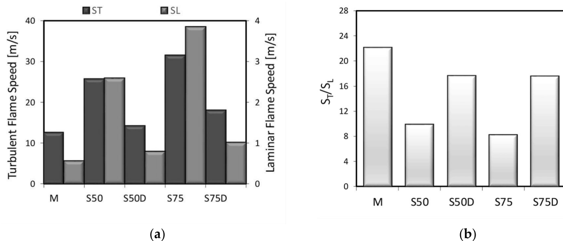
Figure 18. (a) Measured turbulent flame speed and calculated laminar flame speed and (b) the ratio between turbulent and laminar flame speed for the five different fuels at \lambda = 1.0 and engine like condition.
