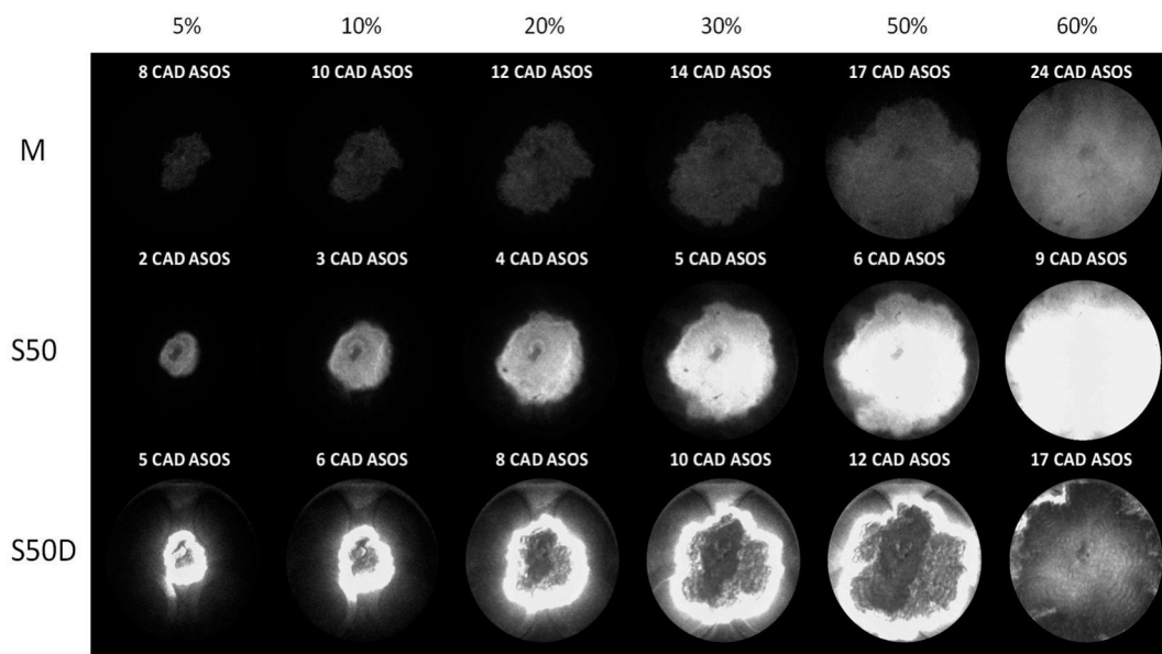
Figure 10. Image sequence of flame evolution at the same flame area (5%, 10%, 20%, 30%, 50% and 60% of the piston cross-section) for a stoichiometric air-fuel ratio ( \lambda = 1.0 ) with M, S50, and S50D fuelling.
