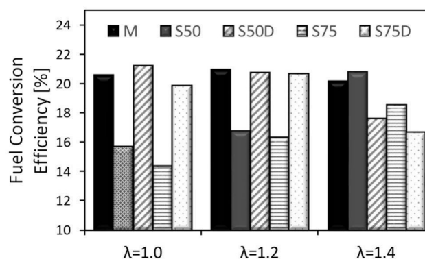
Figure 9. Fuel conversion efficiency average for M, S50, S50D and S75D at fixed SA ( -7 CAD ATDC) and air-fuel dilution from 1.0 to 1.4.
