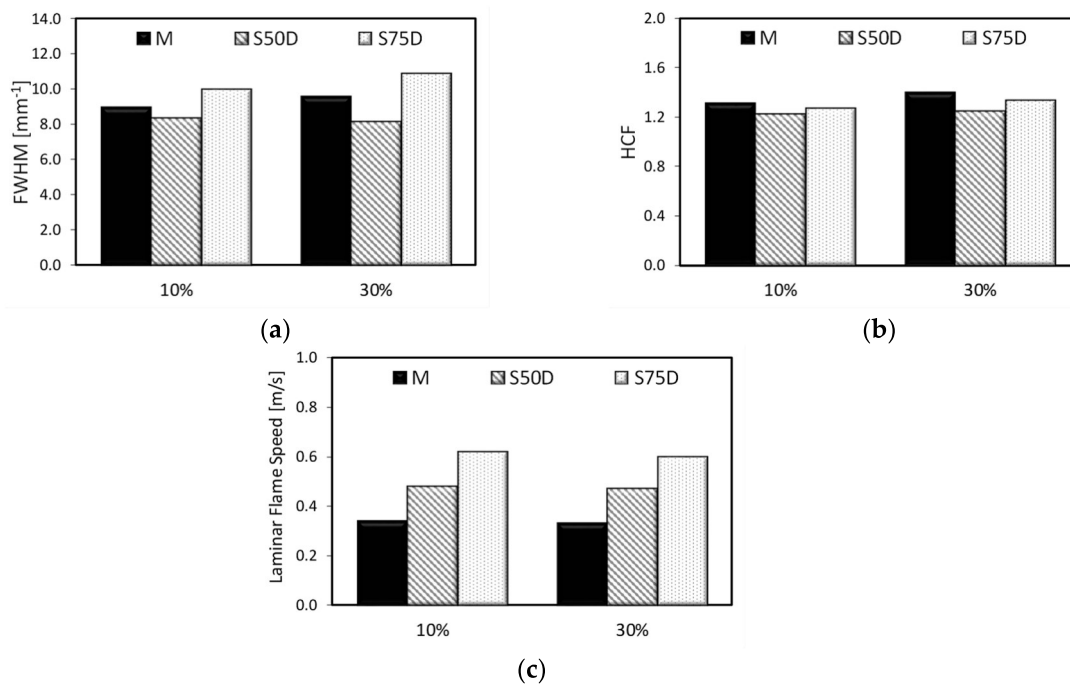
Figure 21. (a) Flame curvature, (b) average Heywood Circularity Factor, and (c) laminar flame speed in engine-like conditions for methane and real syngas mixtures at 10% and 30% flame sizes with respect to the piston area, during lean fueling ( \lambda = 1.4 ).
