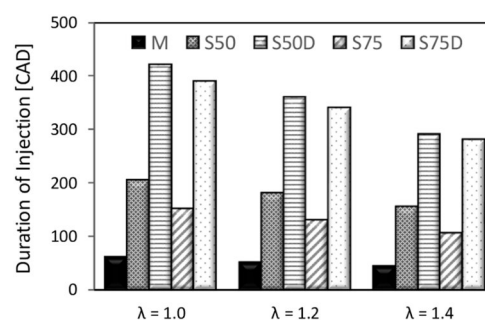
Figure 2. Duration of injection used for obtaining the different relative air-fuel ratio at 900 RPM, with SA -7 CAD ATDC and WOT.
