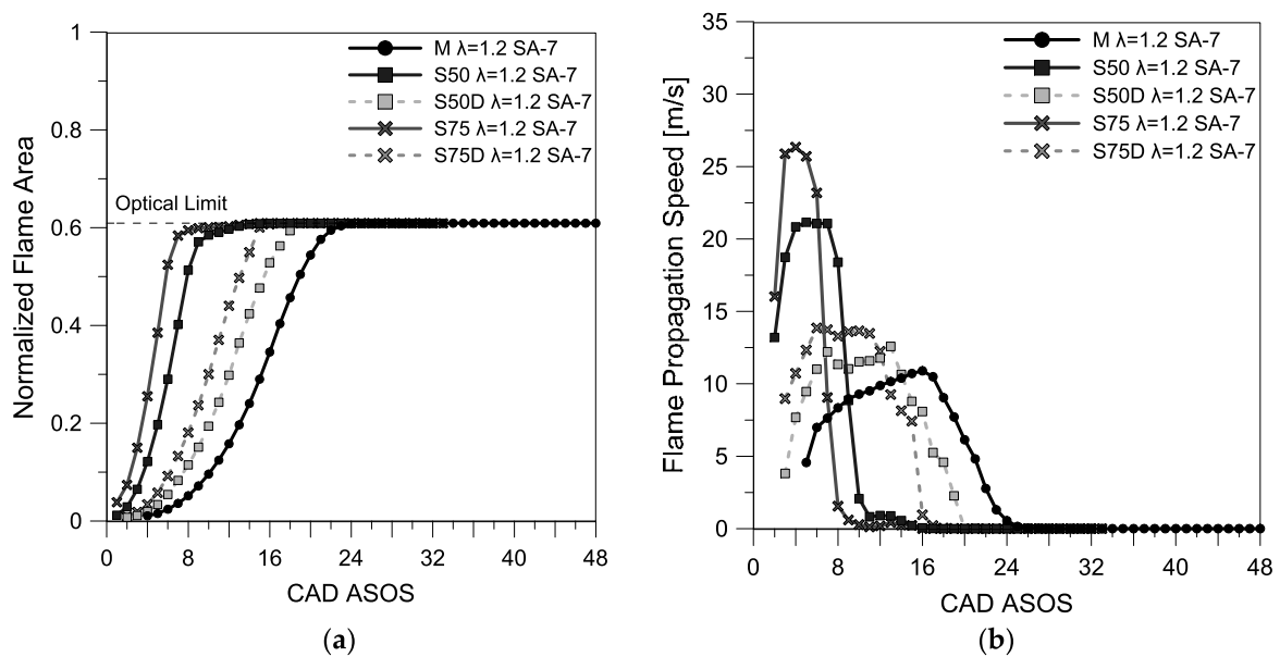
Figure 15. Average flame front evolution in terms of normalized area (cross-section piston area) and flame propagation speed for intermediate lean air-fuel ratio and five different fuels.
