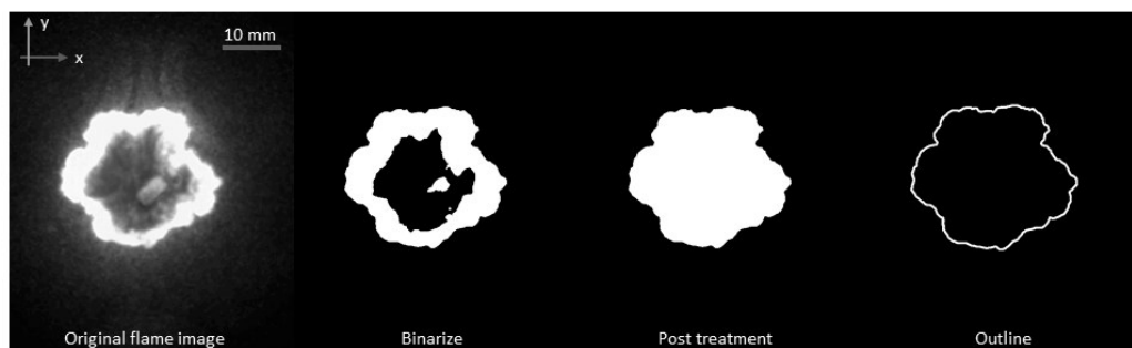
Figure 3. Sketch of the image processing steps for the analysis of spark-ignited flame morphology.
