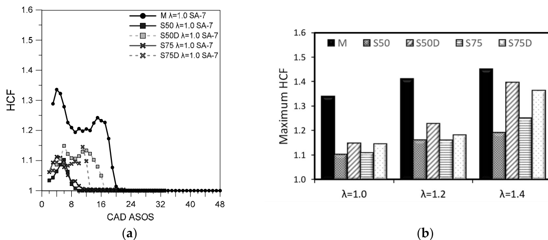
Figure 19. (a) Average Heywood Circularity Factor trend at stoichiometric air-fuel ratio ( \lambda = 1.0 ) and (b) Maximum Heywood Circularity Factor for all air-fuel ratios.
