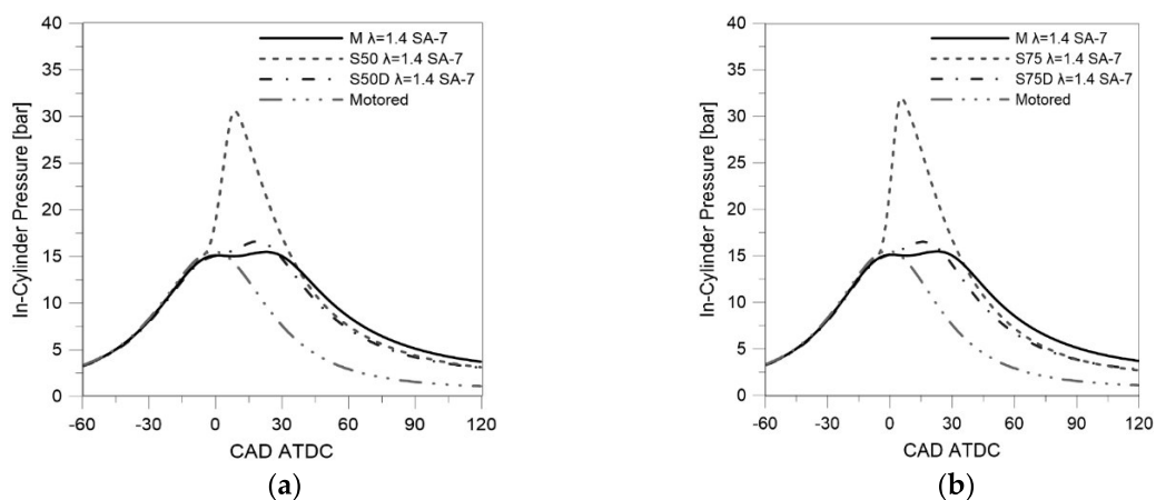
Figure 6. In-cylinder pressure traces averaged for lean fuelling ( \lambda = 1.4 ) for: (a) 50% H_2 blends and (b) 75% H_2 blends, compared with methane.
