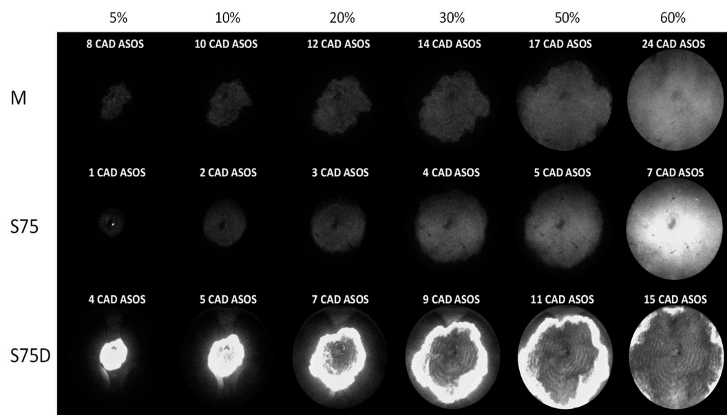
Figure 11. Image sequence of flame evolution at the same flame area (5%, 10%, 20%, 30%, 50% and 60% of the piston cross-section) for a stoichiometric air-fuel ratio ( \lambda = 1.0 ) with M, S75, and S75D fuelling.
