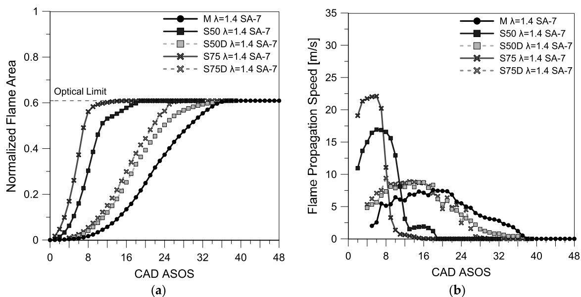
Figure 16. Average flame front evolution in terms of normalized area (cross-section piston area) and flame propagation speed for the leanest air-fuel ratio and five different fuels.
