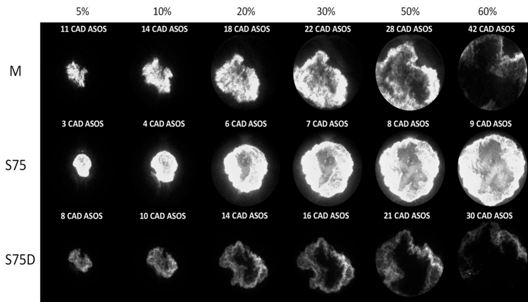
Figure 13. Image sequence of flame evolution at the same flame area (5%, 10%, 20%, 30%, 50% and 60% of the piston area) for a lean air-fuel ratio ( \lambda = 1.4 ) with M, S75, and S75D fueling.
