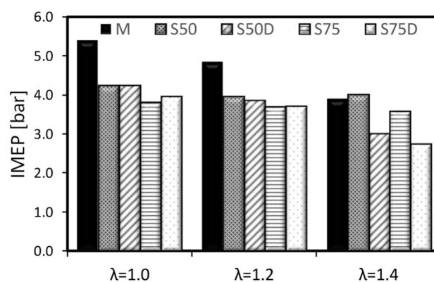
Figure 7. Indicated mean effective pressure for M, S50, S50D, and S75D at fixed SA ( -7 CAD ATDC) and air-fuel dilution from 1.0 to 1.4.
