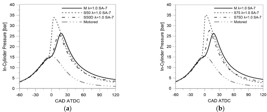
Figure 5. In-cylinder pressure traces averaged for stoichiometric fuelling ( \lambda = 1.0 ) for: (a) 50% H_2 blends and (b) 75% H_2 blends, compared with methane.
