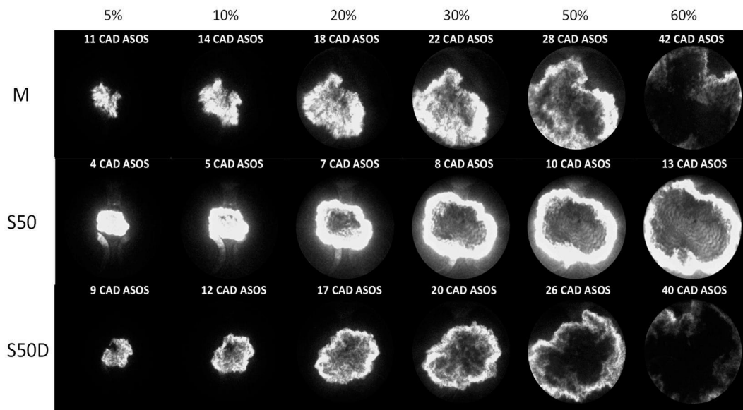
Figure 12. Image sequence of flame evolution at the same flame area (5%, 10%, 20%, 30%, 50% and 60% of the piston area) for a lean air-fuel ratio ( \lambda = 1.4 ) with M, S50, and S50D fueling.
