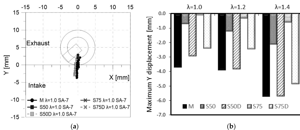
Figure 20. (a) Average evolution of flame centroid with respect to the combustion chamber center at a stoichiometric air-fuel ratio ( \lambda = 1.0 ) and (b) maximum centroid displacement in the vertical direction for all air-fuel ratios.
