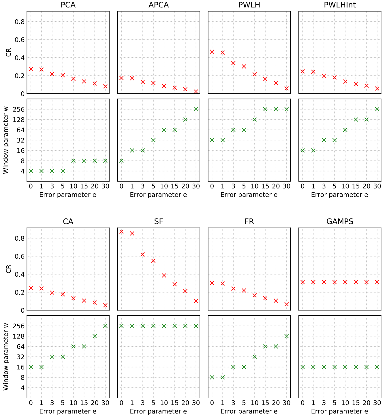
FIGURE C.8: CR and window size parameter plots for every evaluated algorithm, for the data type "Longitude" of the dataset ElNino.
