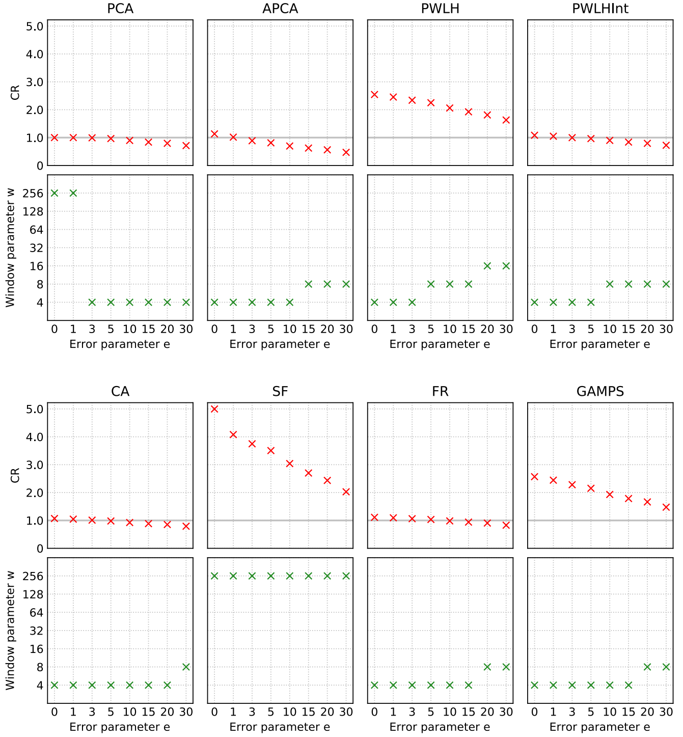
FIGURE C.19: CR and window size parameter plots for every evaluated algorithm, for the data type "Latitude" of the dataset Wind.
