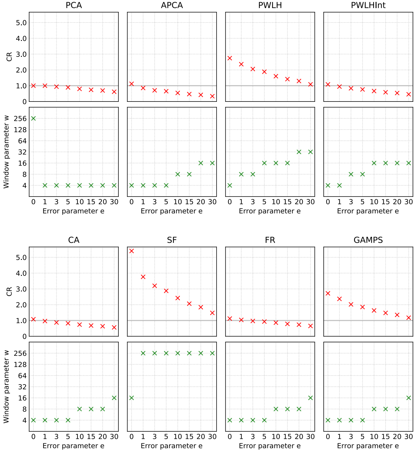
FIGURE C.17: CR and window size parameter plots for every evaluated algorithm, for the data type “Latitude” of the dataset Tornado.
