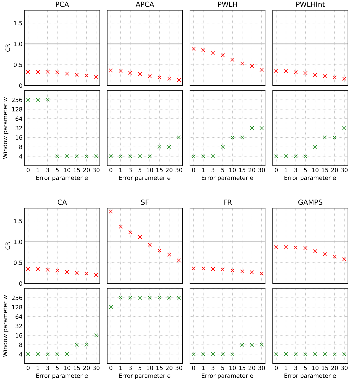
FIGURE C.12: CR and window size parameter plots for every evaluated algorithm, for the data type "Air Temp." of the dataset ElNino.
