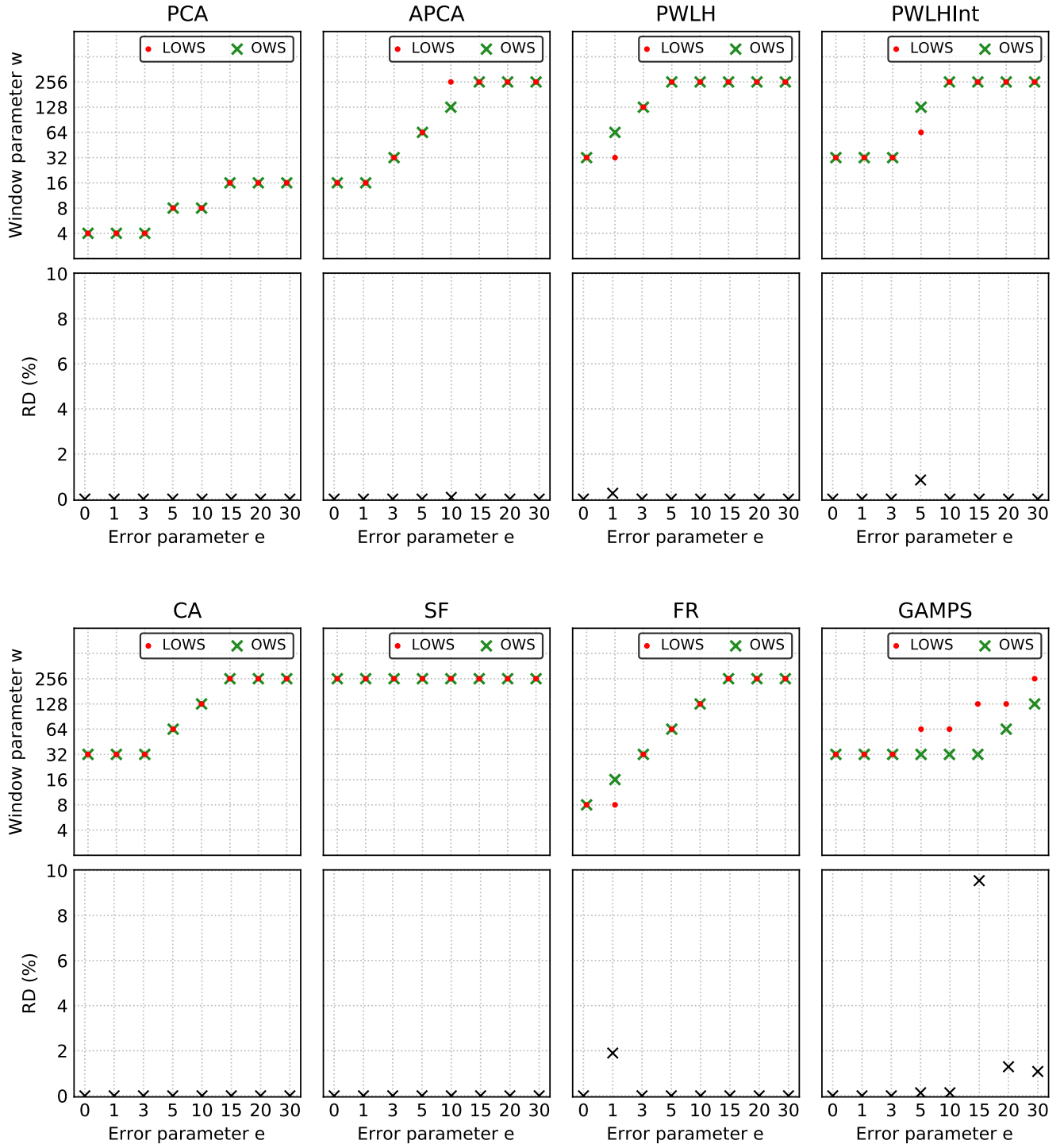
FIGURE B.7: Plots of w_{global}^* , w_{local}^* , and the RD between c_{<a_v, w_{global}^*, e>} and c_{<a_v, w_{local}^*, e>} , as a function of the error parameter e , obtained for the data type “VWC” of the file “irkis-SLF2.csv” of the dataset IRKIS.
