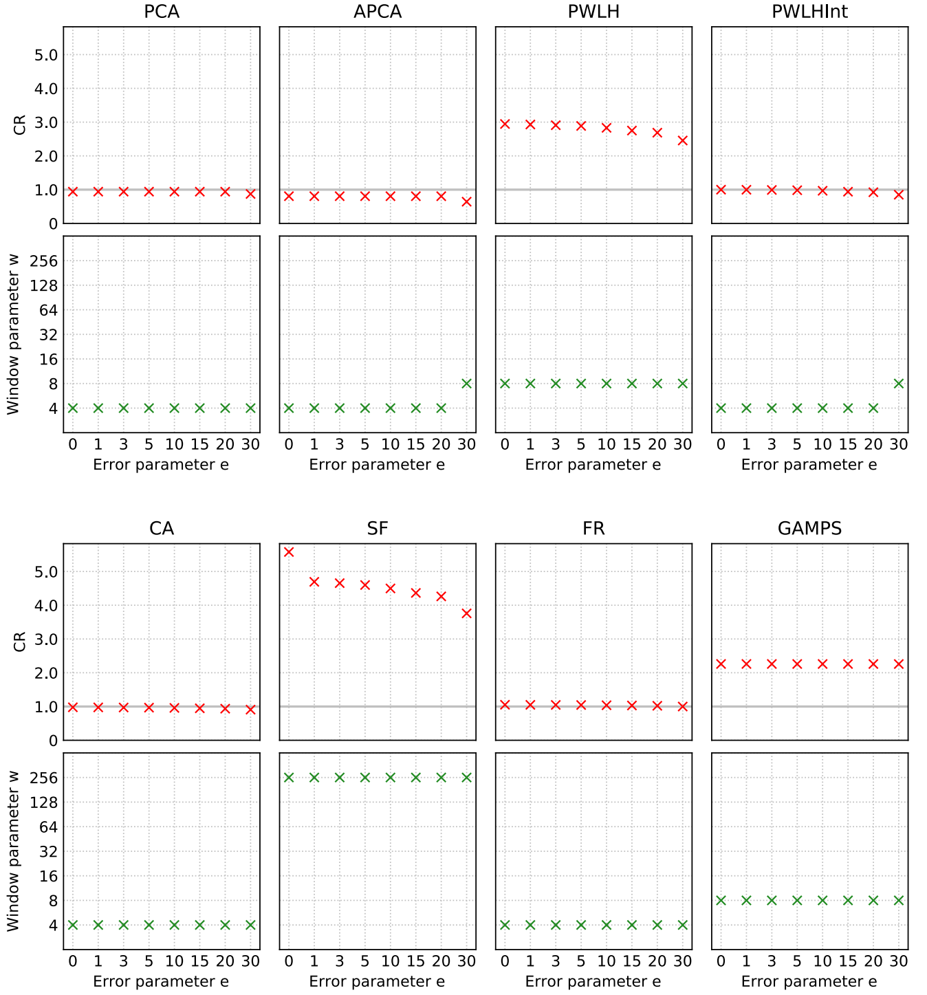
FIGURE C.16: CR and window size parameter plots for every evaluated algorithm, for the data type “Size” of the dataset Hail.
