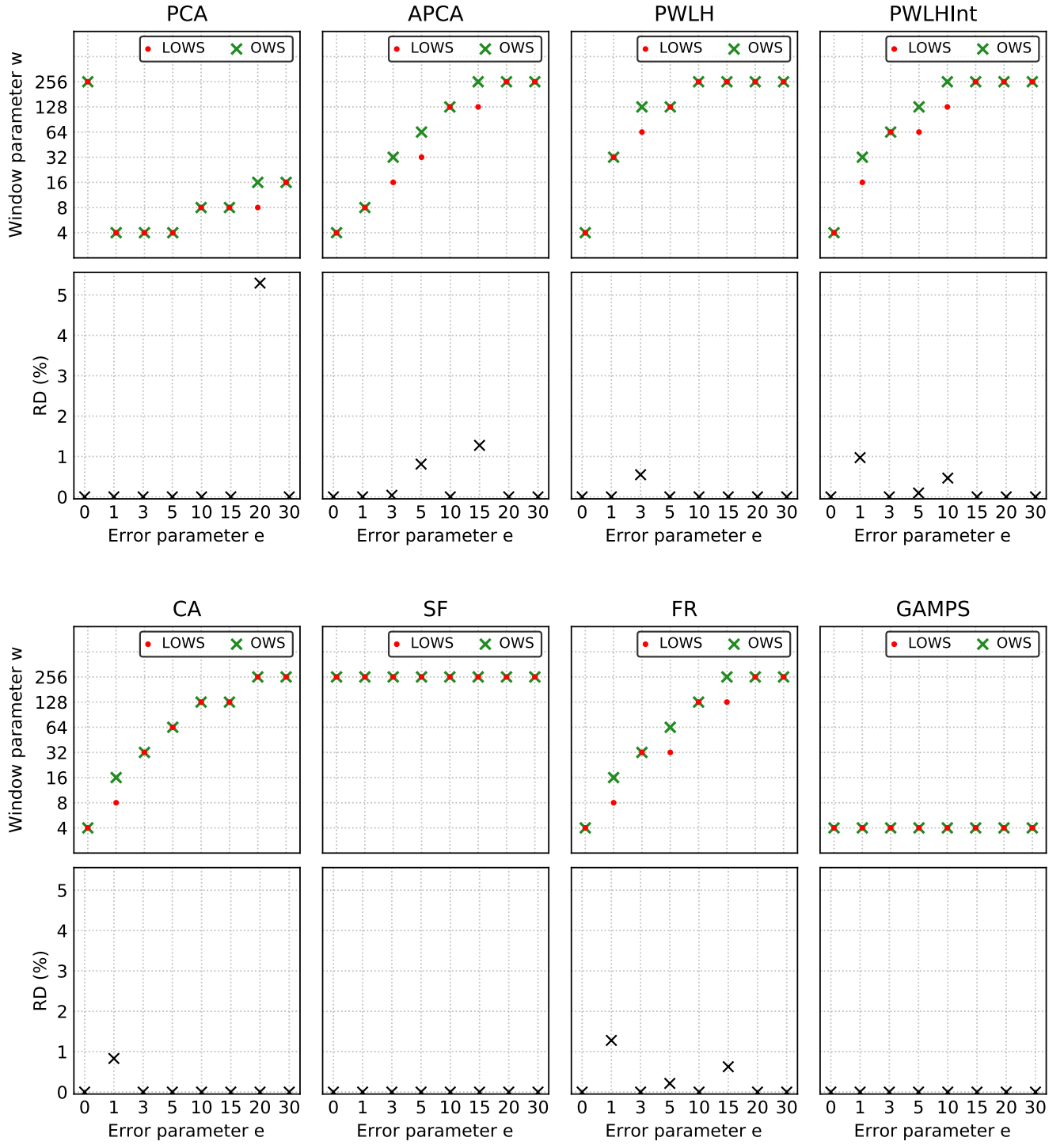
FIGURE B.10: Plots of w_{global}^* , w_{local}^* , and the RD between c_{<a_v, w_{global}^*, e>} and c_{<a_v, w_{local}^*, e>} , as a function of the error parameter e , obtained for the data type “SST” of the file “sst-03-2017.csv” of the dataset SST.
