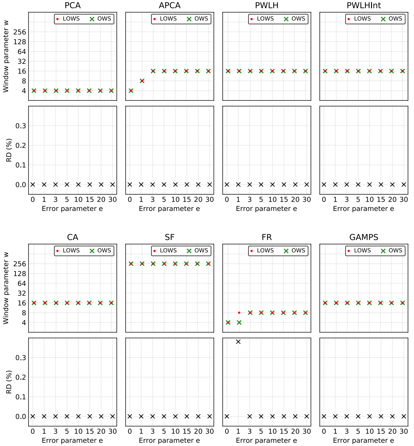
FIGURE B.14: Plots of w_{global}^* , w_{local}^* , and the RD between c_{<a_v, w_{global}^*, e>} and c_{<a_v, w_{local}^*, e>} , as a function of the error parameter e , obtained for the data type “GHI” of the file “solar-2011.csv” of the dataset Solar.
