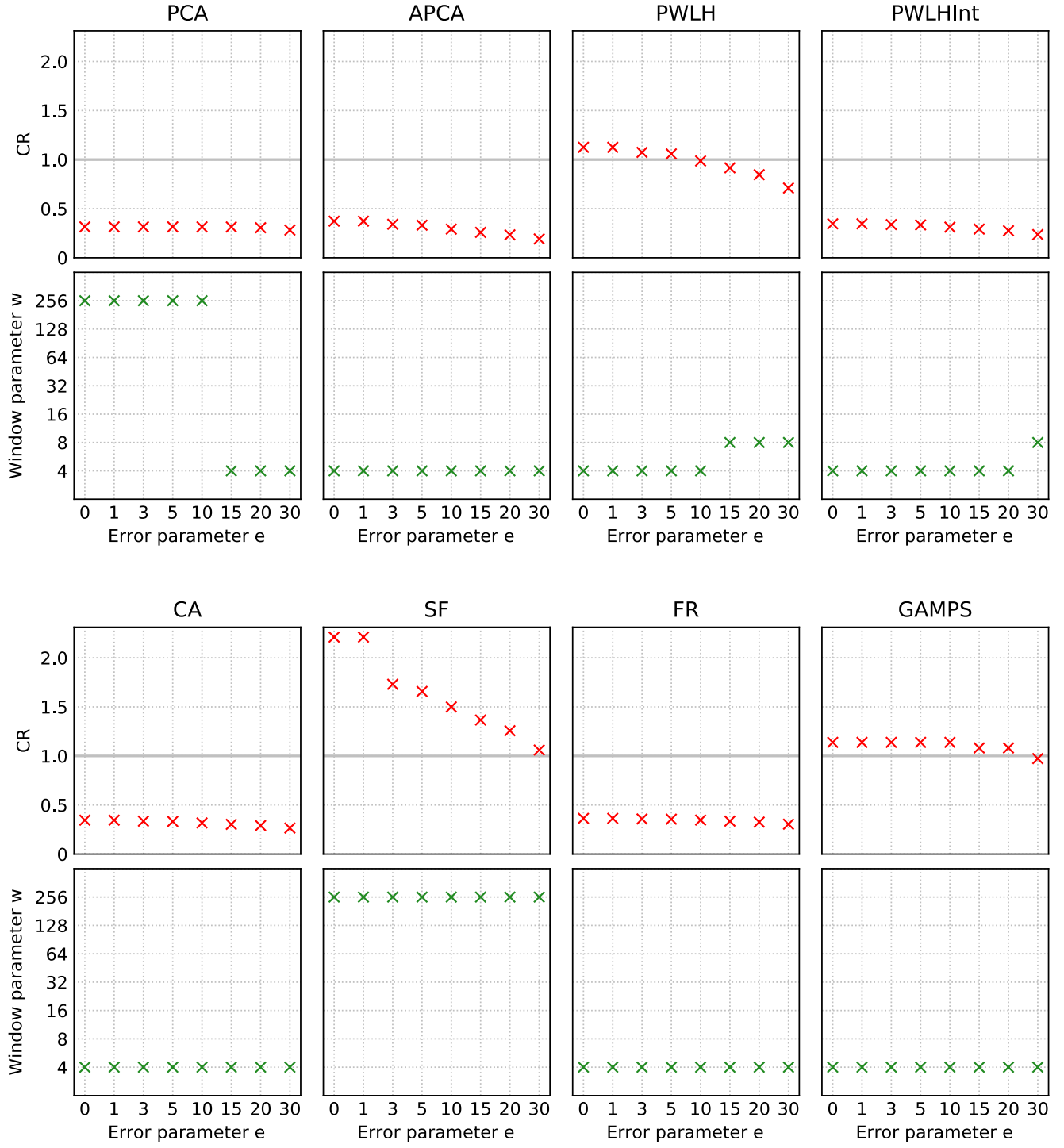
FIGURE C.10: CR and window size parameter plots for every evaluated algorithm, for the data type "Mer. Wind" of the dataset ElNino.
