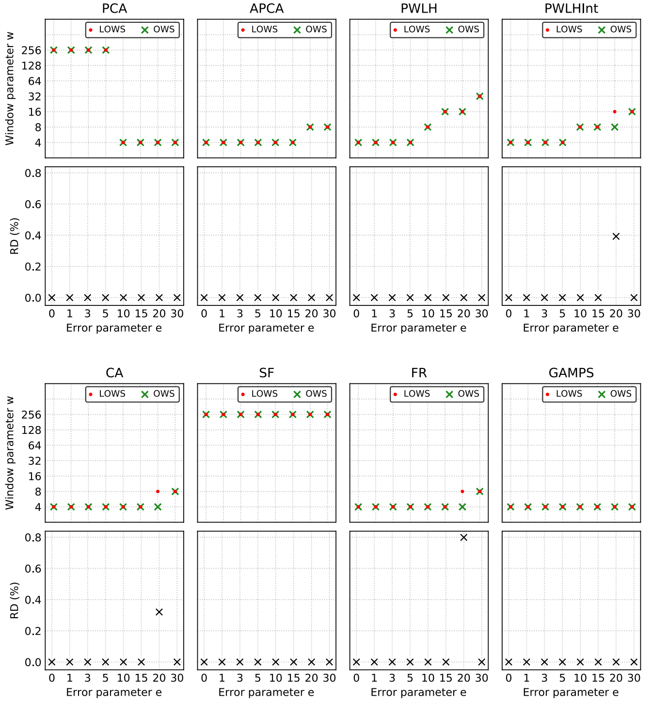
FIGURE B.13: Plots of w_{global}^* , w_{local}^* , and the RD between c_{<a_v, w_{global}^*, e>} and c_{<a_v, w_{local}^*, e>} , as a function of the error parameter e , obtained for the data type “Velocity” of the file “adcp-03-2015.csv” of the dataset SST.
