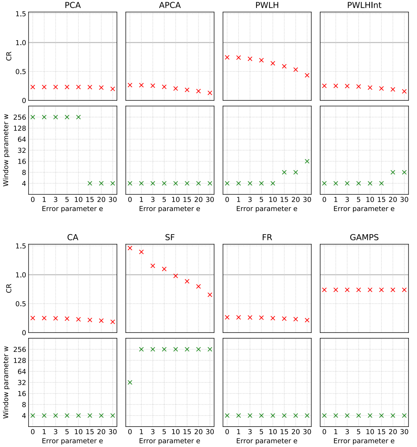
FIGURE C.11: CR and window size parameter plots for every evaluated algorithm, for the data type "Humidity" of the dataset ElNino.
