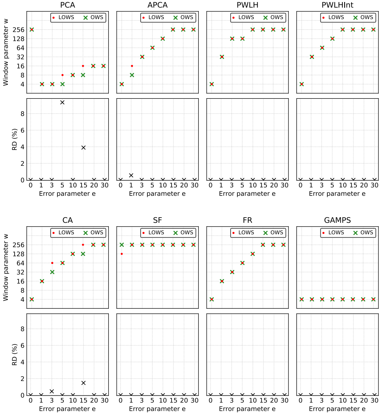
FIGURE B.8: Plots of w_{global}^* , w_{local}^* , and the RD between c_{<a_v, w_{global}^*, e>} and c_{<a_v, w_{local}^*, e>} , as a function of the error parameter e , obtained for the data type “SST” of the file “sst-01-2017.csv” of the dataset SST.
