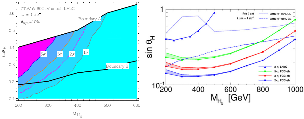
Figure 114. Left: discovery contour with respect to \sin \theta_H and M(H_5^{+ + / - -}) at the LHeC using an unpolarized beam. Reprinted figure with permission from [627], Copyright 2017 by the American Physical Society. Right: limit contours for the case of singly charged Higgs for the FCC-eh and the LHeC. The blue dotted curve and the blue dashed curves give the 95% CL limit from CMS for H_5^{+ / -} and for H^{+ + / - -} , respectively. Reproduced from [628]. CC BY 4.0. An unpolarized beam with an integrated luminosity of 1 \text{ ab}^{-1} and a 10% systematic uncertainty for background yields are assumed in both plots.
