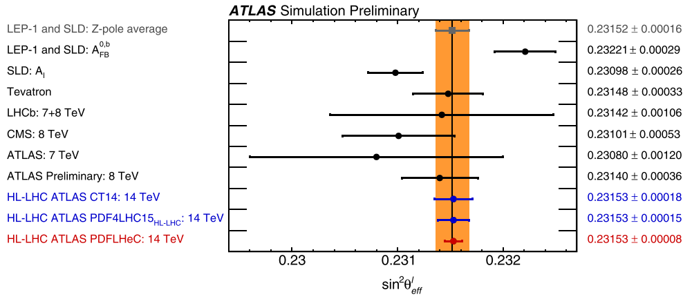
Figure 130. Comparison of measurements or combinations of \sin^2 \theta_{\text{eff}}^{\ell} with the world average value (orange band) and the projected uncertainties of measurements at the HL-LHC. Reproduced from [716]. CC BY 4.0. For the HL-LHC, the central values are set to the world average value, and uncertainties are displayed for different assumptions of the available PDF sets, similarly to table 20.
