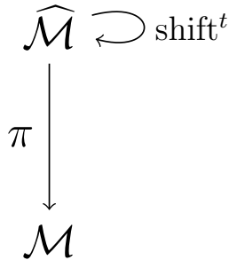
Figure 3.1: The main objects of this section.
