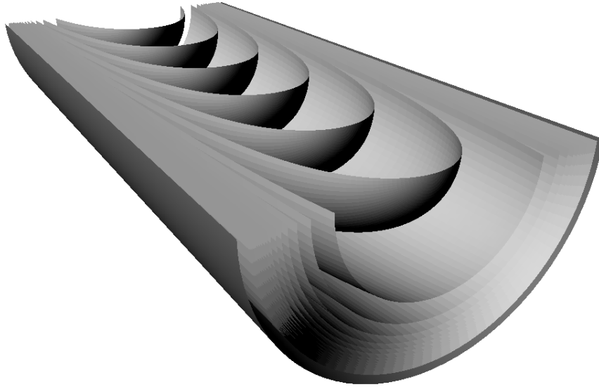
Figure 4.2: A section of the Reeb cylinder.
