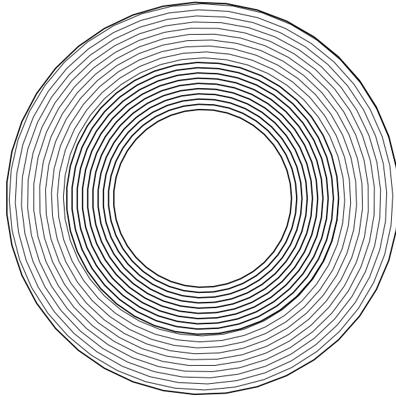
Figure 4.4: A broken record foliation. Circular leaves with trivial holonomy accumulate on a circular leaf with non-trivial holonomy.
