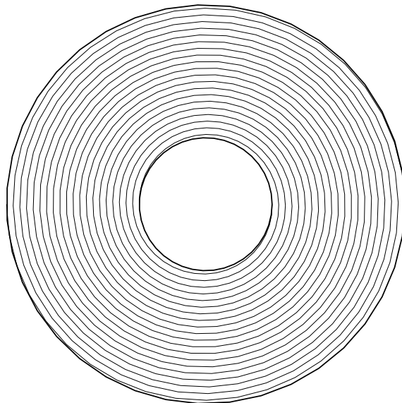
Figure 4.1: The vinyl record foliation.
