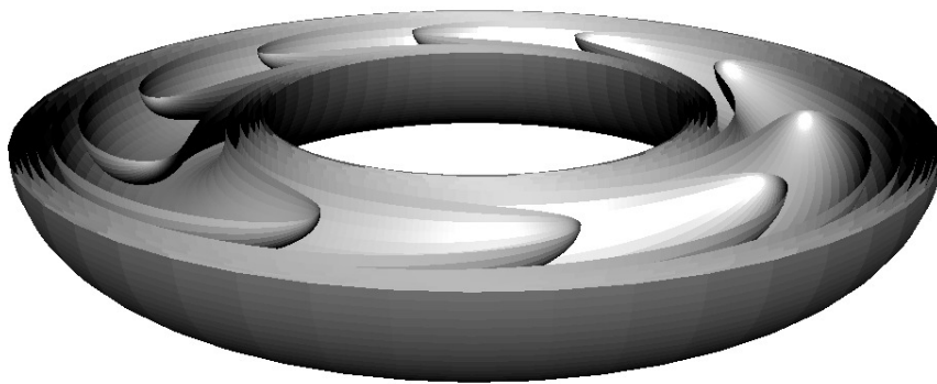
Figure 4.3: Half a Reeb component.
