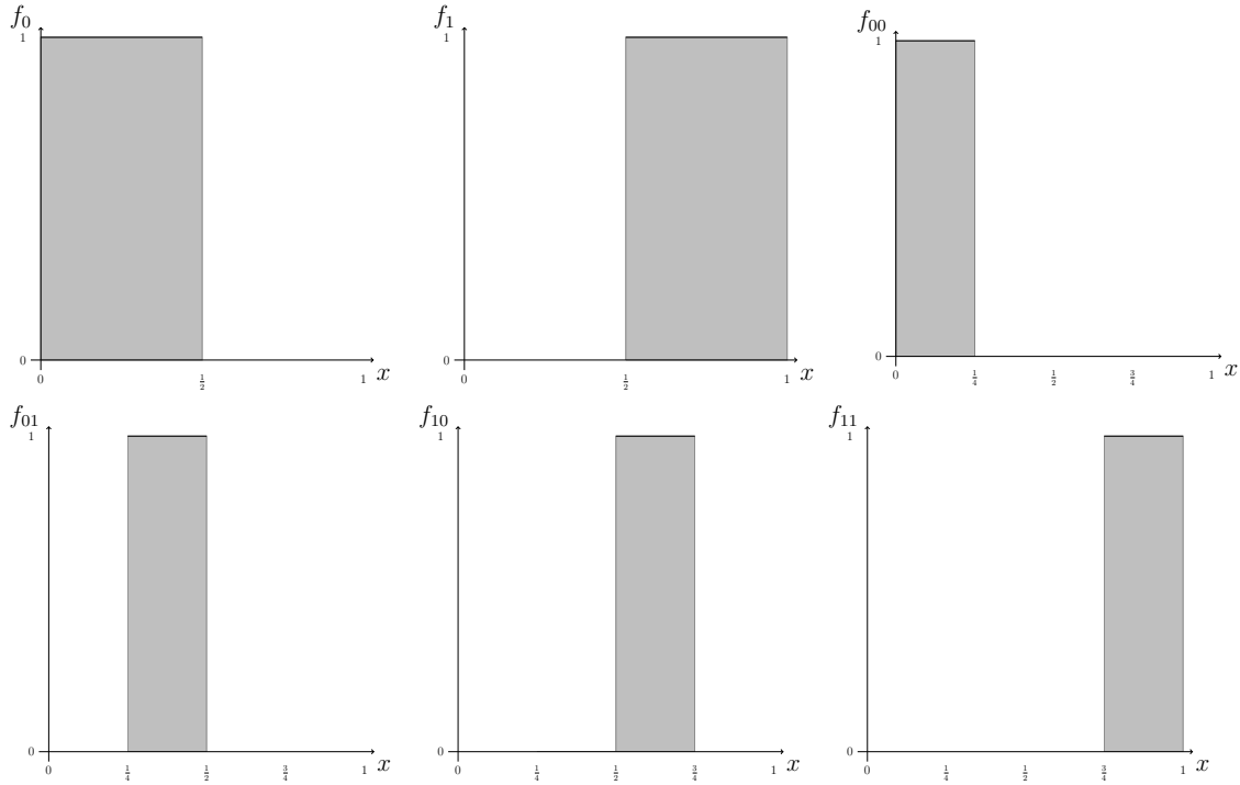
Figure 4.6: Six elements of a sequence of functions which does not converge almost surely to 0 but has no other limit points.
