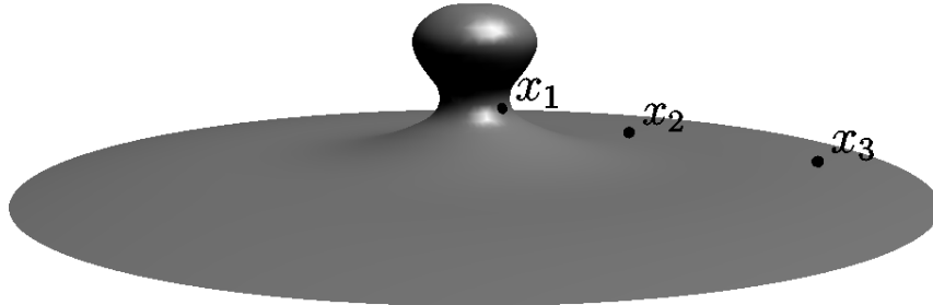
Figure 4.7: An asymptotically flat surface with finite injectivity radius. Changing the basepoint gives an sequence converging to a limit whose injectivity radius is infinite.
