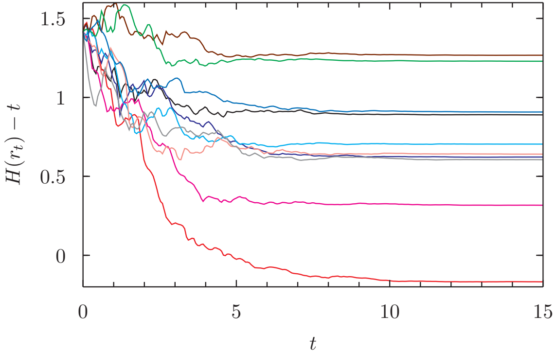
Figure 1.1: Ten trajectories of the process H(r_t) - t .
