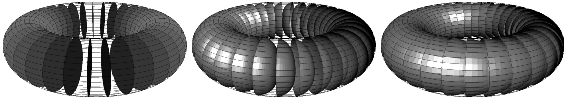
Figure 4.5: A Reeb transition: the trivial partition of a solid torus into disks is deformed into a Reeb component.
