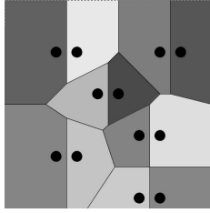
Figure 1: Voronoi diagram.
