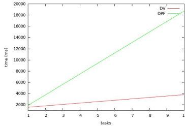
Figure 8: Multiple tasks execution time.
