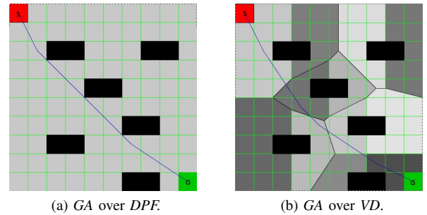
Figure 7: Visual comparison.
