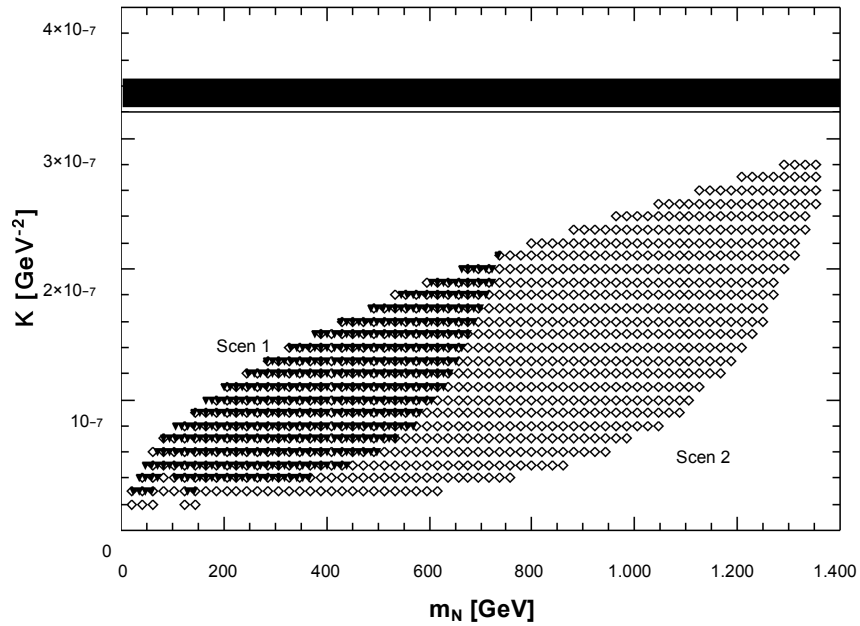
FIG. 6: Majorana neutrino discovery regions at 5 . The horizontal line represents the low-energy and LEP limits discussed in Sec. IIIB.
