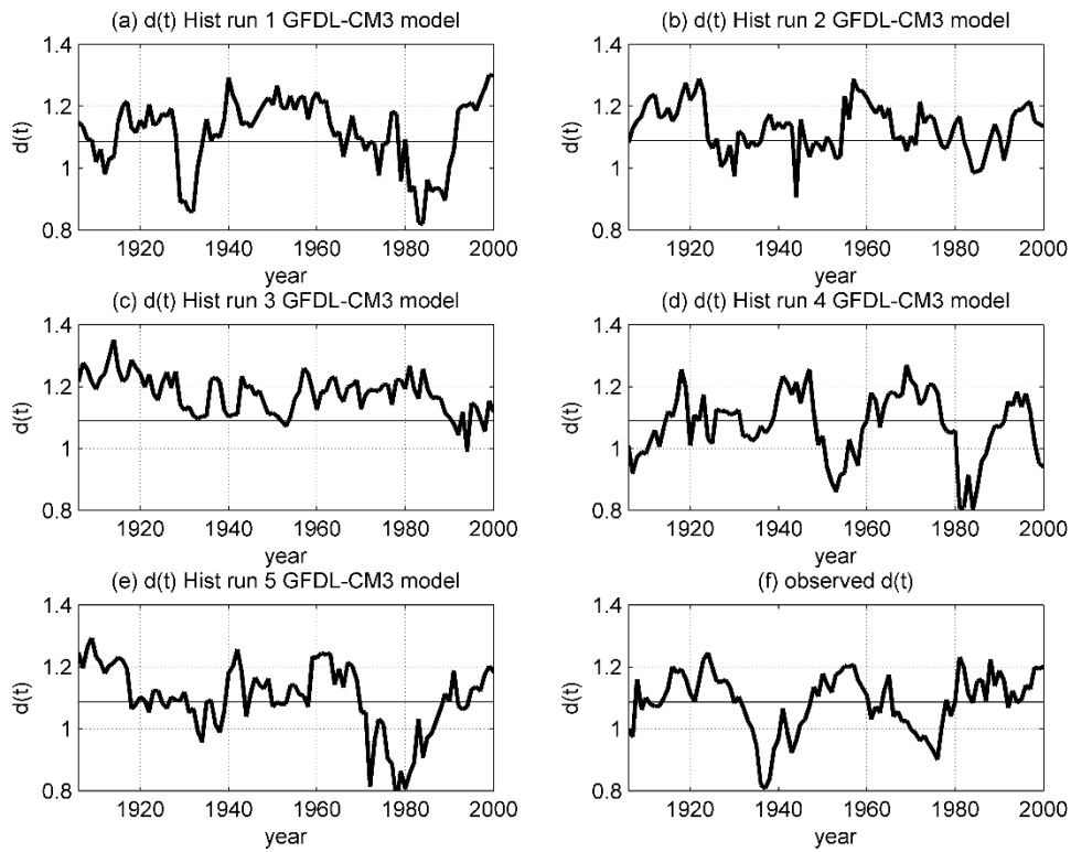
Figure 5.1 Mean network distance time series during the 20 th century computed considering the first (a), second (b), third (c), forth (d) and fifth (e) historical run form GFDL-CM3 model, and the 20 th century observations (SST from ERSSTv3b and PCP from GPCCv5) on figure (f). Mean network distance computed following Martín-Gómez and Barreiro, 2015. The horizontal black line represents the threshold level.
