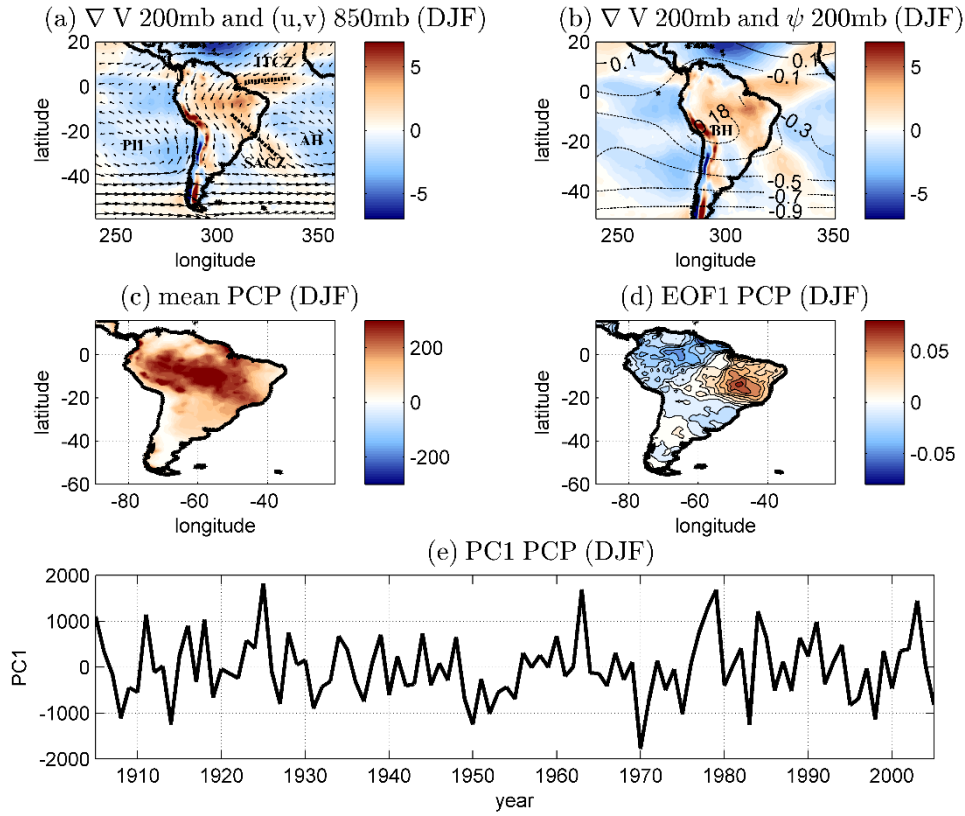
Figure 2.2. Mean values of (a) horizontal wind divergence at 200mb in 10^{-6} \text{ s}^{-1} (shaded regions) and horizontal wind pattern at 850mb in \text{m} \cdot \text{s}^{-1} (vectors); (b) horizontal wind divergence at 200mb in 10^{-6} \text{ s}^{-1} (shaded regions) and streamfunction at 200mb (contours), (c) mean PCP over SA, (d) the EOF1 component of PCP over DJF and (e) its associated PC1.
