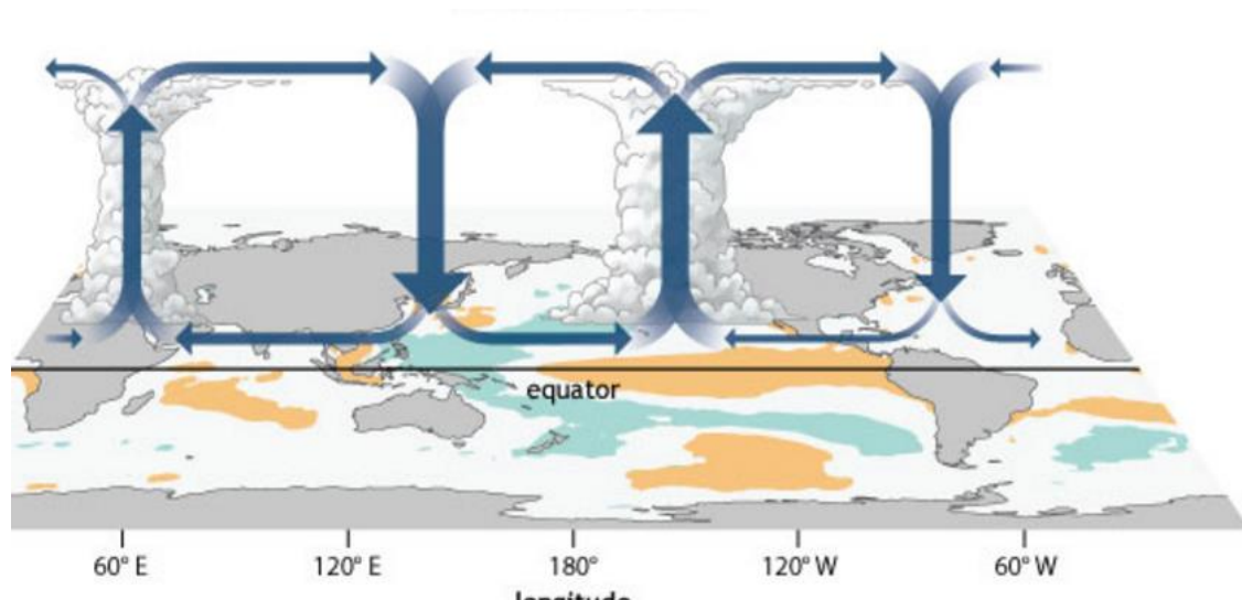
Figure 3.6. Pacific Walker circulation during DJF ENSO conditions. Figure taken from NOAA Climate.gov: https://www.climate.gov/news-features/blogs/enso/walker-circulation-ensos-atmospheric-buddy . For the case of the negative phase of ENSO, the anomalous Walker circulation would be the opposite.
